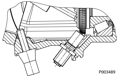
Cartridge housing
