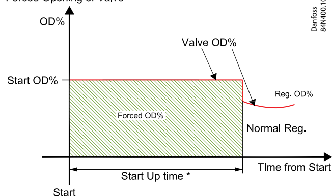
Forced Opening of Valve
