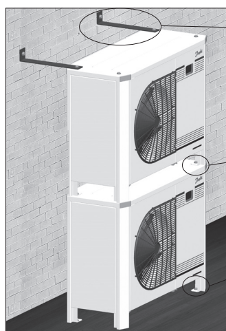
Picture 2 : Stacked mounting
