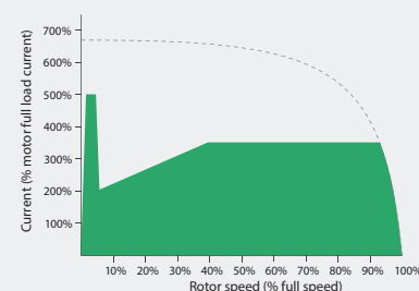
Constant current/ current ramp – shown here with kickstart
