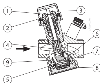
AB-QM DN 15-32
