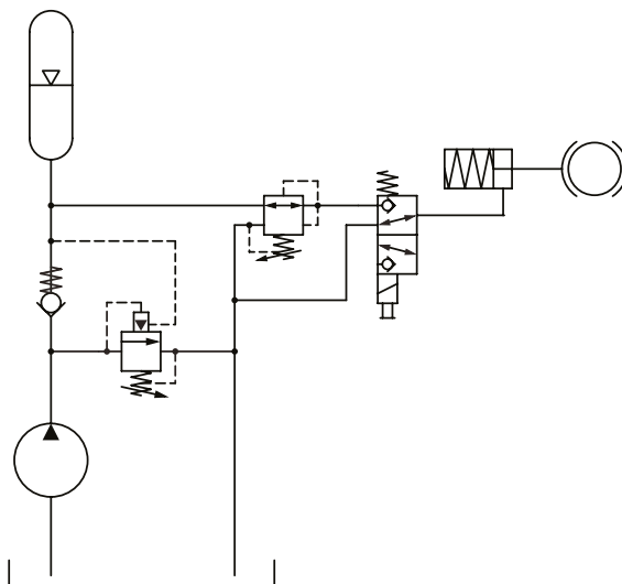
▲ Brake Circuit
