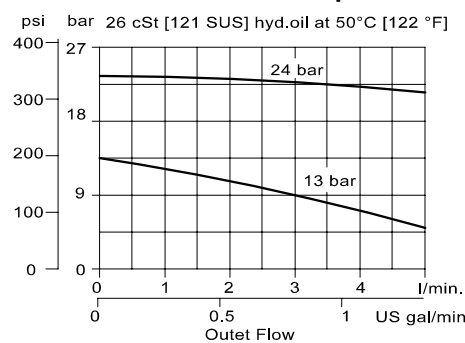
Reduced Pressure from ports 2-1
