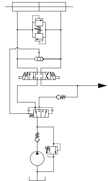
▲ Steering Circuit
