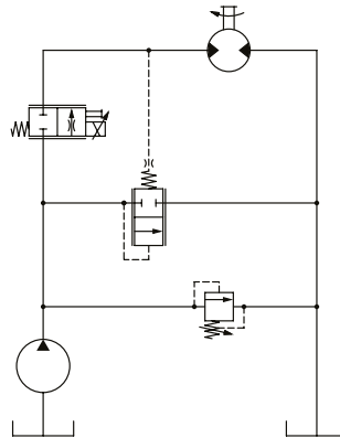
▲ Proportional Bypass Flow Control
