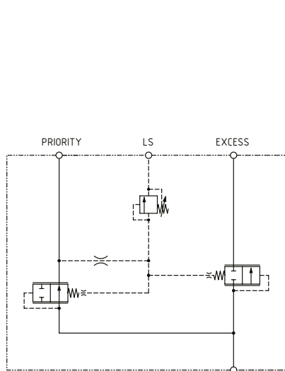
▲ Dynamic Priority Valve with Relief
