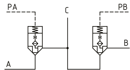
▲ Poppet Type
