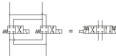
▲ 4-Way, 3-Position
