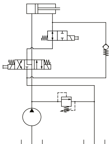
▲ Regenerative Circuit
