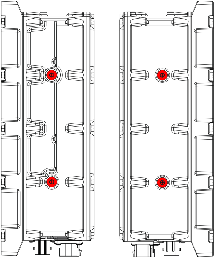
Lifting points
