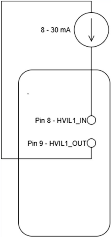
HVIL1 loop connection in the signal connector
