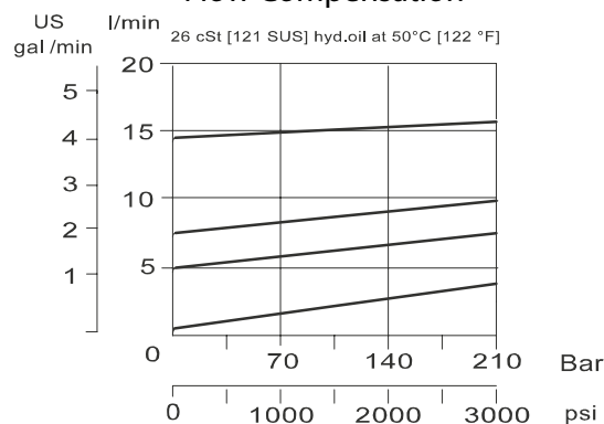
Flow Compensation
