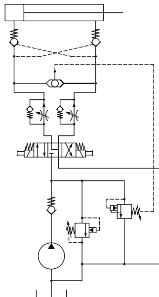
▲ Speed control
