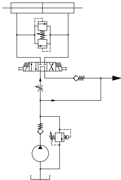
▲ Priority flow
