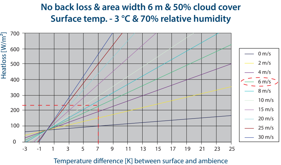
Fig. 1. Wind and temperature dependent heat loss
