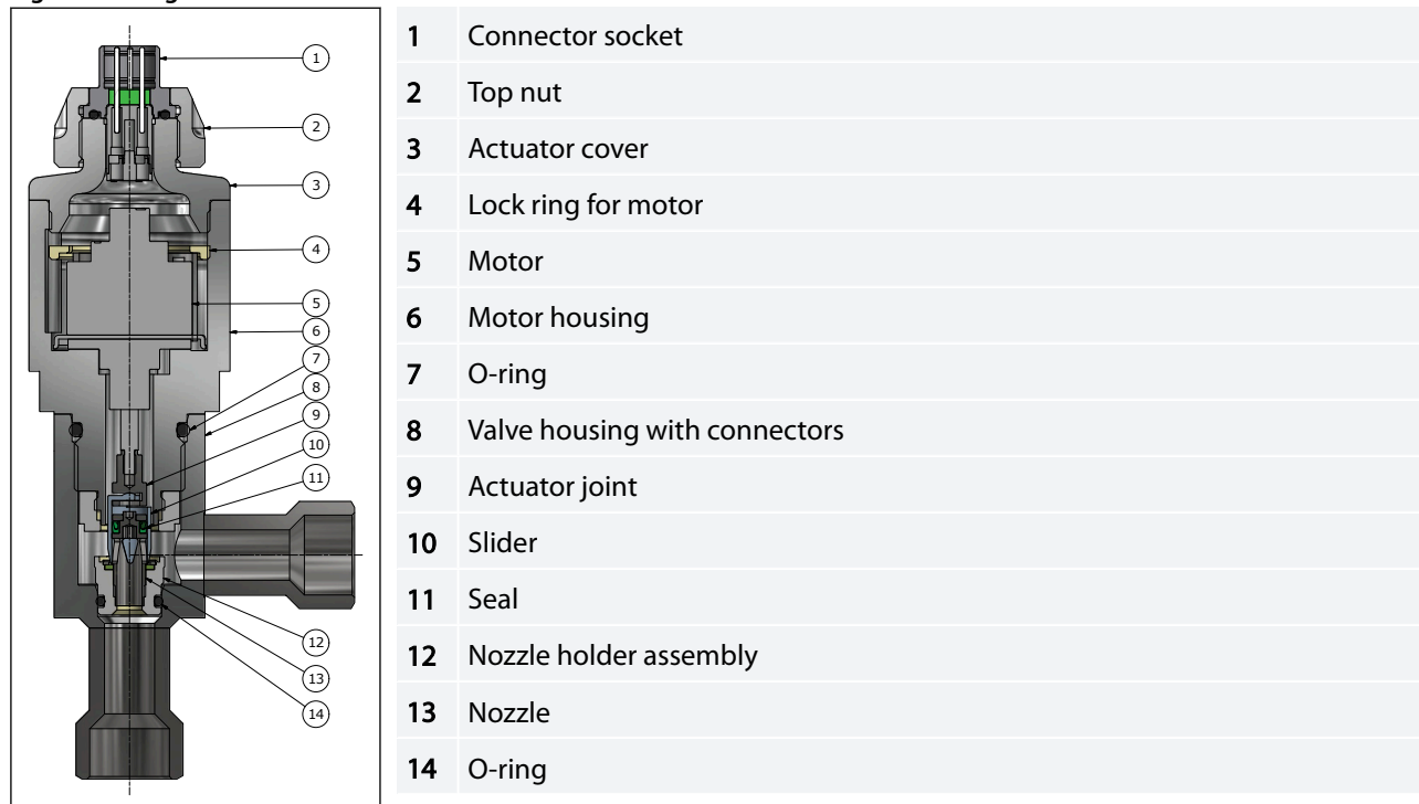
Figure 2: Design
