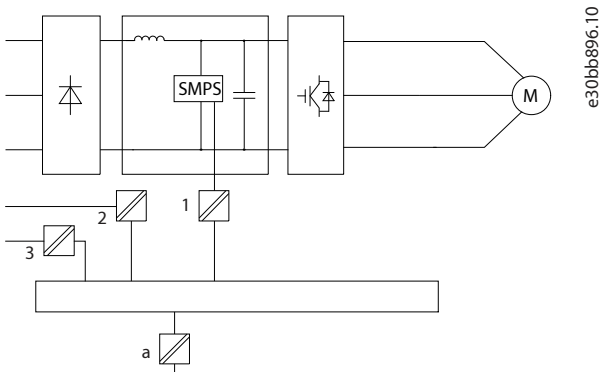
图 24: 电气隔离 0.37-22 kW (0.5-30 hp)
