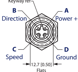
4 pin Turck Eurofast connector
