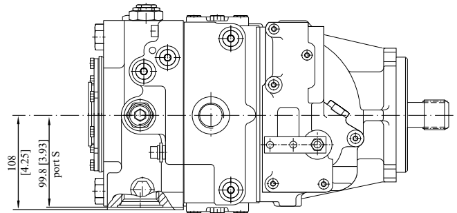
View "Y"
