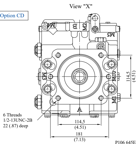
View "X"
