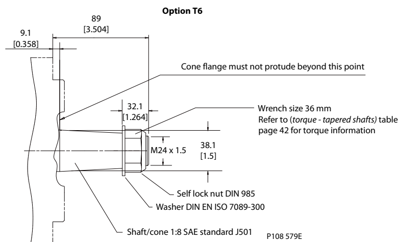
Shaft dimensions
