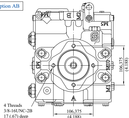
View "X"
