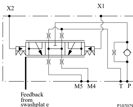
Hydraulic displacement control schematic
