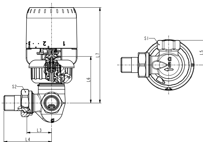
RA-DV DN : Bypass left & right / Danfoss Aero and Aveo® sensor
