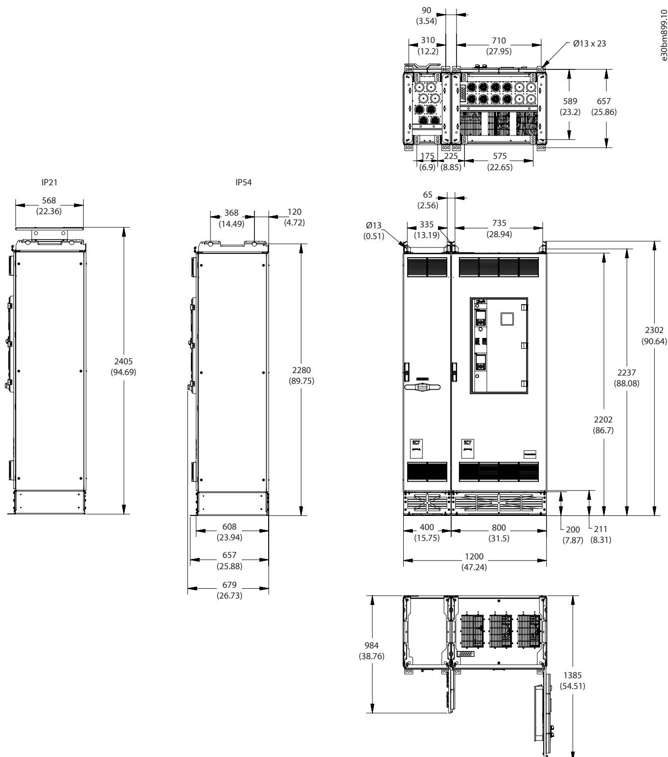
Figure 83: Dimensions for the Bottom Cabling Option, AE11, IE11, in mm (in)
