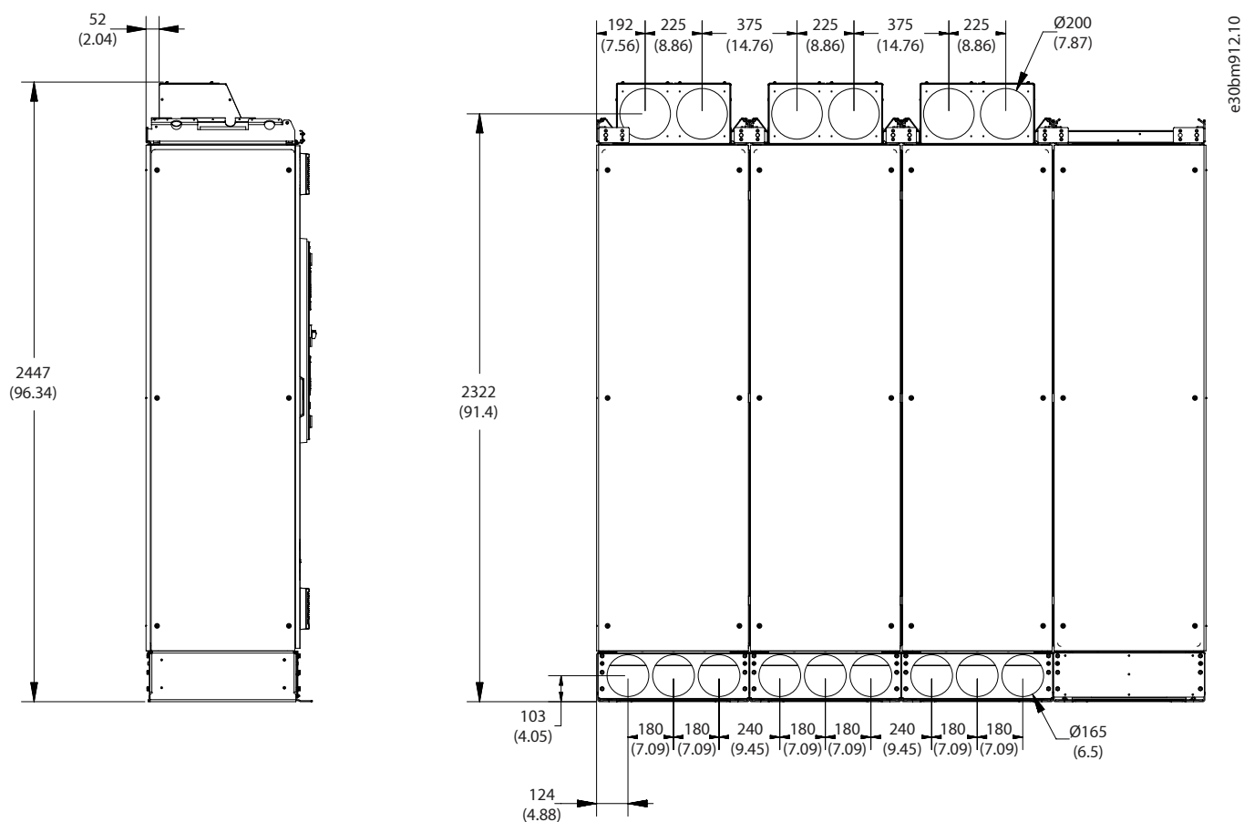
Figure 101: Dimensions for Back-channel Cooling (+OABC), 2 x AE11, 2 x IE11, in mm (in)
