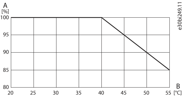
Figure 126: Output Current Derating vs. Ambient Temperature
