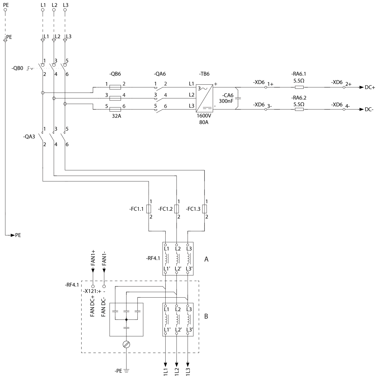
Figure 116: Wiring Diagram, AE10+IE10, 385–590 A
