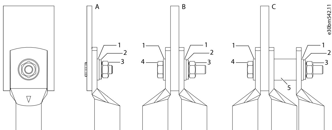
Figure 53: Connecting the Power Cables to the Terminals
