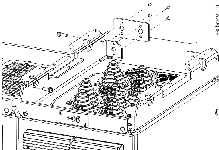
Figure 23: Lifting Bar Connection Plate
