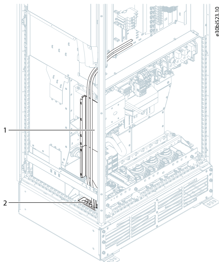
Figure 70: Routing of Control Cables from the Bottom, AE10/11, IE10/11
