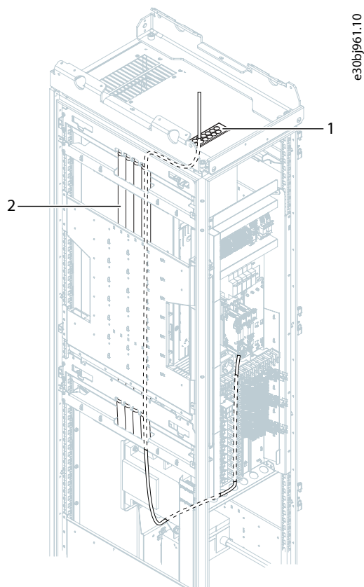
Figure 67: Routing of Control Cables from the Top, FE9, FE10
