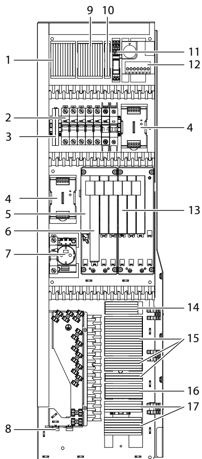
Figure 59: Elements inside the Control Compartment, FE9
