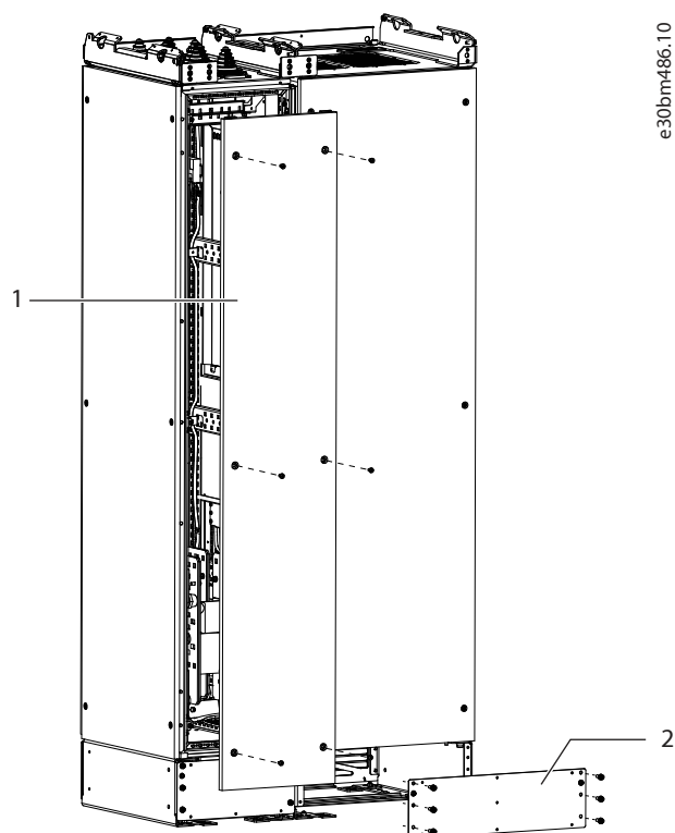
Figure 19: Removing the Back Wall and the Back Plate
