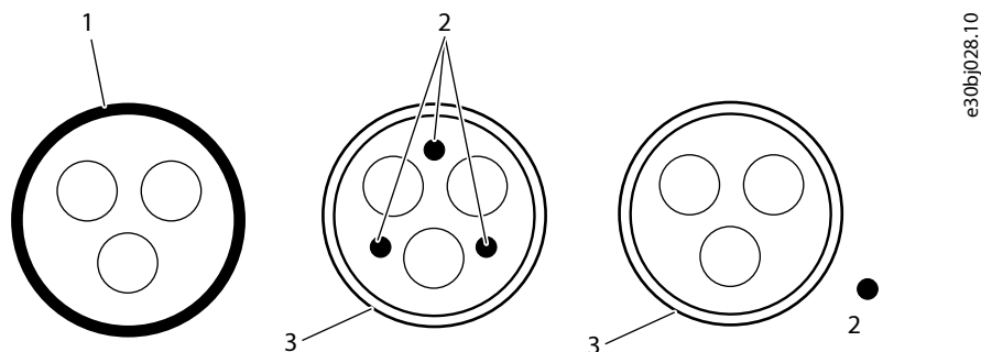
Figure 36: Recommended Cable Types for Mains and Motor Cabling
