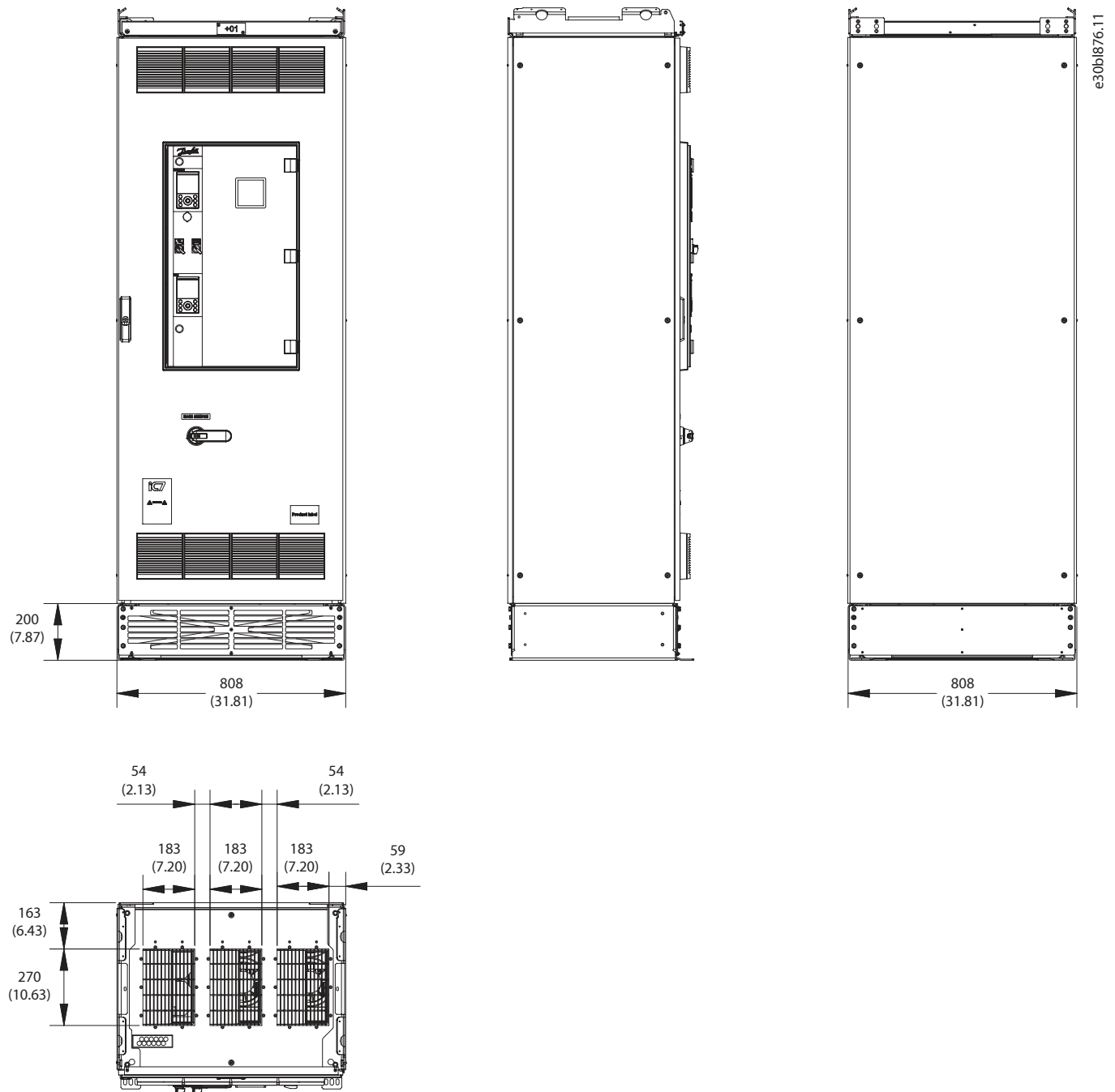
Figure 92: Dimensions for Default Cooling, AE10, IE10, in mm (in)
