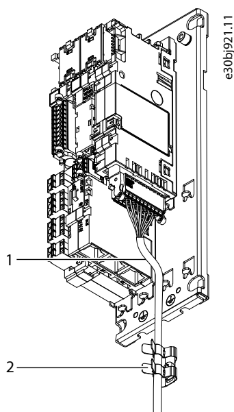
Figure 72: Example of Installing the Control Cables on the Option Board
