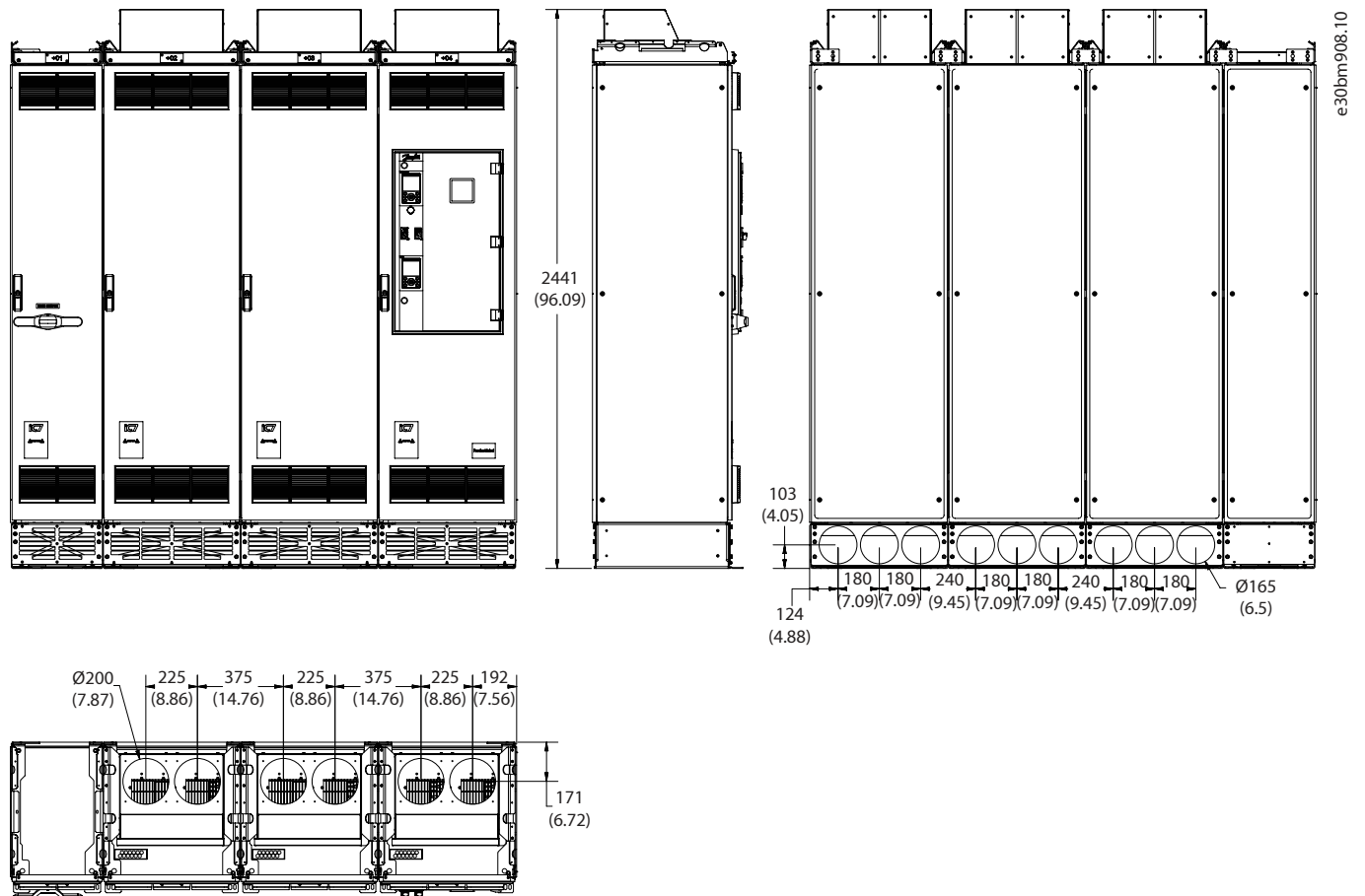
Figure 106: Dimensions for the Cooling Air Output Flange Option (+OAOF), 2 x AE10, 2 x IE10, in mm (in)
