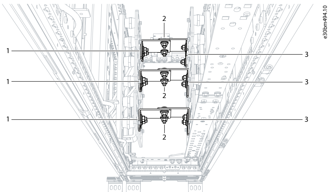
Figure 26: Busbar Connection
