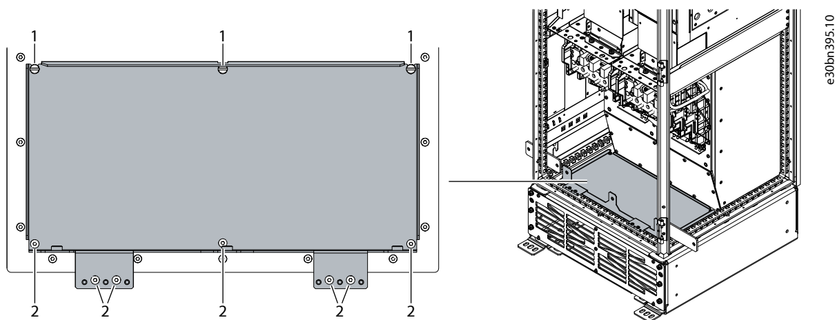
Figure 55: Removing the Gland Plate from the Bottom of the Inverter Cabinet
