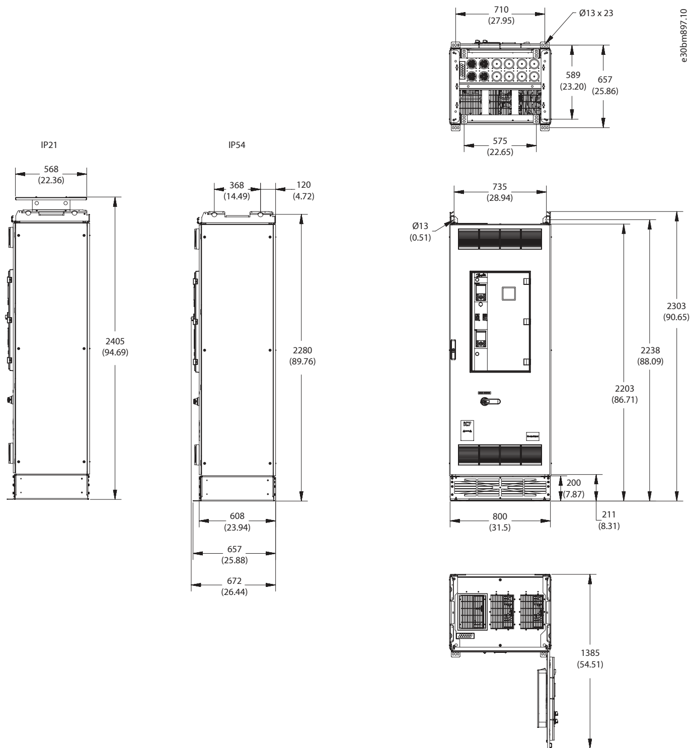
Figure 82: Dimensions for the Bottom Cabling Option, AE10, IE10, in mm (in)
