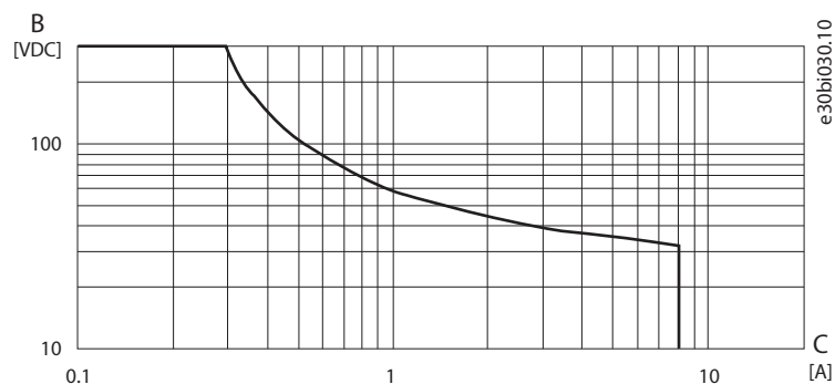
Figure 66: Maximum DC Load Breaking Capacity
