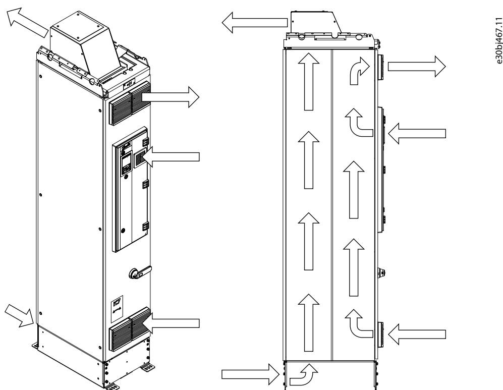
Figure 30: Back-channel Cooling (+OABC), Intake Back, Output Back
