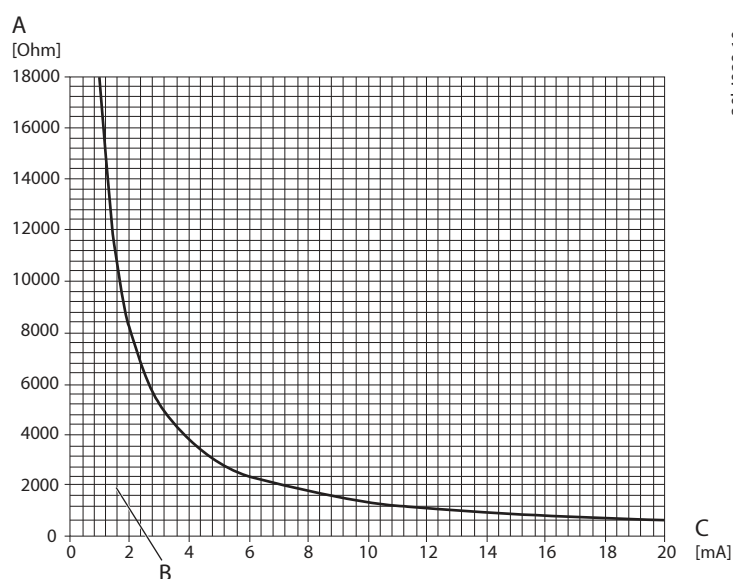
Figure 65: Allowed Load Resistance of Analog Output in Current Mode
