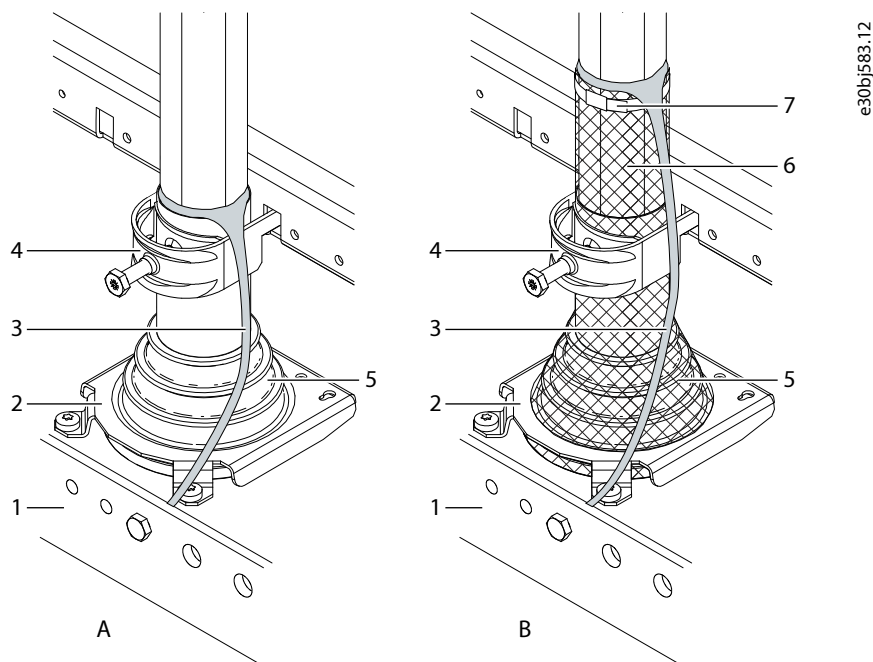
Figure 40: Cabling Methods (IEC)
