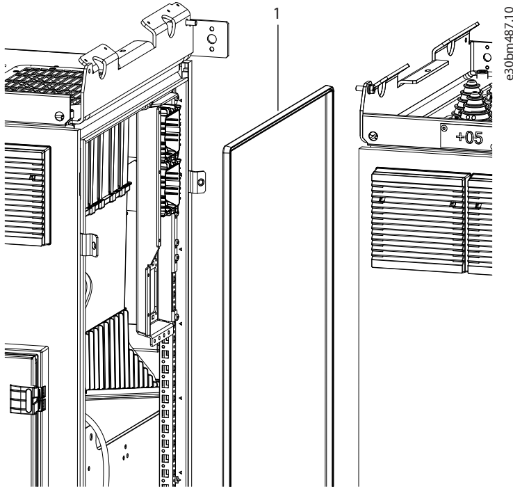
Figure 20: Installing the Seal to the Inverter Cabinet Section
