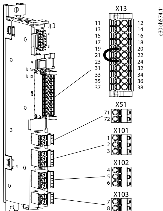
Figure 64: I/O and Relay Option Terminal Block and Terminal Numbering
