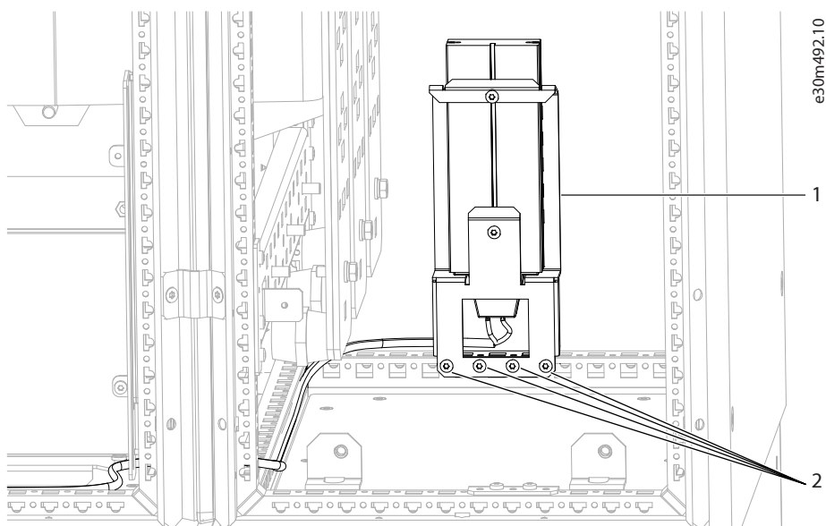
Figure 24: Installing the Cabinet Heater
