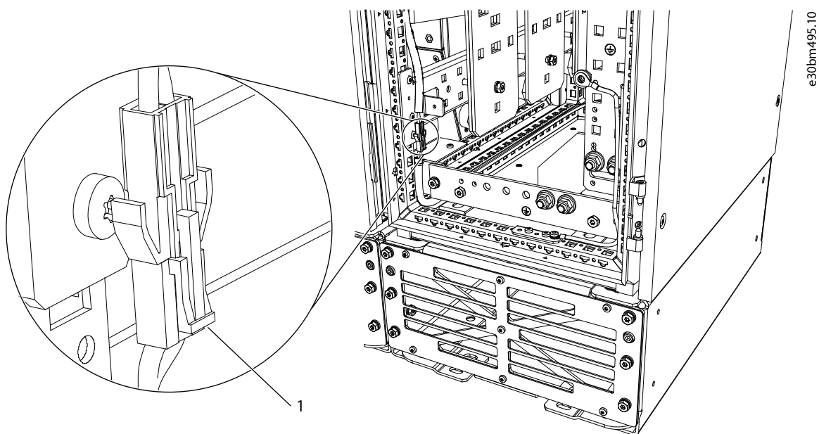
Figure 27: Wiring of the Top Fans
