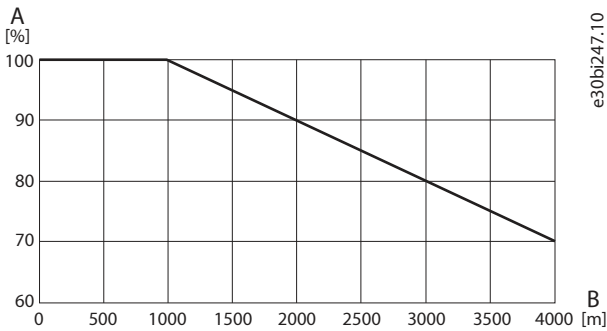
Figure 127: Output Current Derating vs. Installation Altitude
