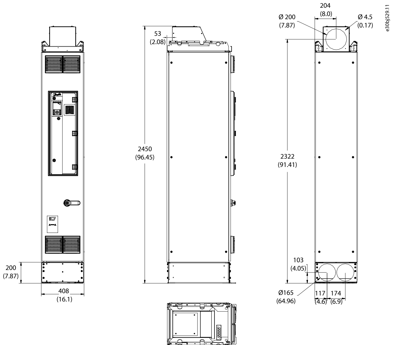
Figure 96: Dimensions for Back-channel Cooling (+OABC), FE9, in mm (in)
