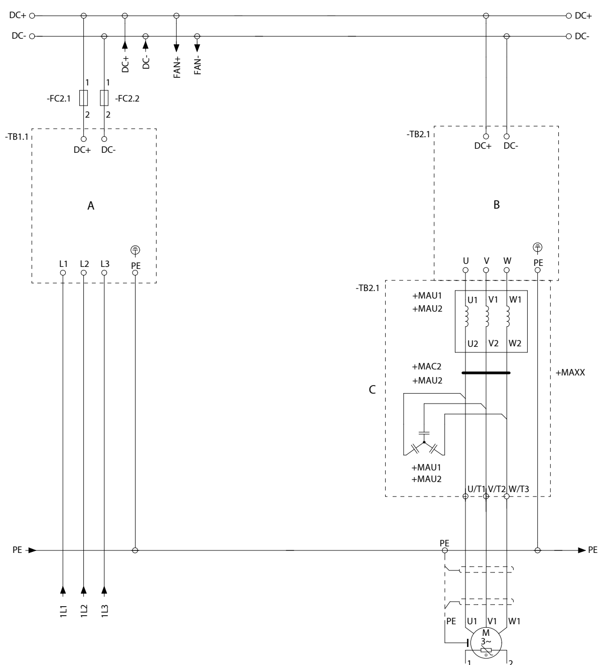
Figure 117: Wiring Diagram, AE10+IE10, 385-590 A (continued)
