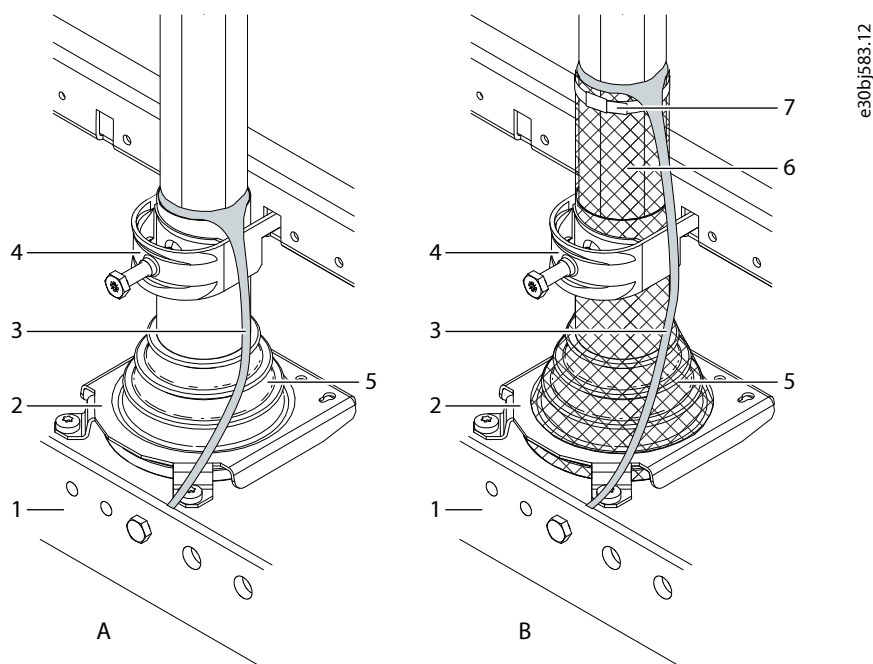
Figure 47: Cabling Methods (IEC)
