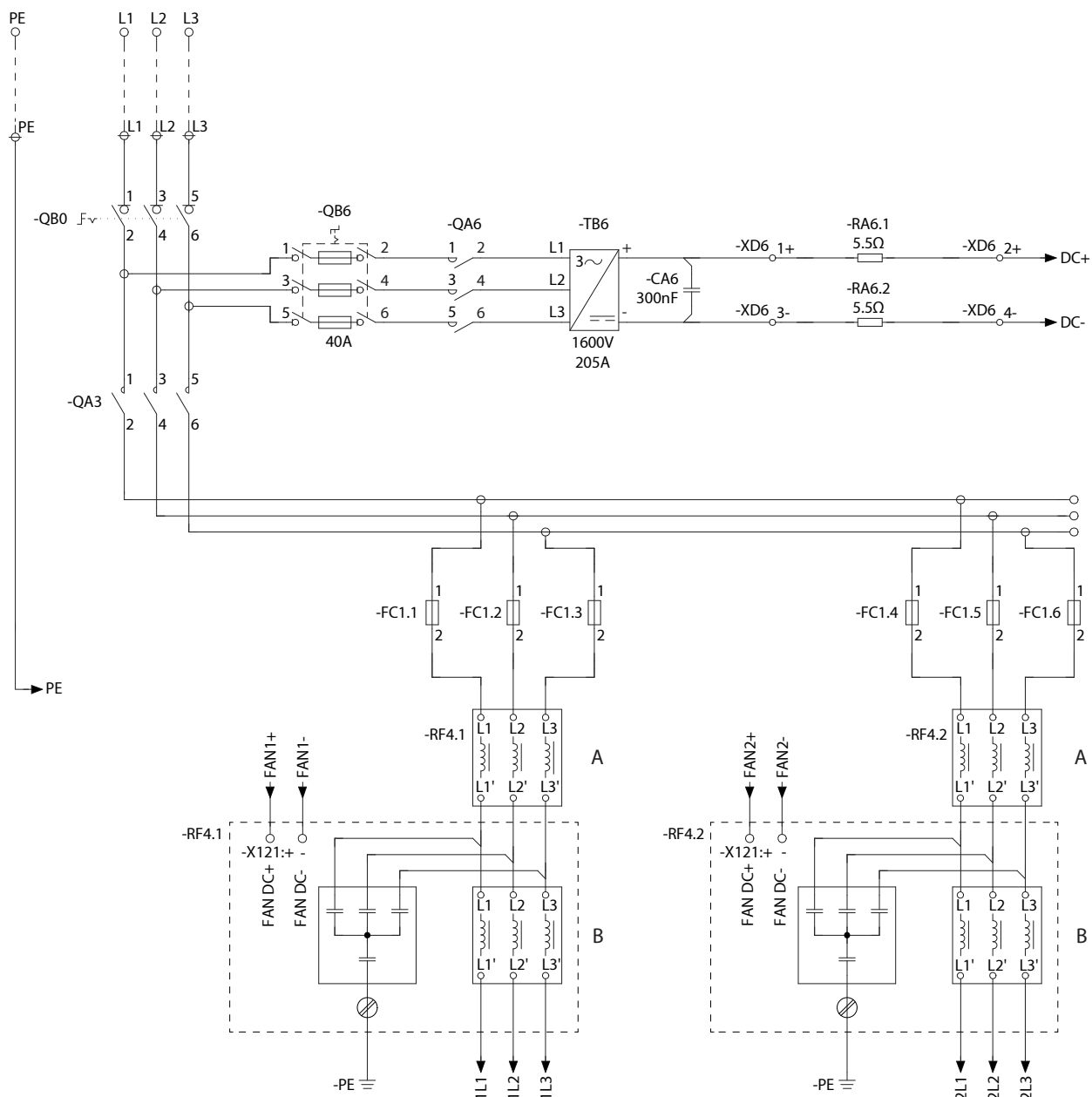
Figure 120: Wiring Diagram, 2 x AE10+2 x IE10, 1000–1100 A
