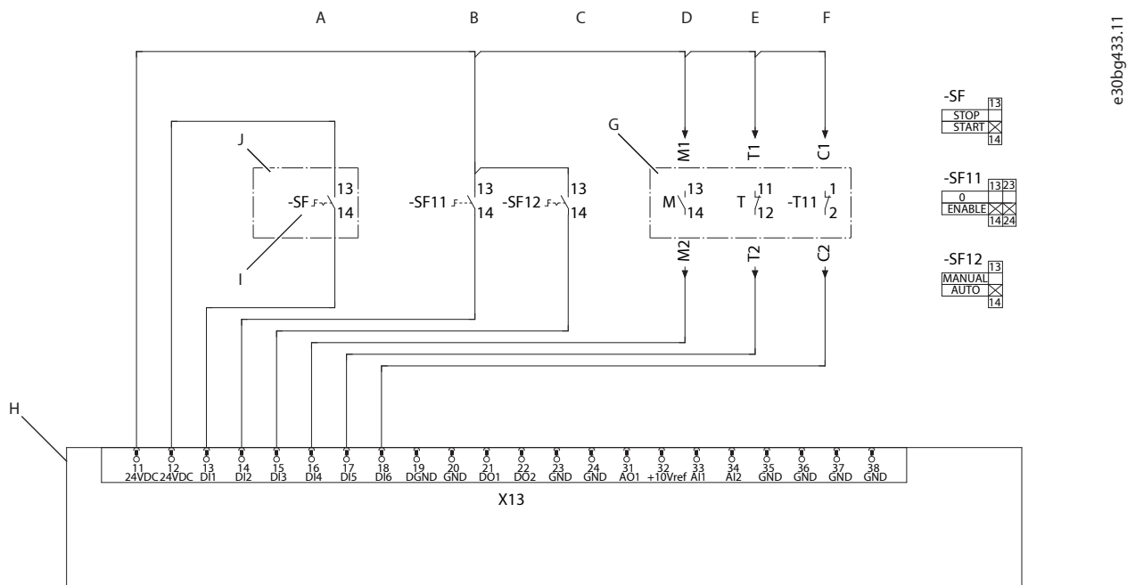
Figure 124: Pre-charging Control Wiring Diagram, AE10, AE11, IE10, IE11
