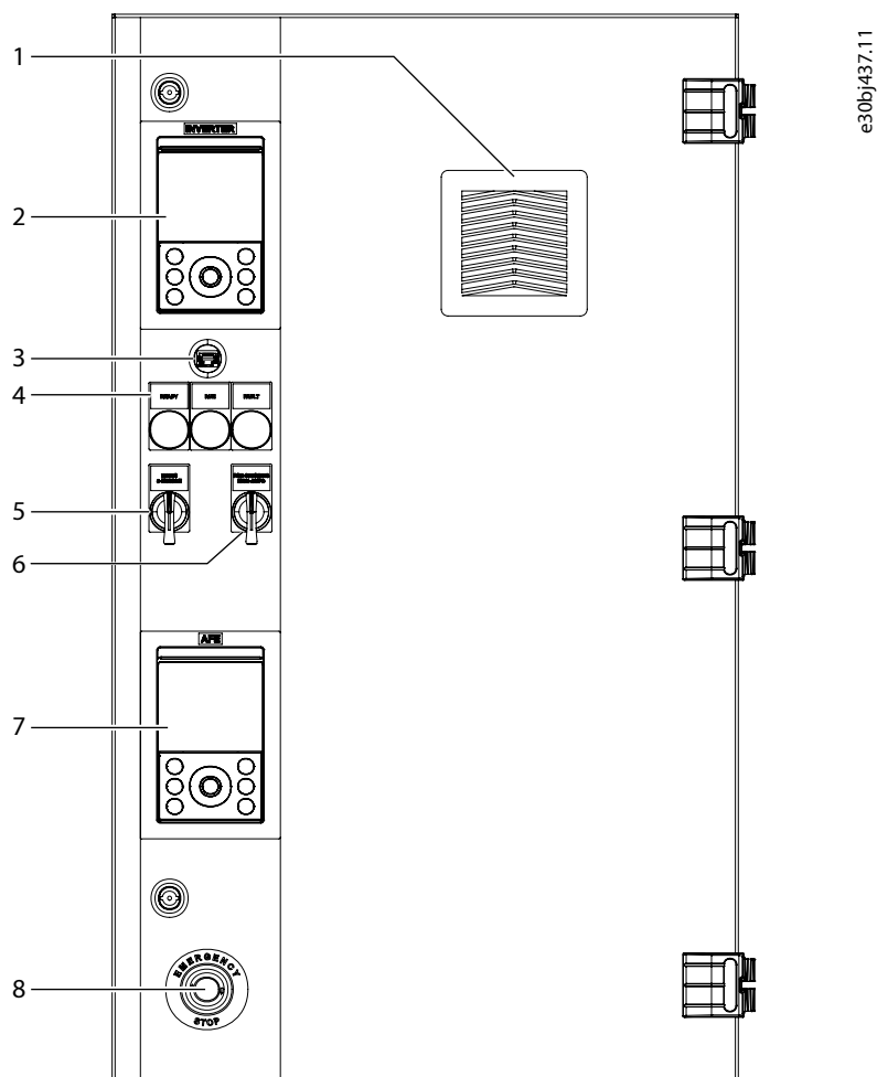
Figure 58: Control Compartment Door Elements, AE10/11, IE10/11
