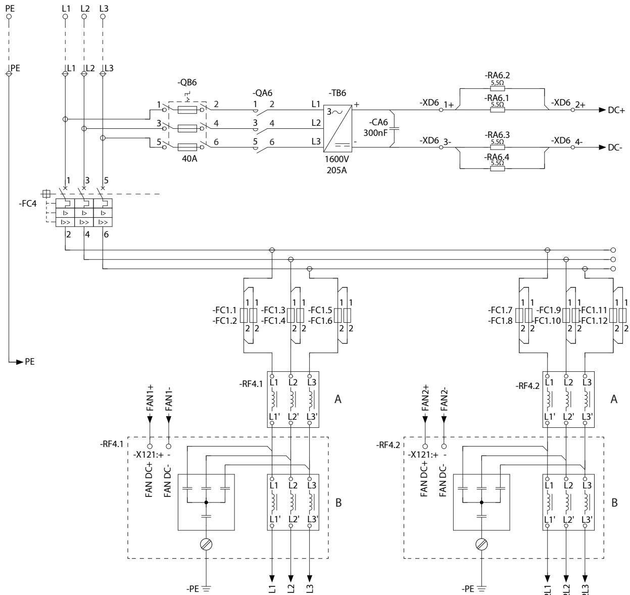
Figure 122: Wiring Diagram, 2 x AE11+2 x IE11, 1260–1710 A
