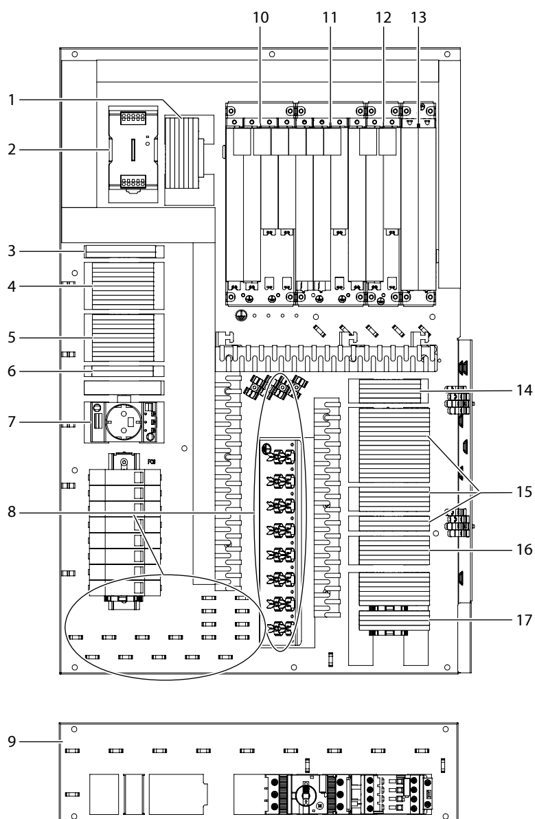
Figure 61: Elements inside the Control Compartment, AE10/11, IE10/11
