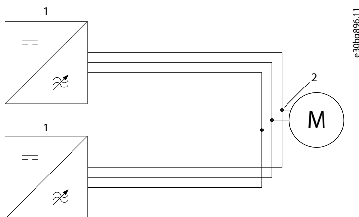
Figure 39: Recommended Installation
