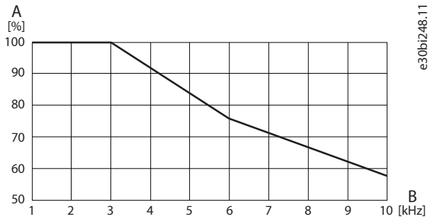
Figure 128: Output Current Derating vs. Switching Frequency (INU)
