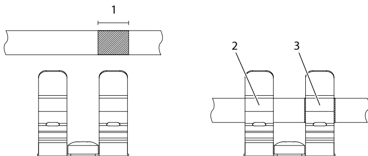
Figure 74: Stripping the Cable and Using the Grounding Plates
