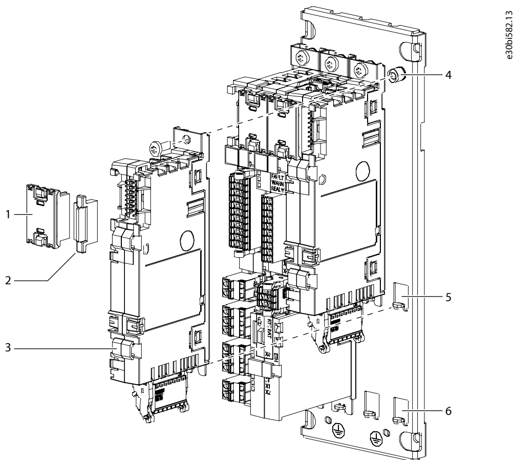
Figure 71: Installing a Board to the Modular Control Unit Mounting Plate
