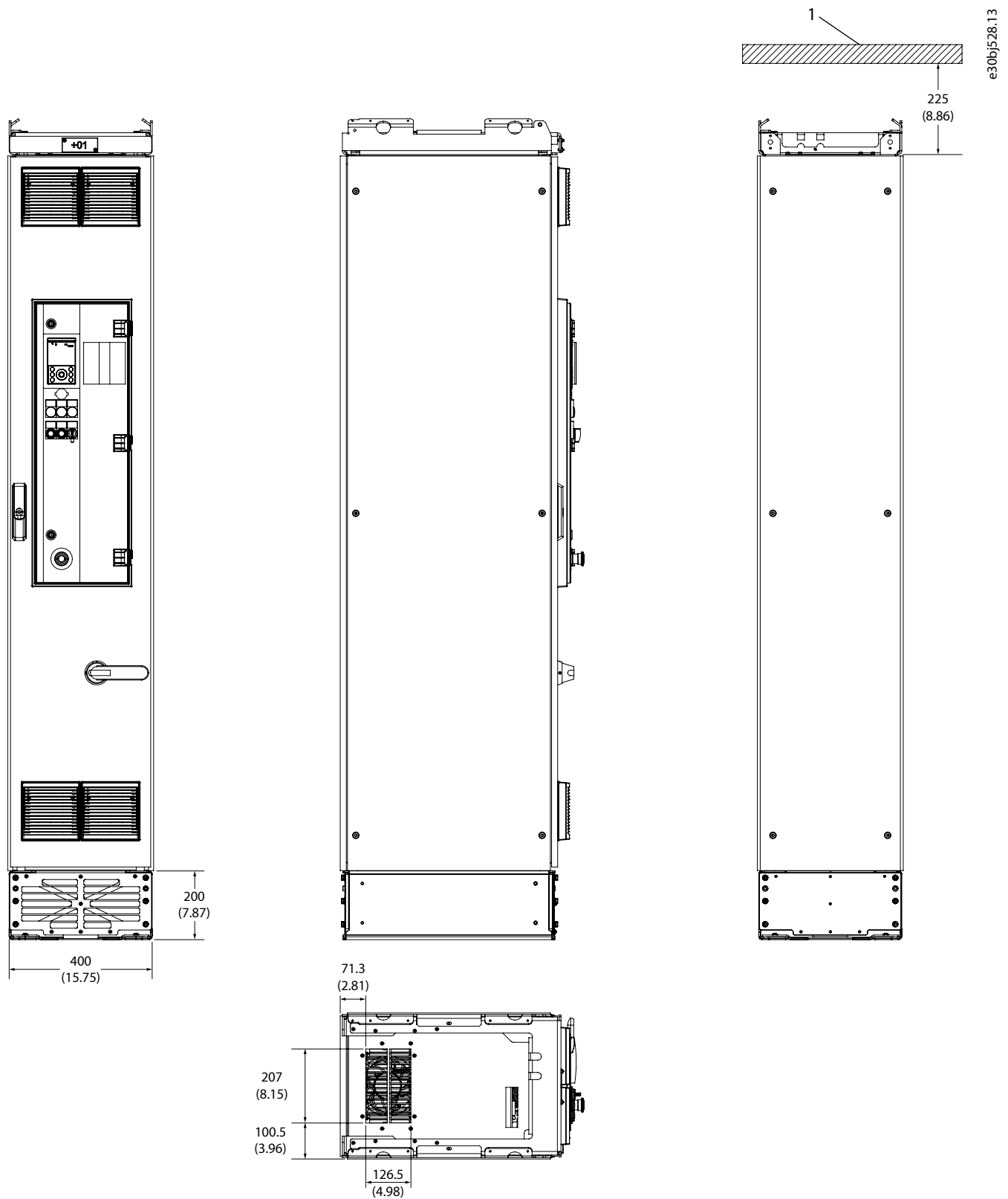
Figure 90: Dimensions for Default Cooling, FE9, in mm (in)
