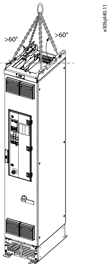
Figure 12: Lifting the Enclosed Drive
