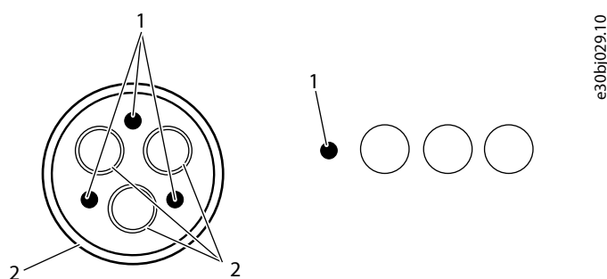
Figure 37: Not Recommended Motor Cable Types
