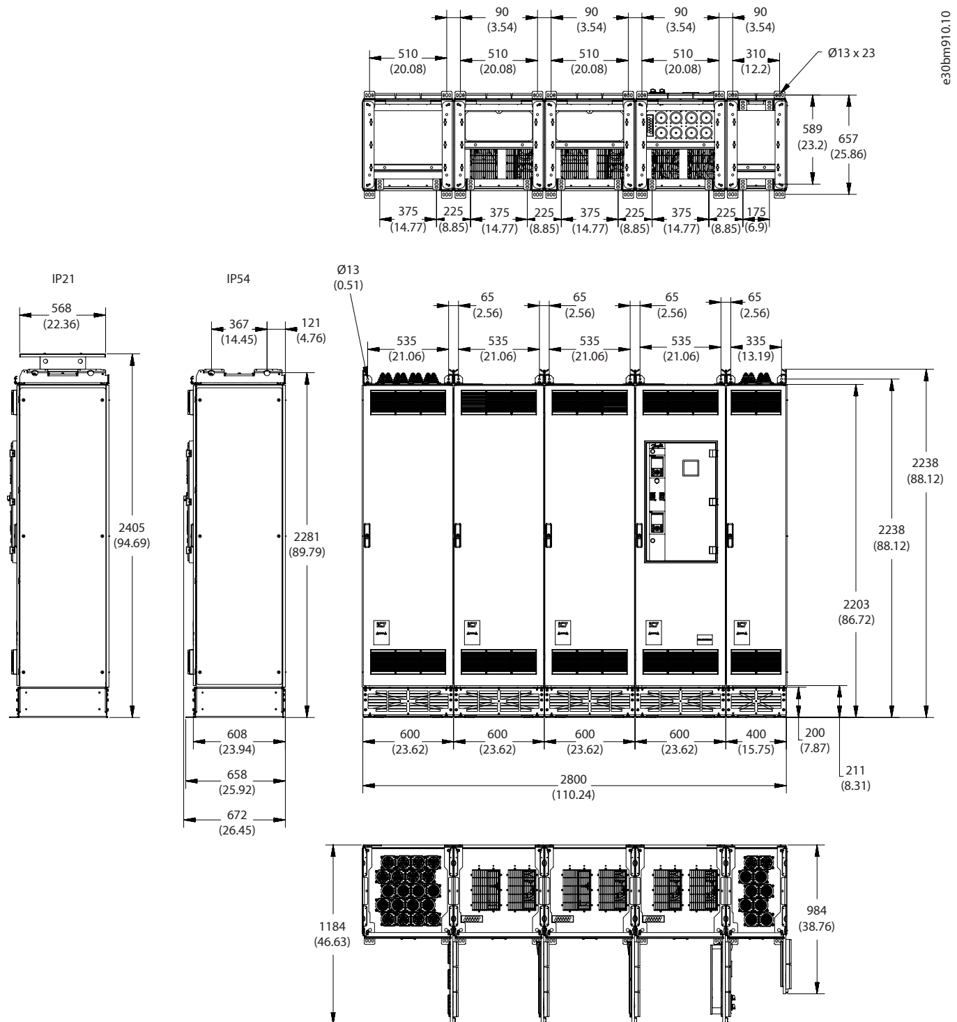
Figure 89: Dimensions for the Top Cabling Option, 2 x AE11, 2 x IE11, in mm (in)
