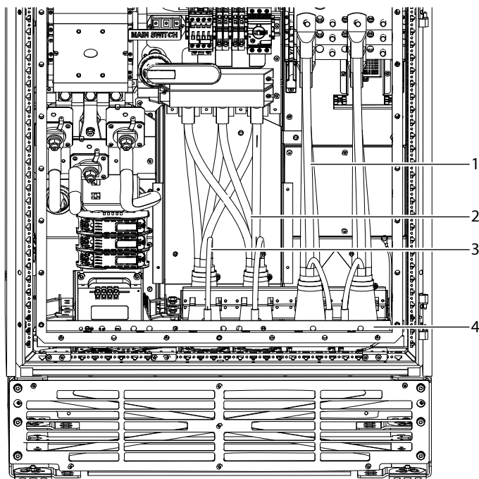
Figure 49: Cabling of the Enclosed Drive
