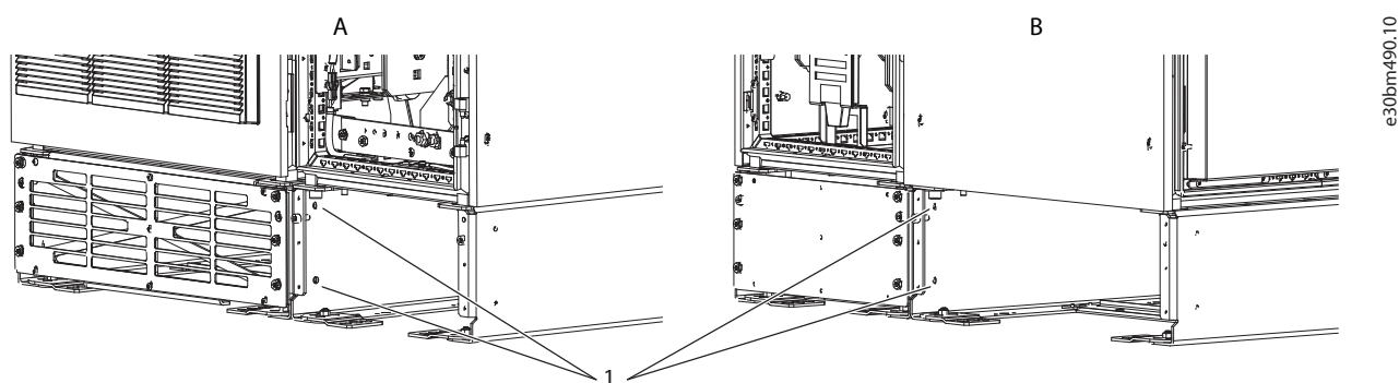
Figure 22: Attaching the Cabinet Sections from the Plinths
