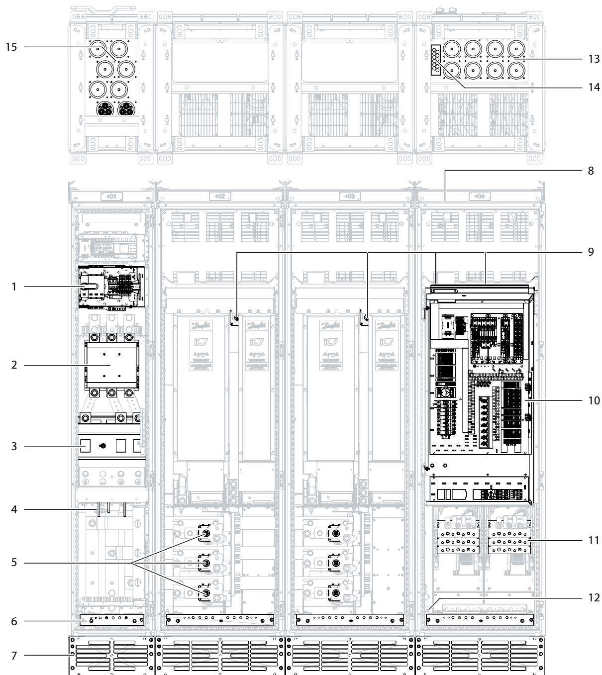
Figure 6: Interior View of the Cabinet, 2 x AE10 + 2 x IE10
