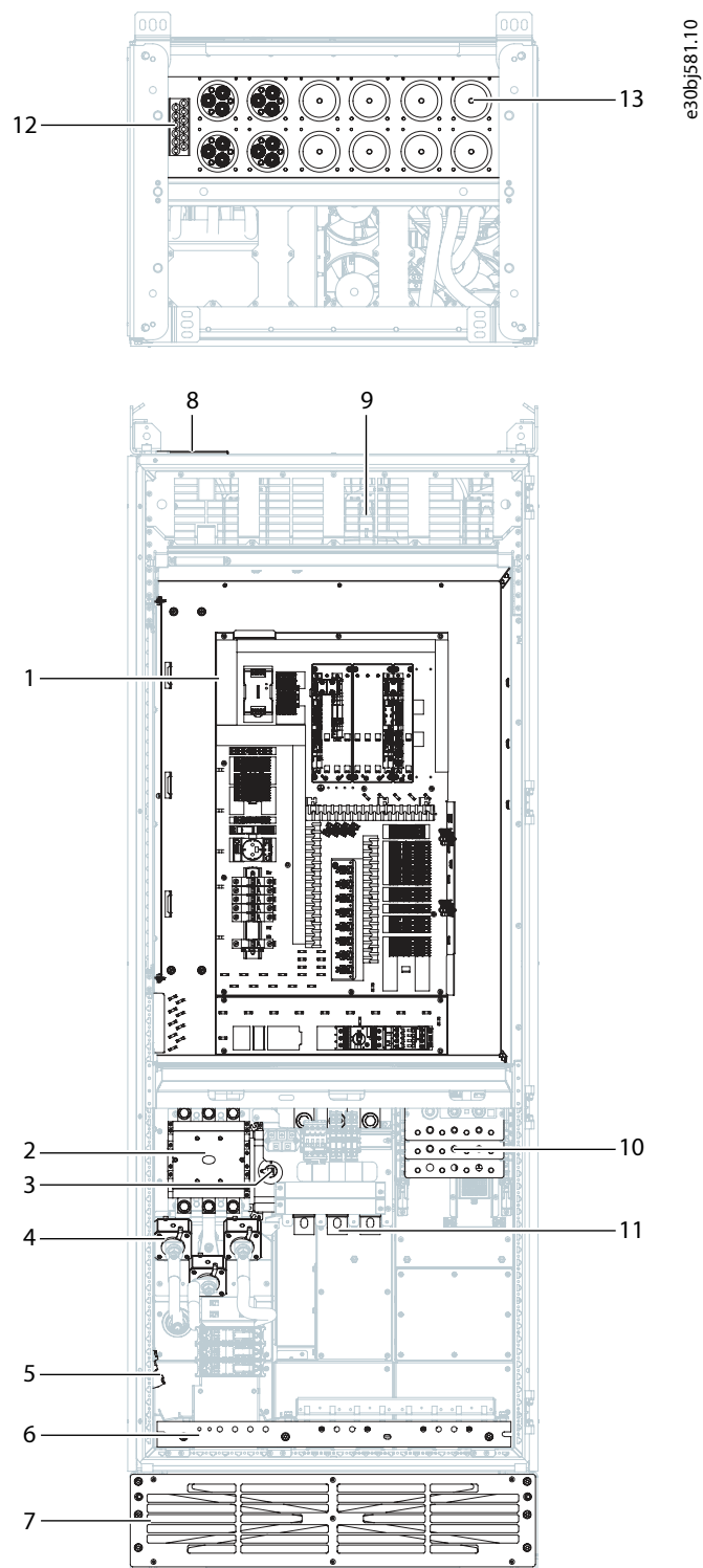
Figure 5: Interior View of the Cabinet, AE10 + IE10
