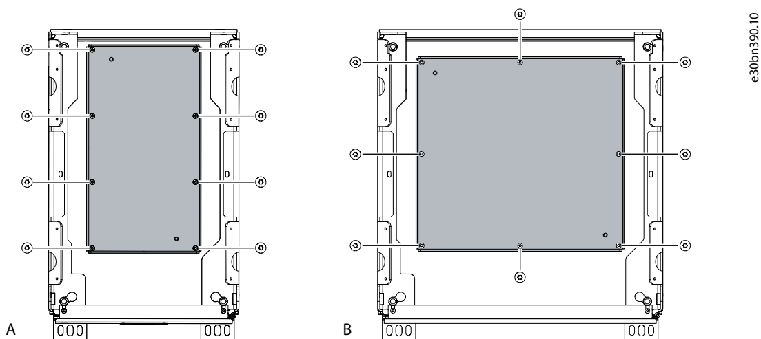
Figure 50: Releasing the Gland Plate from the Roof of the Module Cabinet Section
