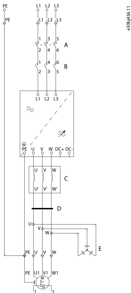
Figure 115: Wiring Diagram, FE9, FE10
