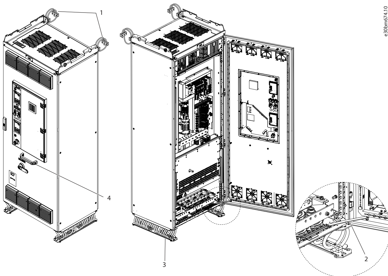
Figure 35: Components of the Marine Construction Option +AFMC
