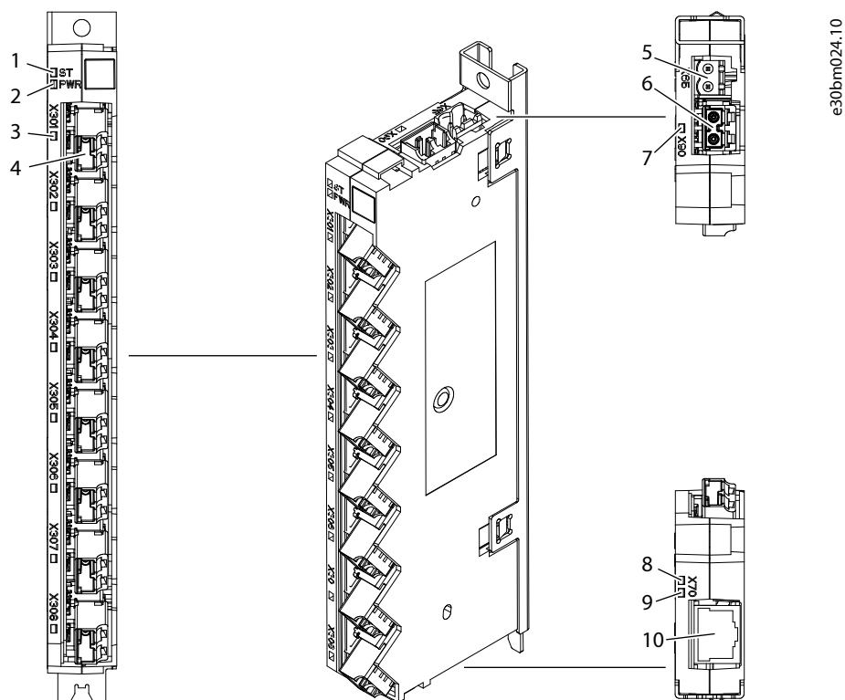
Figure 63: Terminal and Indicator Light Locations on the 8-port Star Coupler Board
