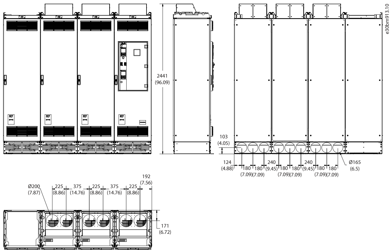
Figure 107: Dimensions for the Cooling Air Output Flange Option (+OAOF), 2 x AE11, 2 x IE11, in mm (in)
