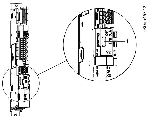
Figure 76: Location of the RTC Battery
