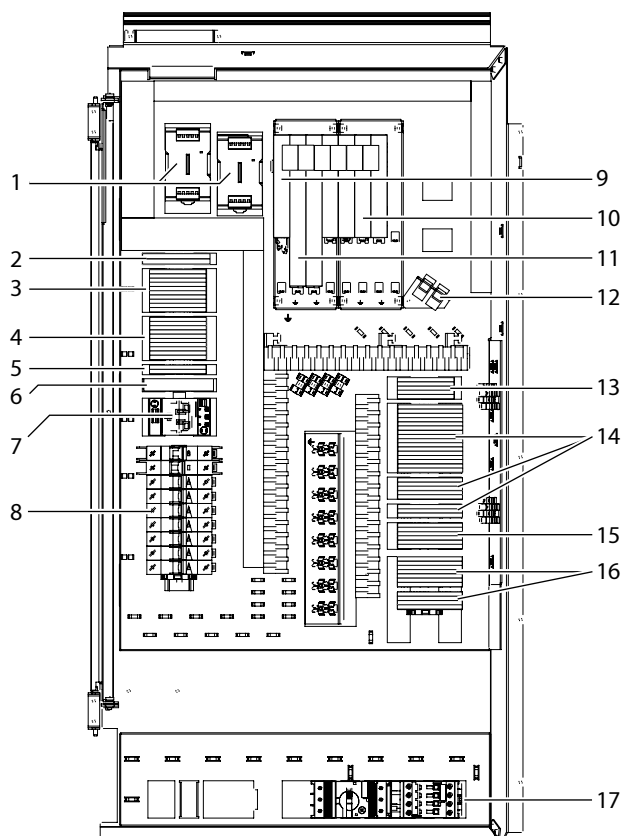
Figure 60: Elements inside the Control Compartment, FE10
