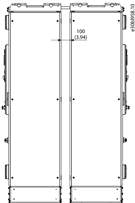
Figure 15: Installation of Cabinets Back to Back, mm (in)
