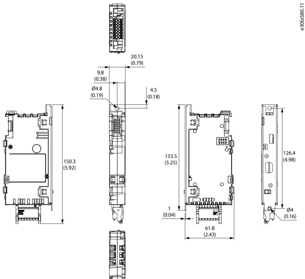
Figure 111: Dimensions of an Option Board in mm (in)
