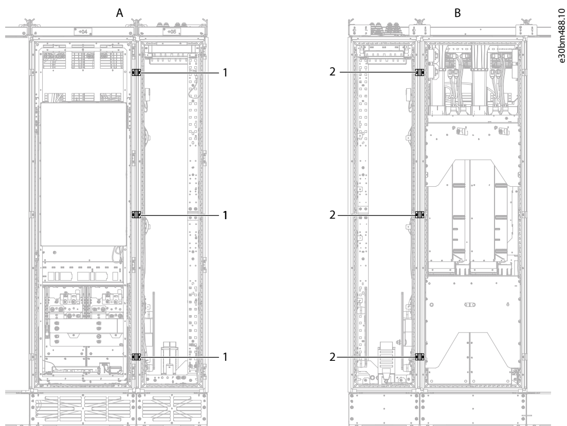
Figure 21: Attach the Connection Pieces to the Output Cabinet Section
