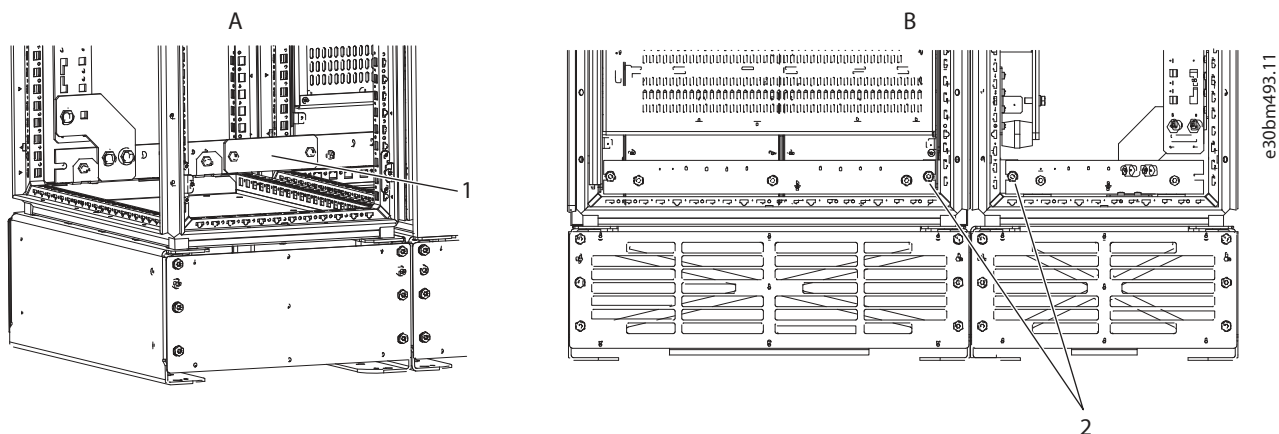
Figure 25: Installing the PE Connection Busbar
