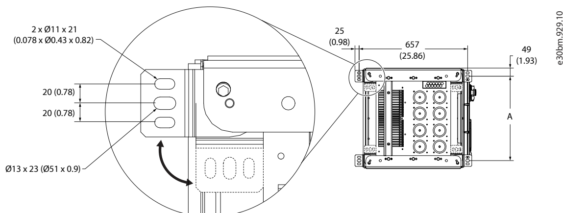
Figure 79: Dimensions of the Cabinet Feet, in mm (in)
