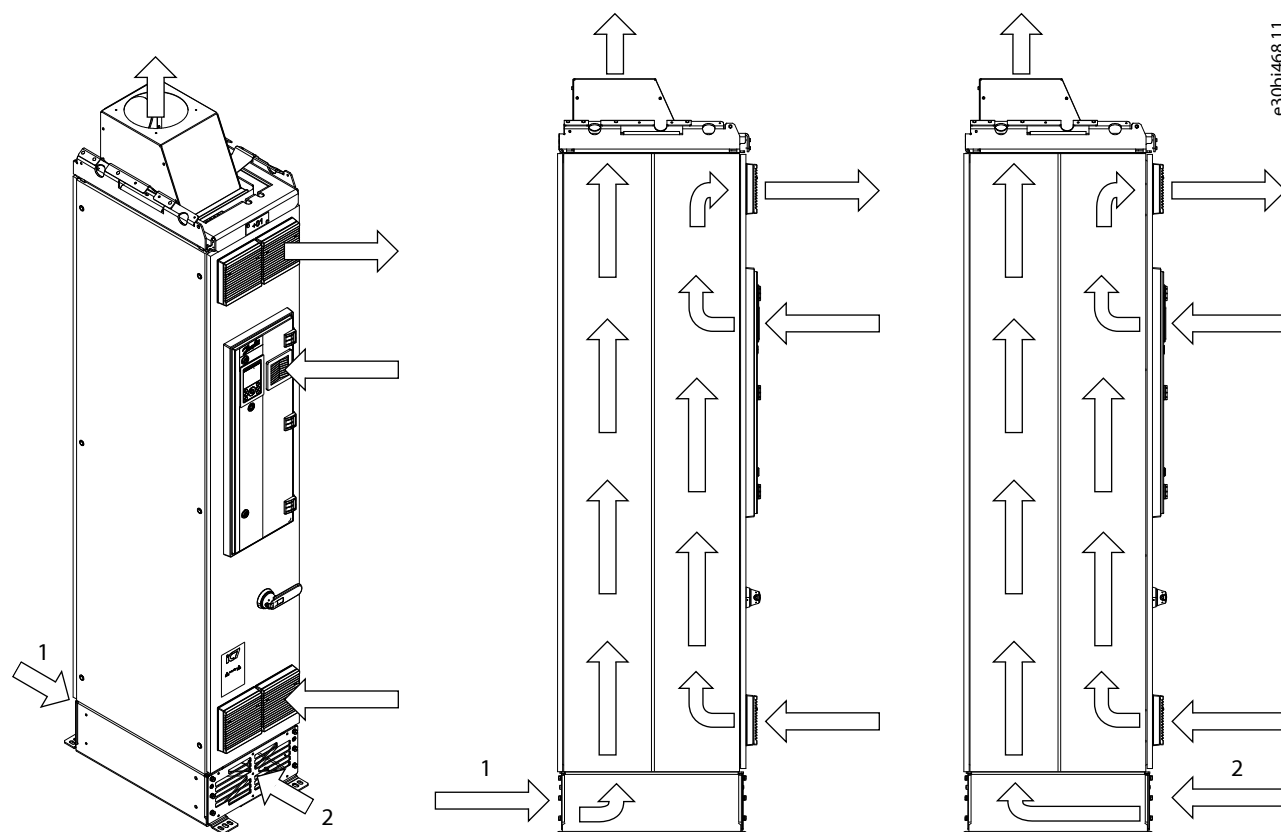
Figure 31: Cooling Air Output Flange (+OAOF), Intake Front or Back, Output Top
