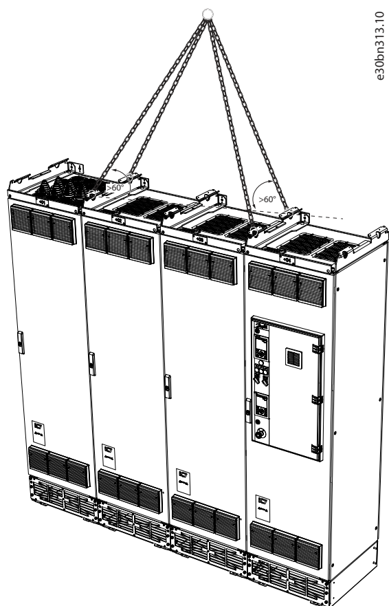
Figure 13: Lifting the Enclosed Drive with Several Cabinet Sections
