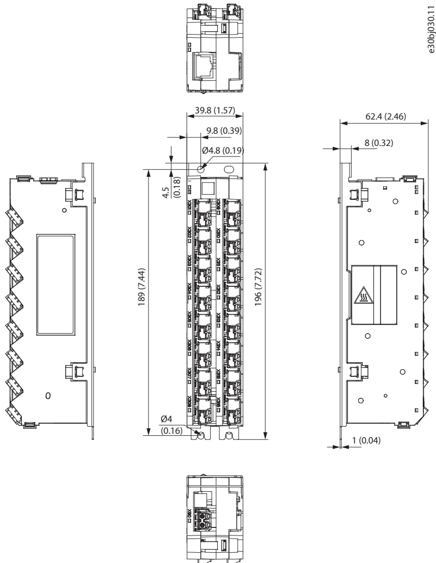
Figure 114: Dimensions of the 16-port Star Coupler Board in mm (in)
