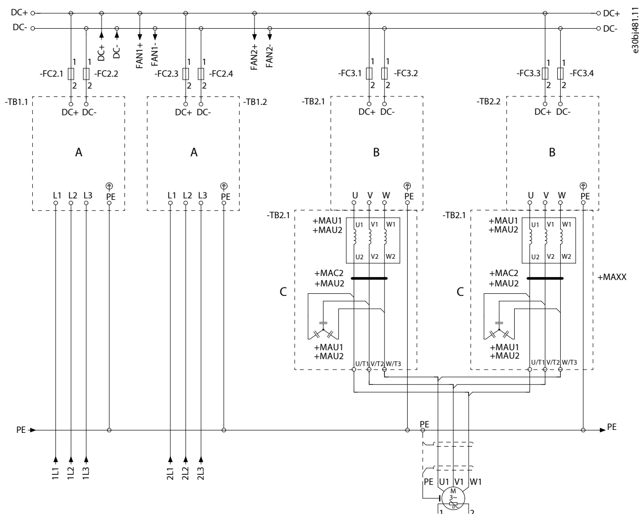
Figure 123: Wiring Diagram, 2 x AE11+2 x IE11, 1260-1710 A (continued)
