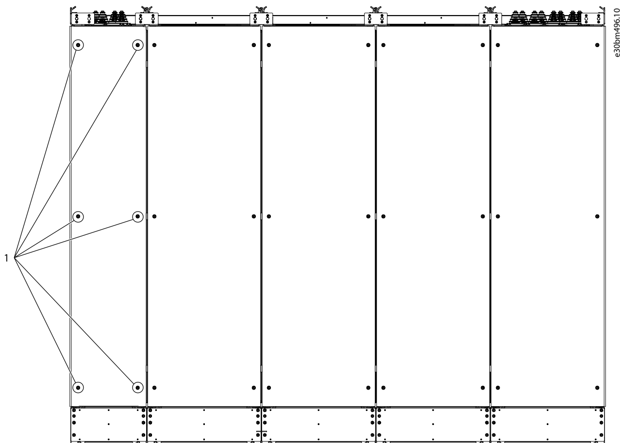
Figure 28: Attaching the Back Wall to the Cabinet Section
