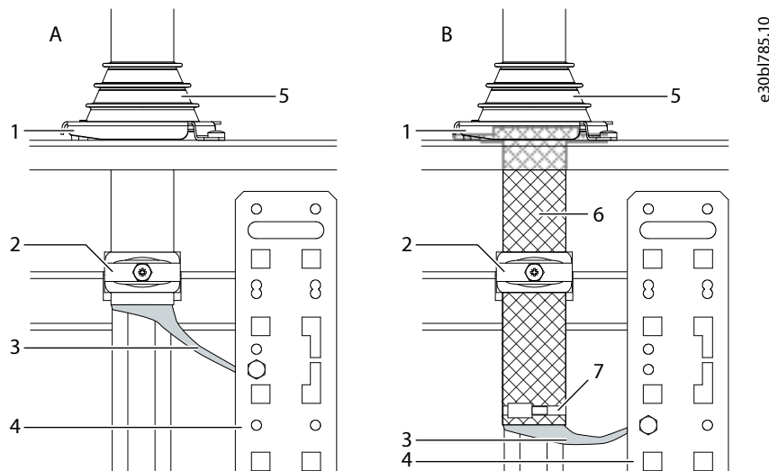
Figure 52: Cabling Methods (IEC)
