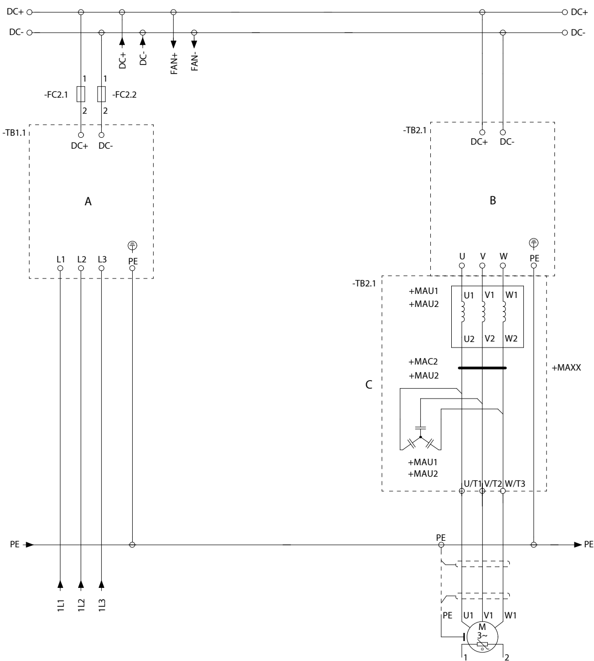
Figure 119: Wiring Diagram, AE11+IE11, 658-880 A (continued)
