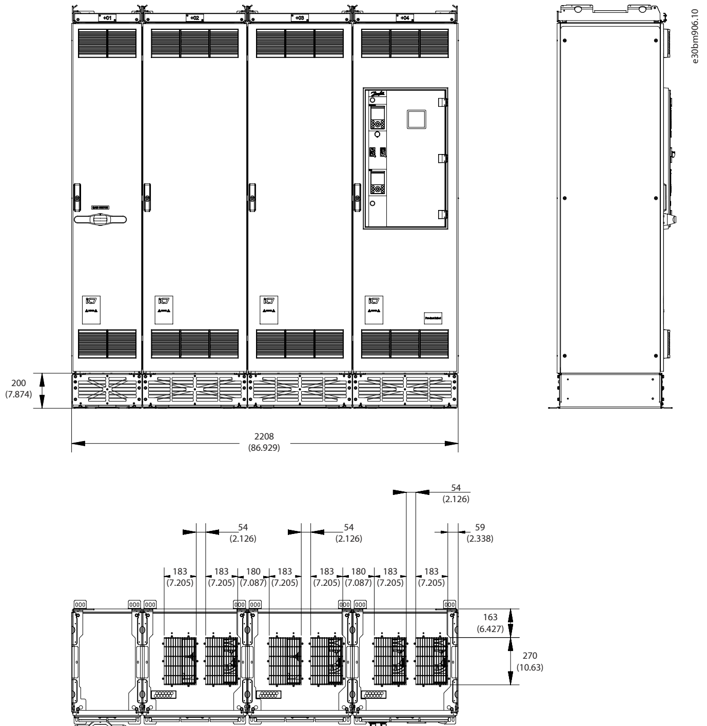
Figure 94: Dimensions for Default Cooling, 2 x AE10, 2 x IE10, in mm (in)
