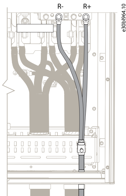
Figure 56: Installing the Brake Cables in the Enclosed Drive, FE9, FE10
