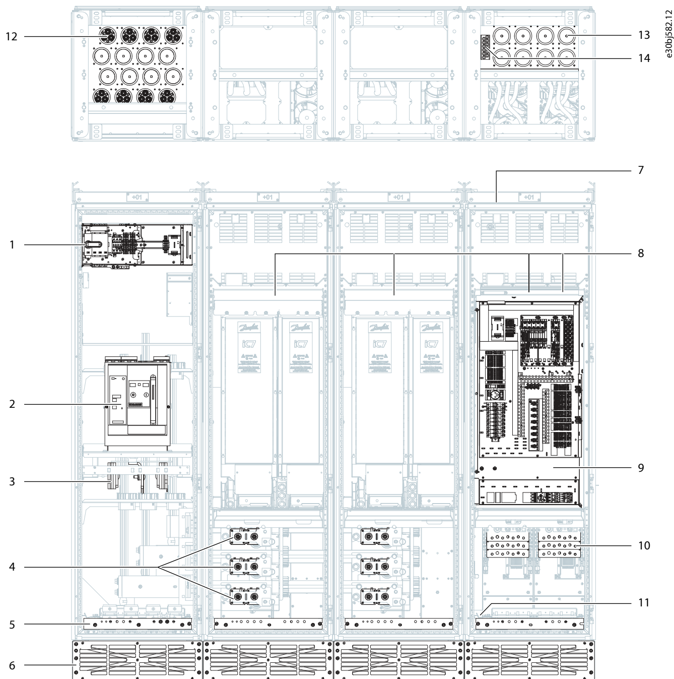
Figure 8: Interior View of the Cabinet, 2 x AE11 + 2 x IE11
