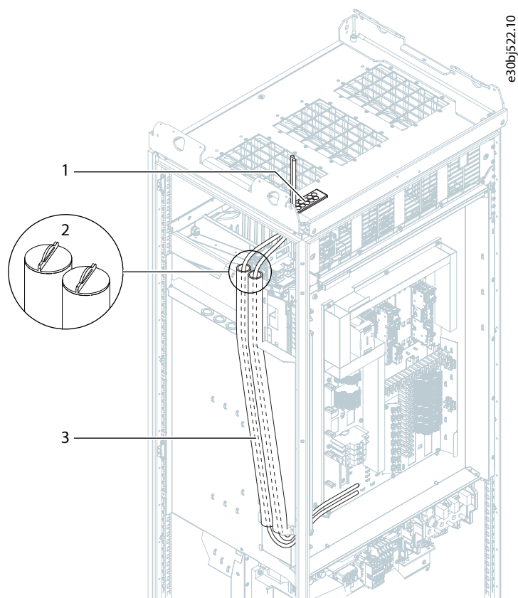
Figure 68: Routing of Control Cables from the Top, AE10/11, IE10/11
