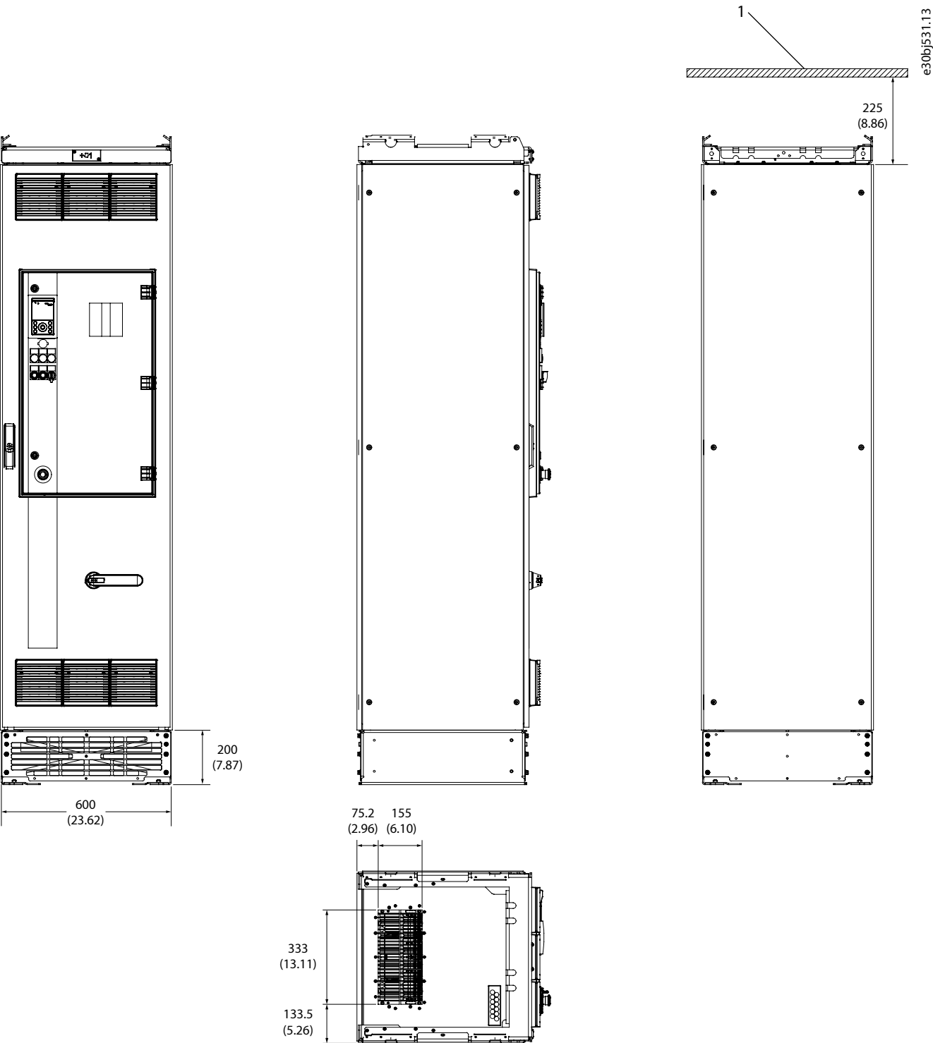
Figure 91: Dimensions for Default Cooling, FE10, in mm (in)
