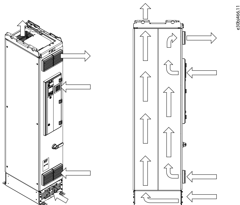
Figure 29: Airflow in Default Cooling of the Enclosed Drives
