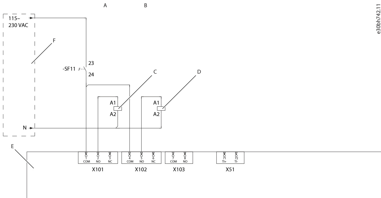
Figure 125: Pre-charging Control Wiring Diagram, AE10, AE11, IE10, IE11
