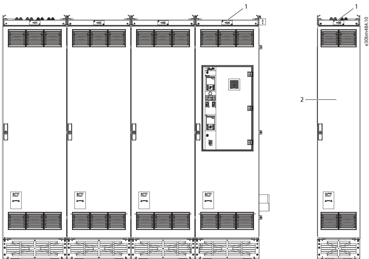
Figure 17: Attaching the Output Cabinet Section to the Other Cabinet Sections (Example)
