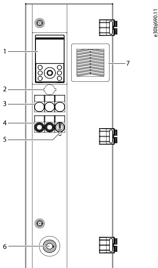
Figure 57: Control Compartment Door Elements, FE9, FE10
