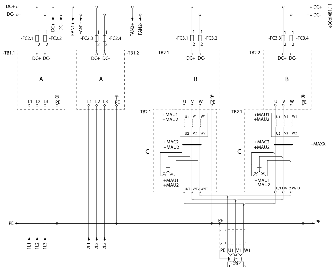
Figure 121: Wiring Diagram, 2 x AE10+2 x IE10, 1000–1100 A (continued)
