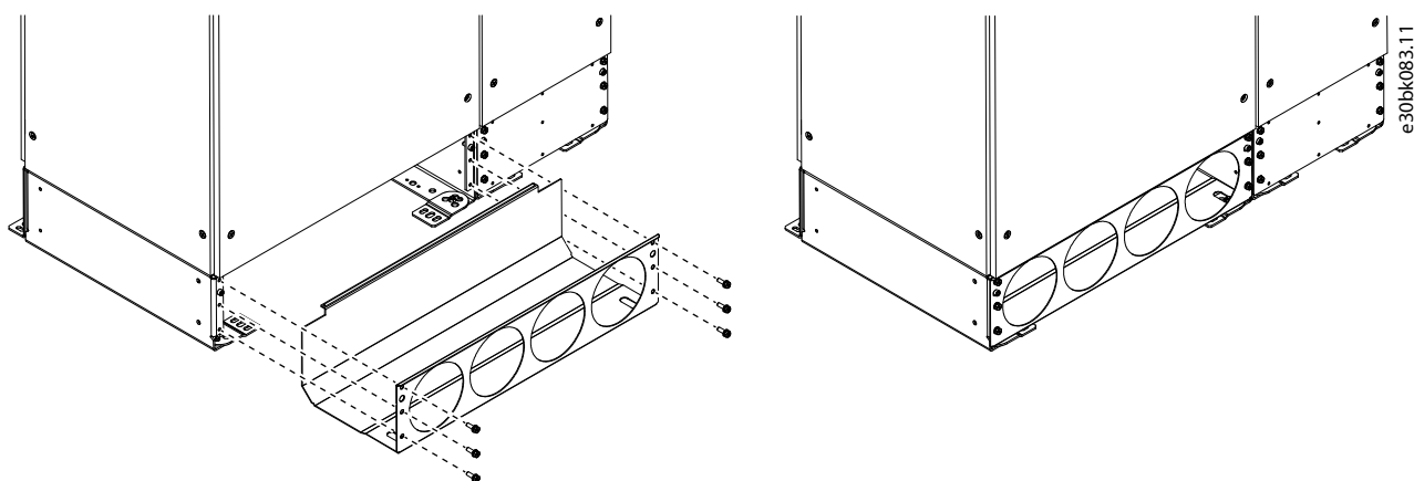
Figure 34: Back-channel Cooling Option Air Guide at the Bottom
