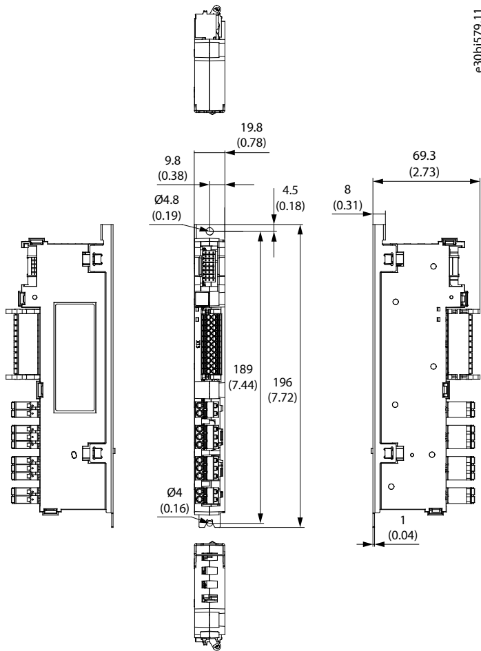
Figure 110: Dimensions of the I/O and Relay Option in mm (in)
