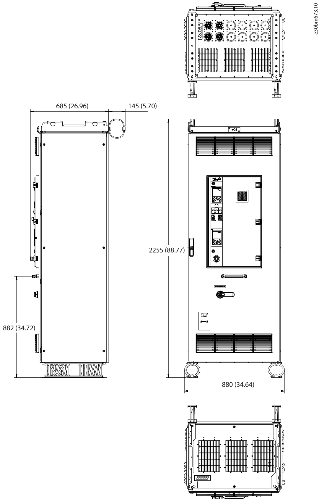
Figure 108: Dimensions for the Marine Construction Option, +AFMC
