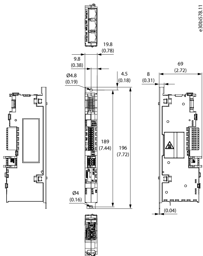
Figure 109: Dimensions of the Control Board in mm (in)
