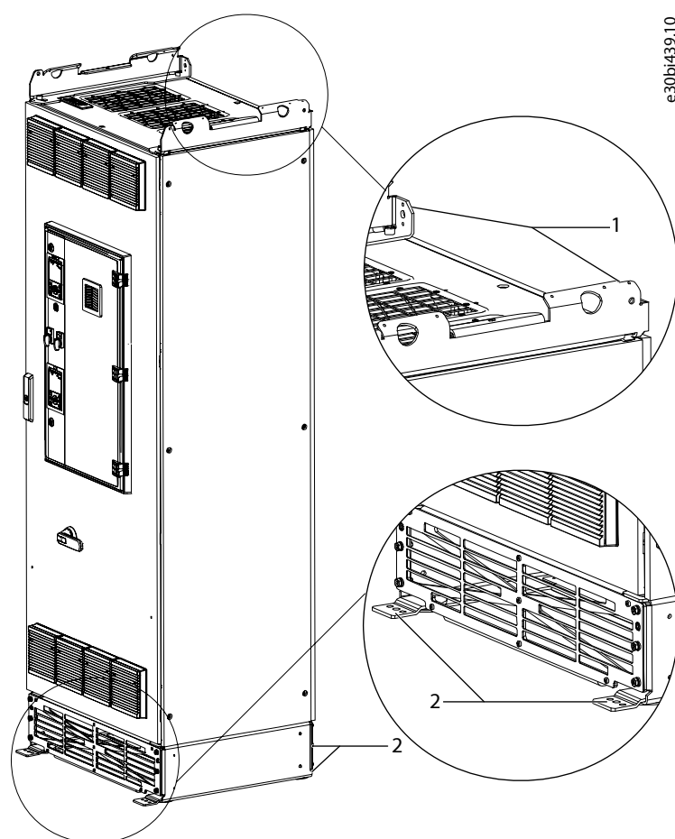
Figure 14: Installing the Enclosed Drive, FE9, FE10
