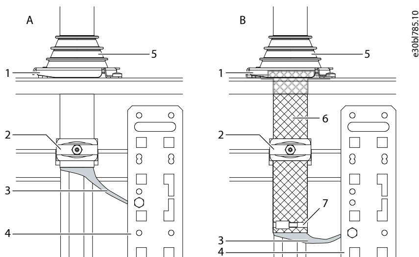
Figure 43: Cabling Methods (IEC)
