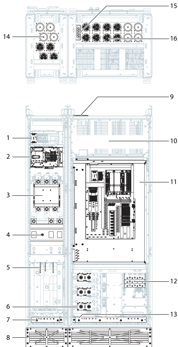
Figure 7: Interior View of the Cabinet, AE11 + IE11
