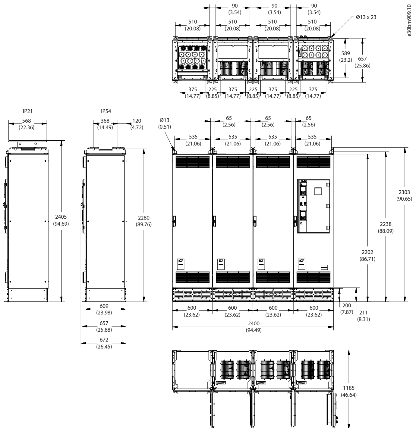
Figure 85: Dimensions for the Bottom Cabling Option, 2 x AE11, 2 x IE11, in mm (in)
