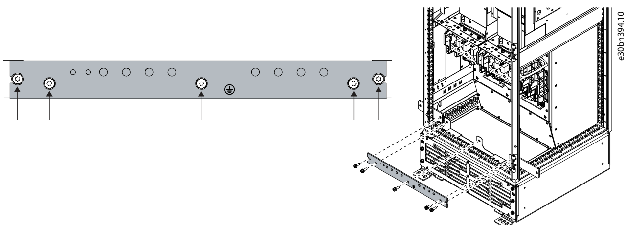
Figure 54: Removing the PE Busbar
