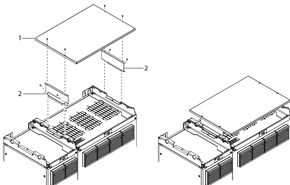
Figure 16: Installing the IP21 Top Cover
