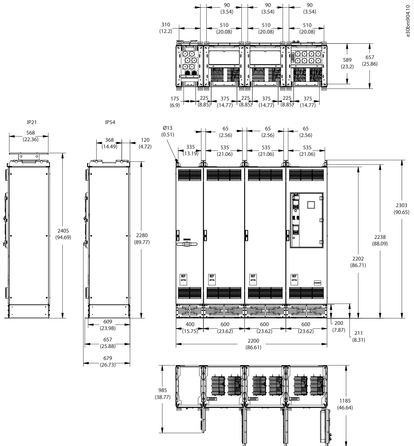
Figure 84: Dimensions for the Bottom Cabling Option, 2 x AE10, 2 x IE10, in mm (in)
