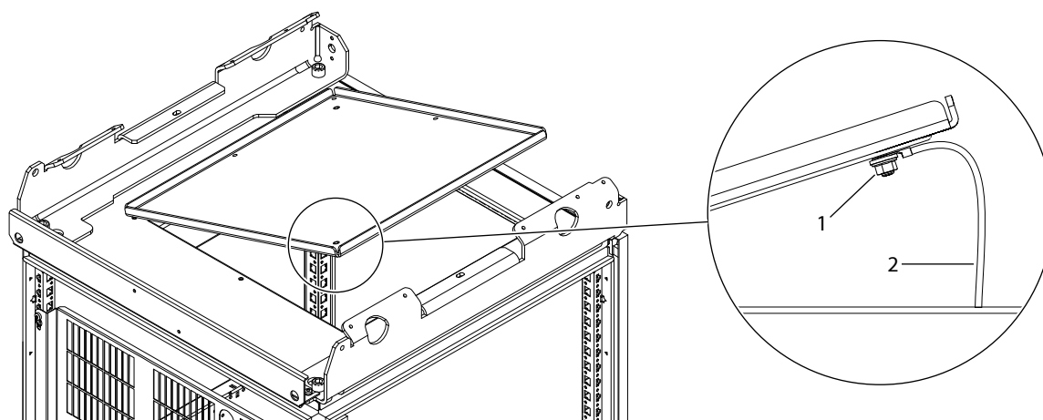
Figure 51: Opening the Gland Plate and Releasing the Grounding Wire
