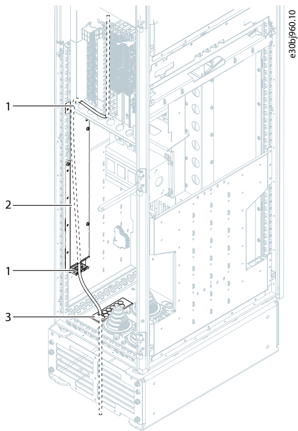
Figure 69: Routing of Control Cables from the Bottom, FE9, FE10
