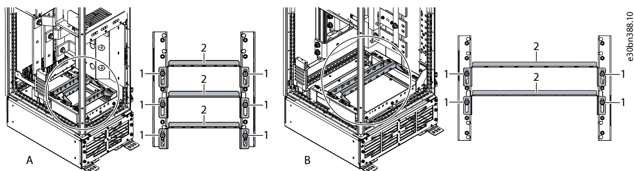
Figure 45: Removing the Cable Supports
