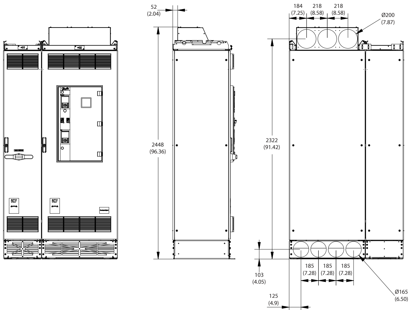
Figure 99: Dimensions for Back-channel Cooling (+OABC), AE11, IE11, in mm (in)
