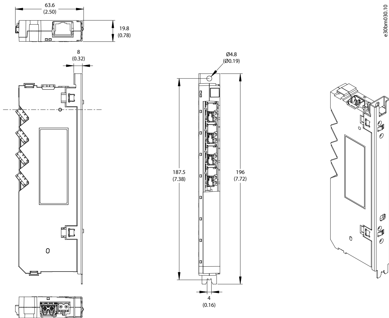
Figure 112: Dimensions of the 4-port Star Coupler Board in mm (in)
