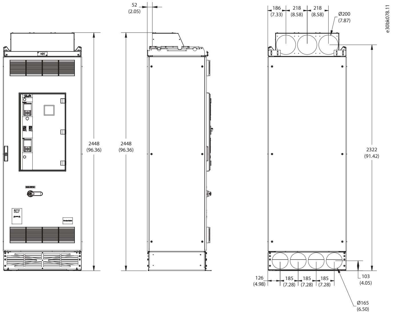
Figure 98: Dimensions for Back-channel Cooling (+OABC), AE10, IE10, in mm (in)
