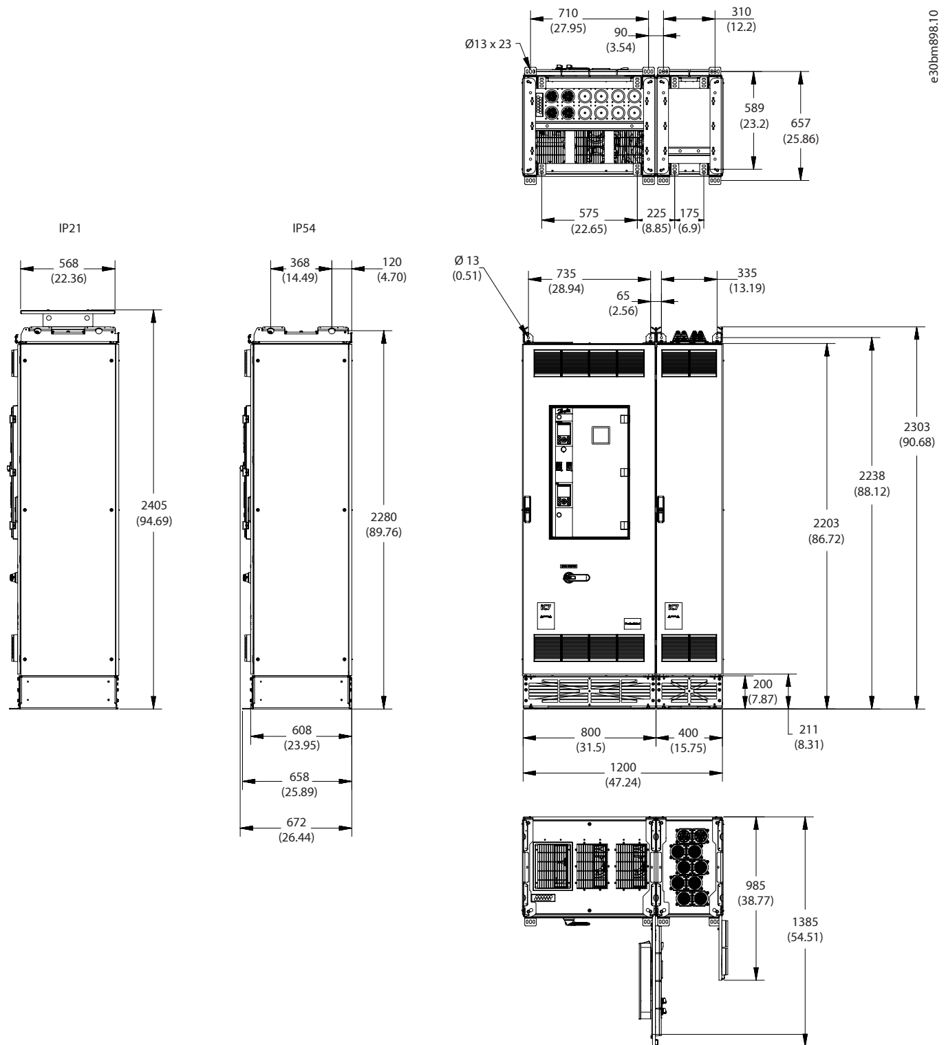
Figure 86: Dimensions for the Top Cabling Option, AE10, IE10, in mm (in)
