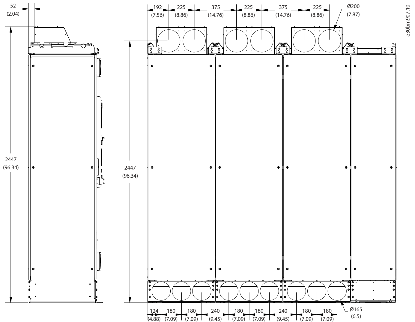
Figure 100: Dimensions for Back-channel Cooling (+OABC), 2 x AE10, 2 x IE10, in mm (in)
