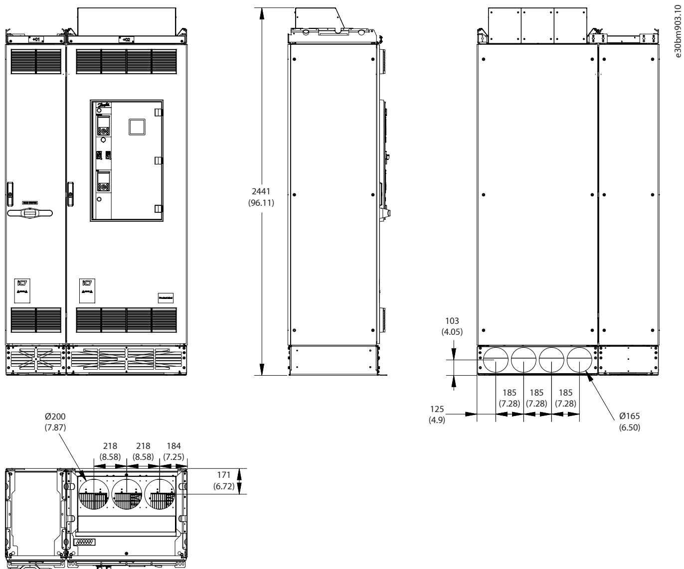
Figure 105: Dimensions for the Cooling Air Output Flange Option (+OAF), AE11, IE11, in mm (in)
