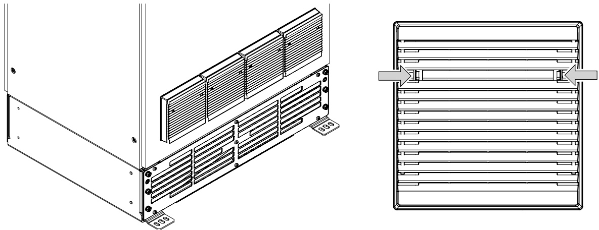
Figure 78: Removing the Fan Grill
