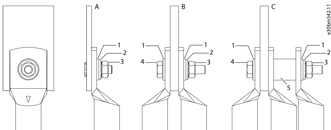
Figure 44: Connecting the Power Cables to the Terminals
