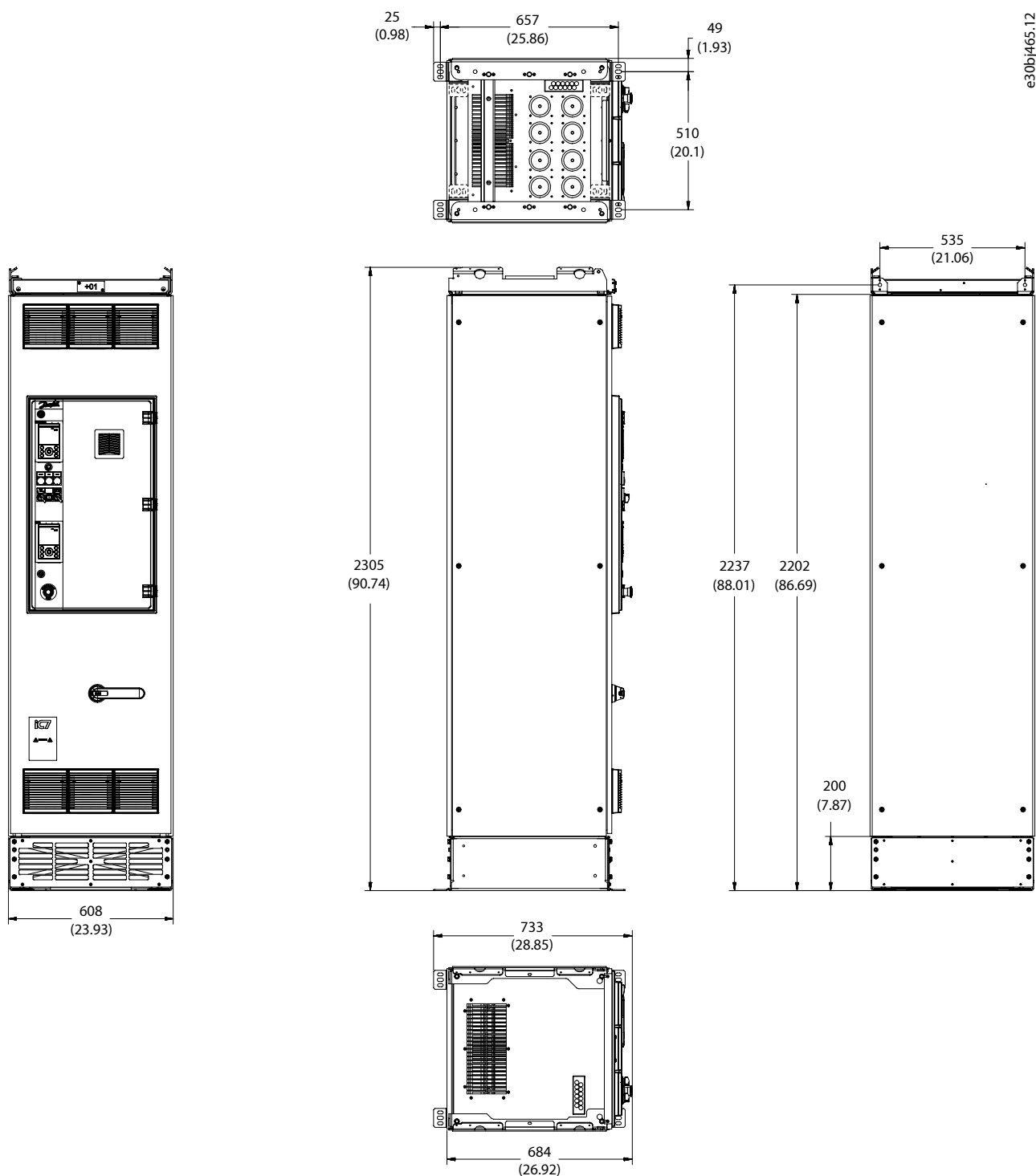
Figure 81: Dimensions of the Enclosed Drive, FE10, in mm (in)
