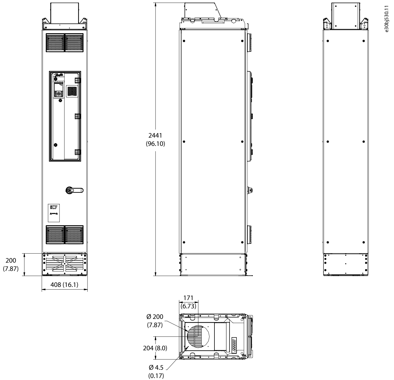
Figure 102: Dimensions for the Cooling Air Output Flange (+OAOF), FE9, in mm (in)
