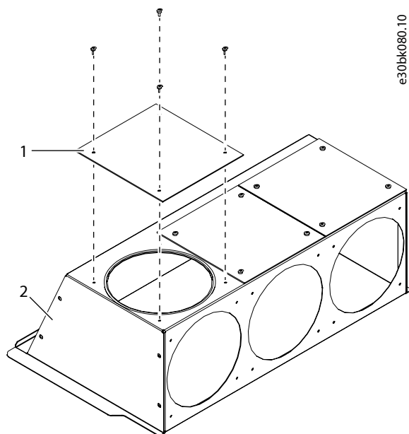
Figure 32: Installing the Back-channel Cooling Option Cover Plate
