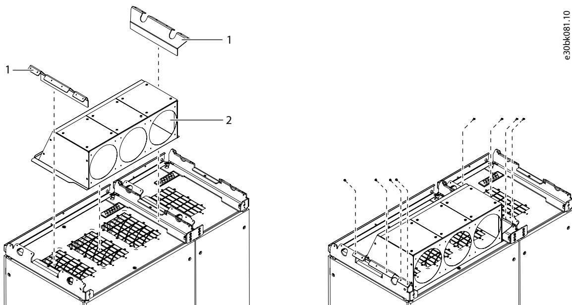
Figure 33: Installing the Back-channel Cooling Option Brackets
