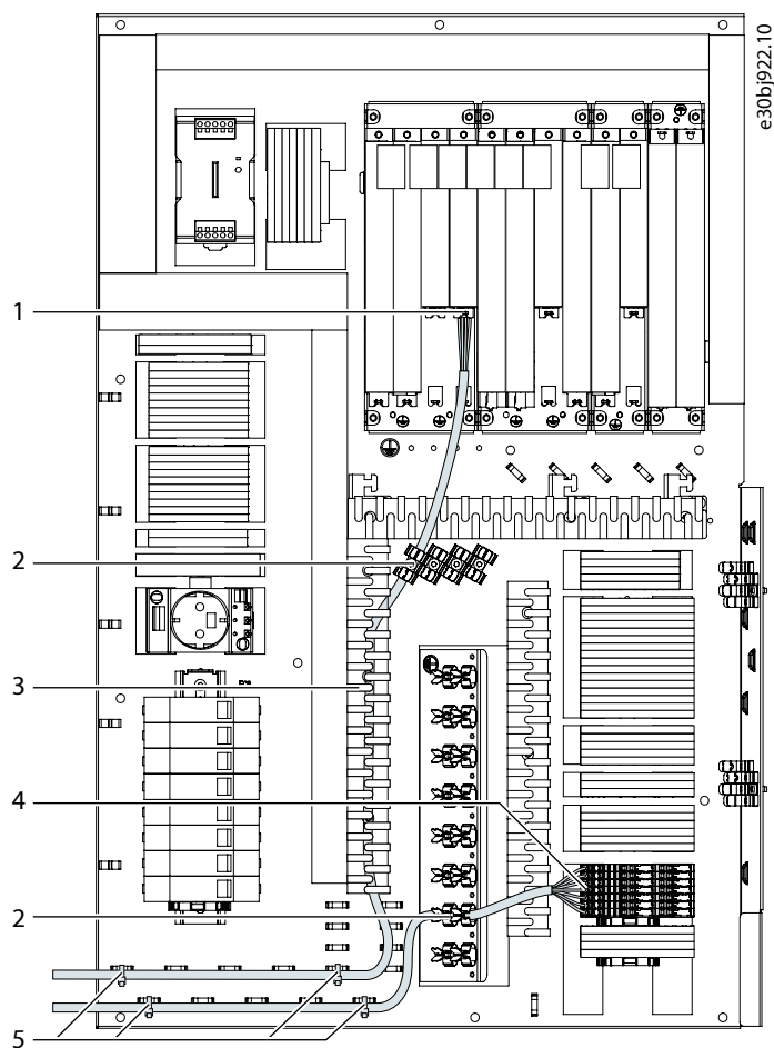
Figure 73: Example of Installing the Control Cables on Terminals Blocks
