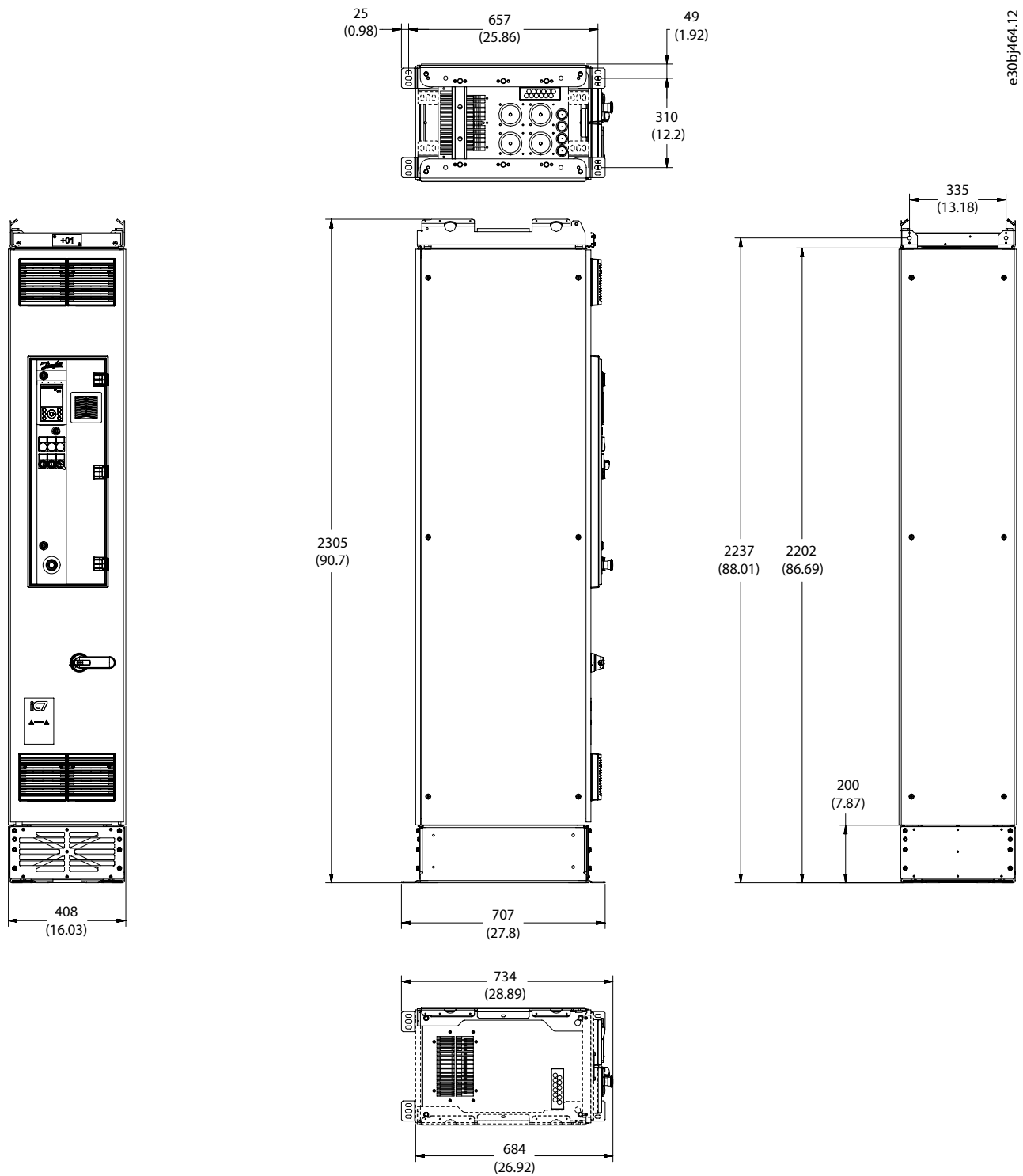
Figure 80: Dimensions of the Enclosed Drive, FE9, in mm (in)
