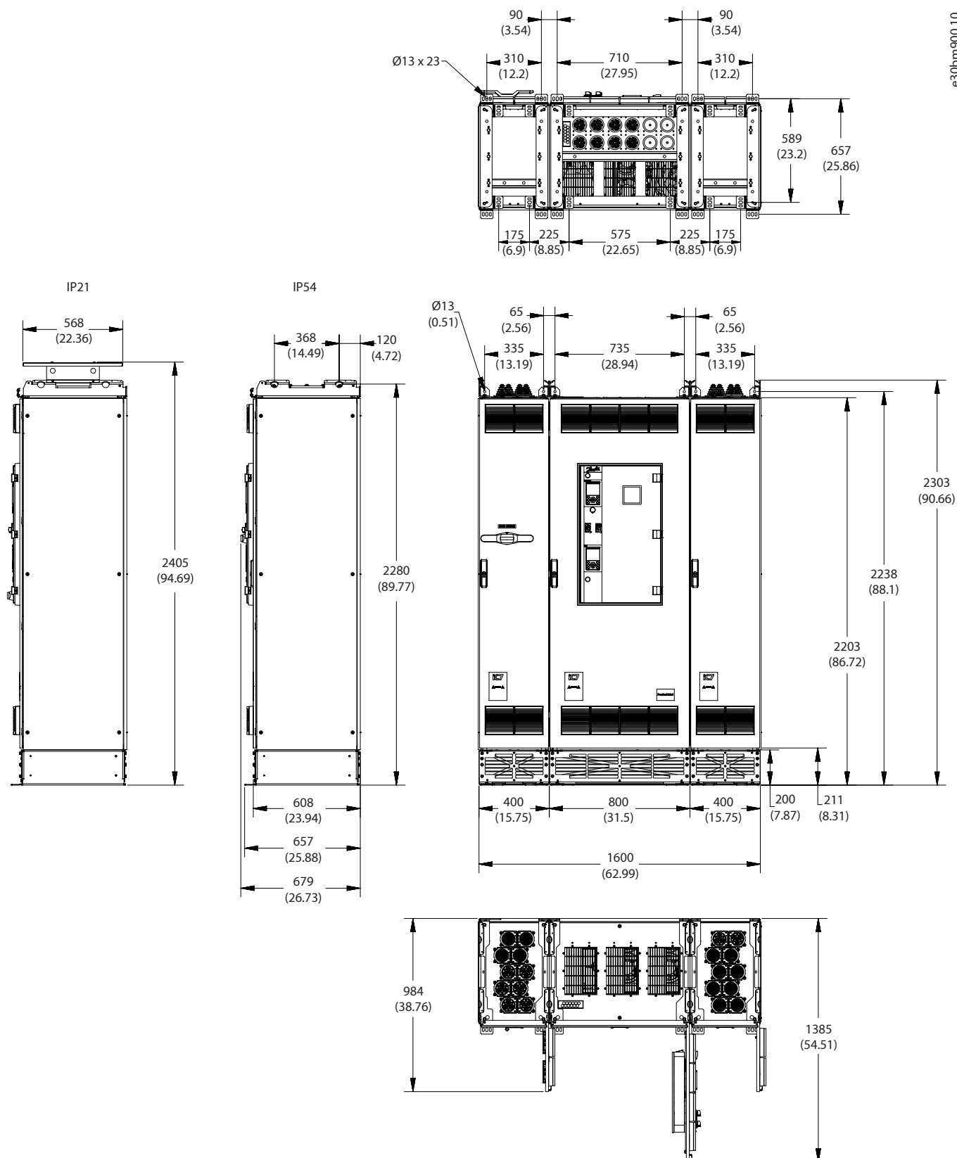
Figure 87: Dimensions for the Top Cabling Option, AE11, IE11, in mm (in)
