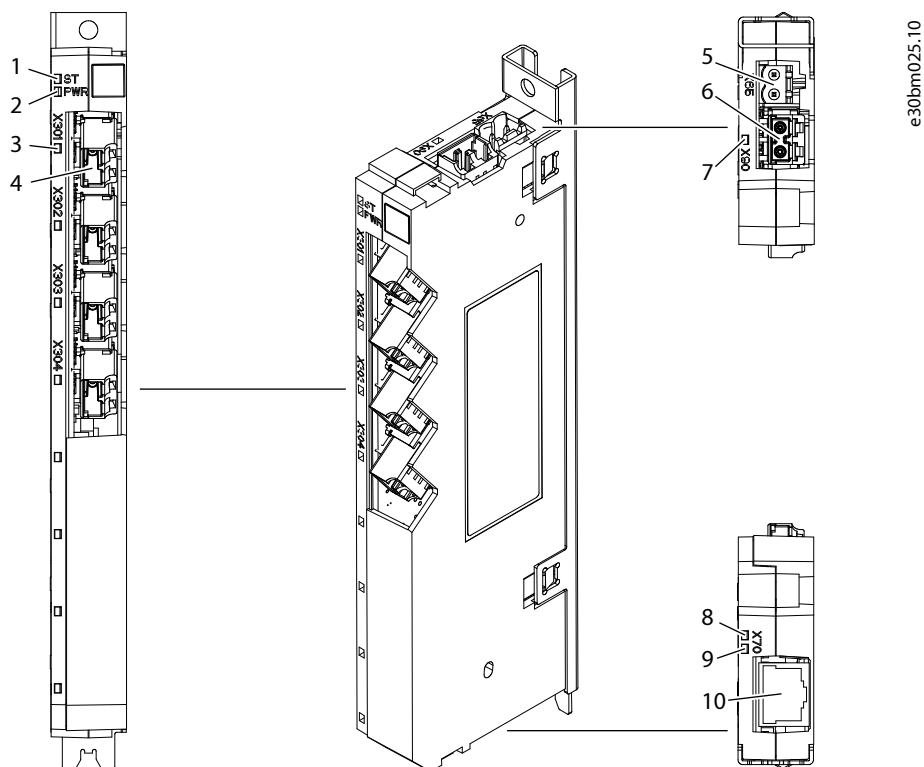
Figure 62: Terminal and Indicator Light Locations on the 4-port Star Coupler Board
