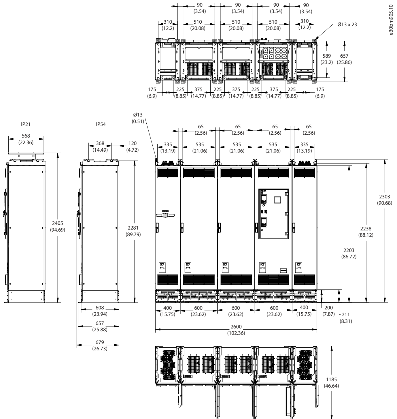
Figure 88: Dimensions for the Top Cabling Option, 2 x AE10, 2 x IE10, in mm (in)
