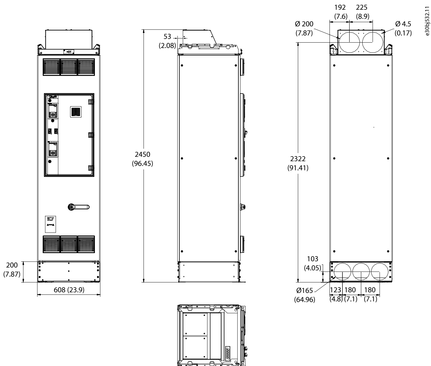
Figure 97: Dimensions for Back-channel Cooling (+OABC), FE10, in mm (in)
