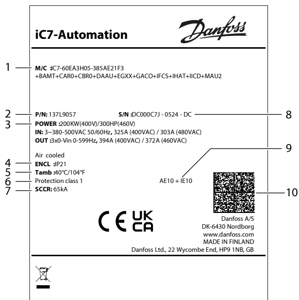
Figure 10: Product Label for iC7-Automation Enclosed Drives
