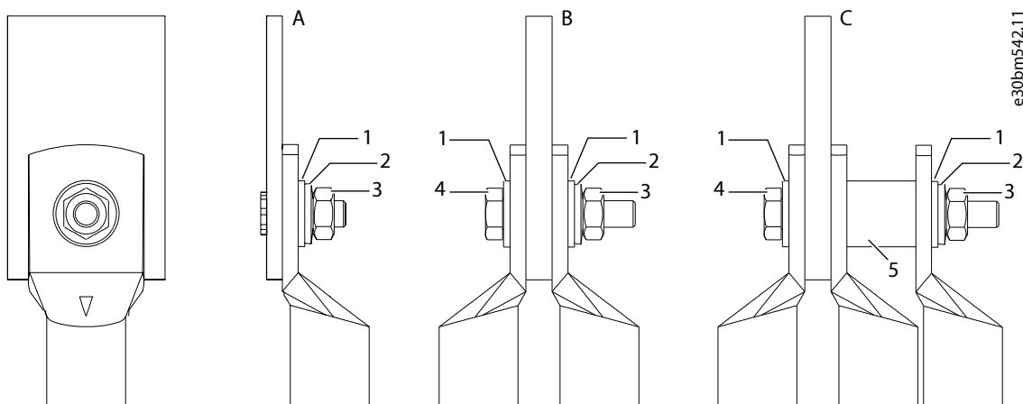
Figure 41: Connecting the Power Cables to the Terminals
