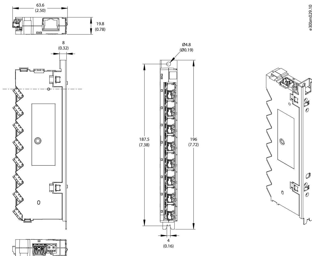
Figure 113: Dimensions of the 8-port Star Coupler Board in mm (in)
