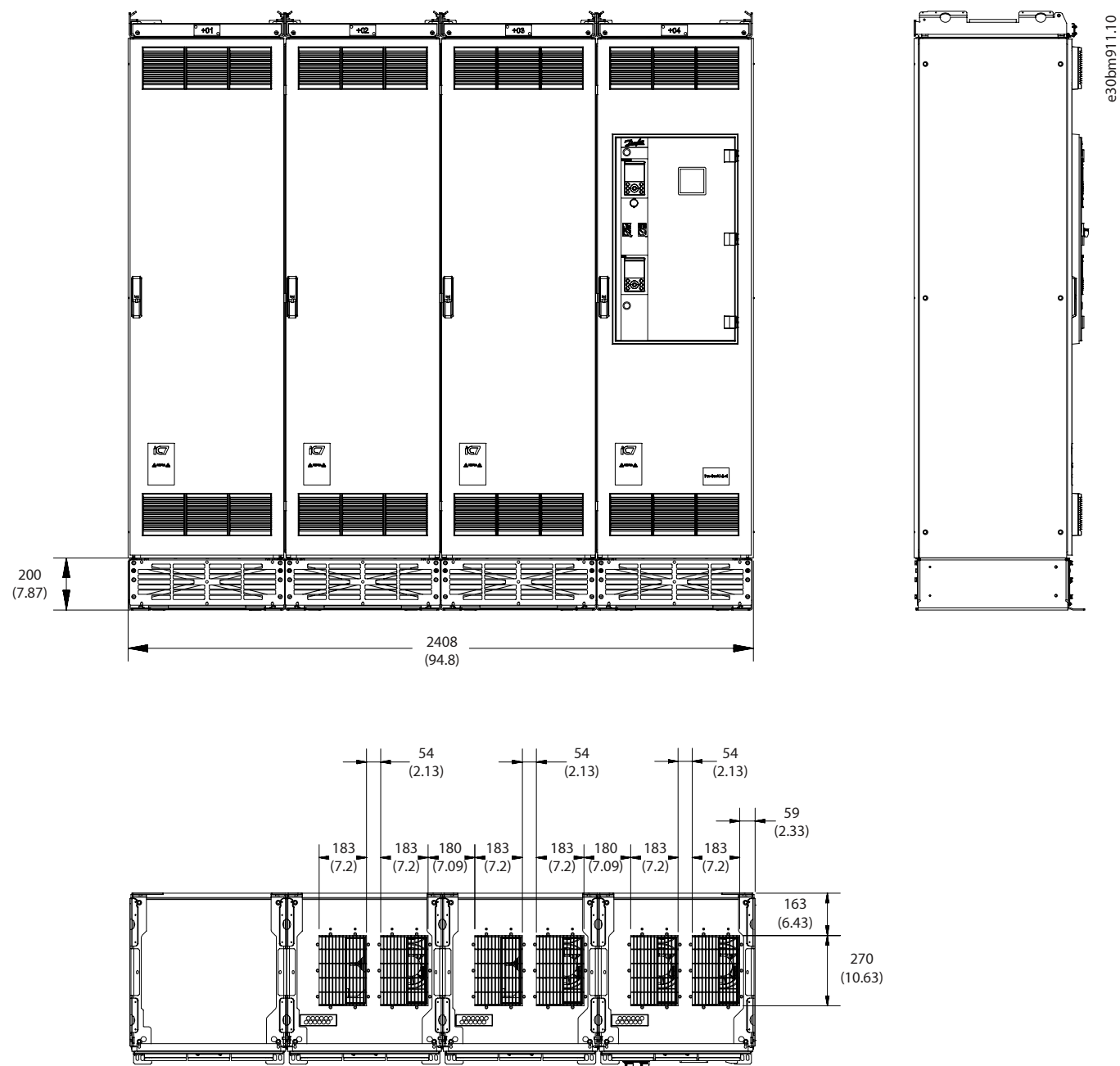
Figure 95: Dimensions for Default Cooling, 2 x AE11, 2 x IE11, in mm (in)
