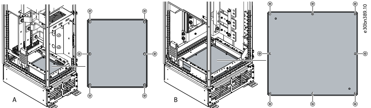
Figure 46: Removing the Gland Plate from the Bottom of the Module Cabinet Section
