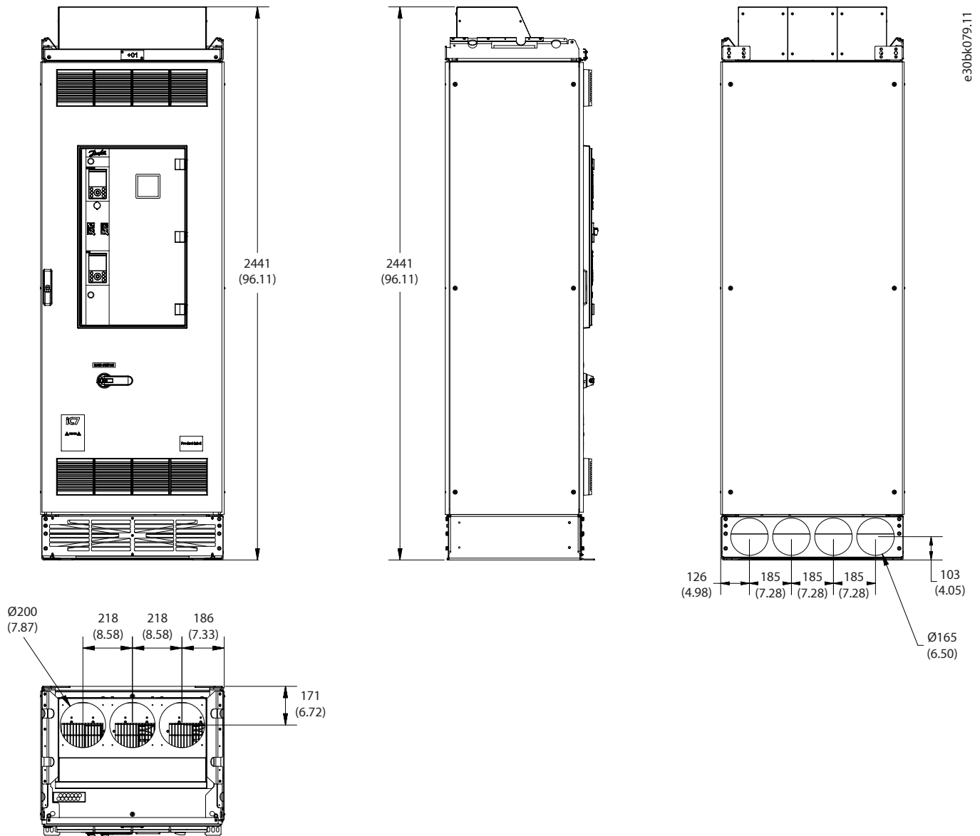
Figure 104: Dimensions for the Cooling Air Output Flange Option (+OAF), AE10, IE10, in mm (in)
