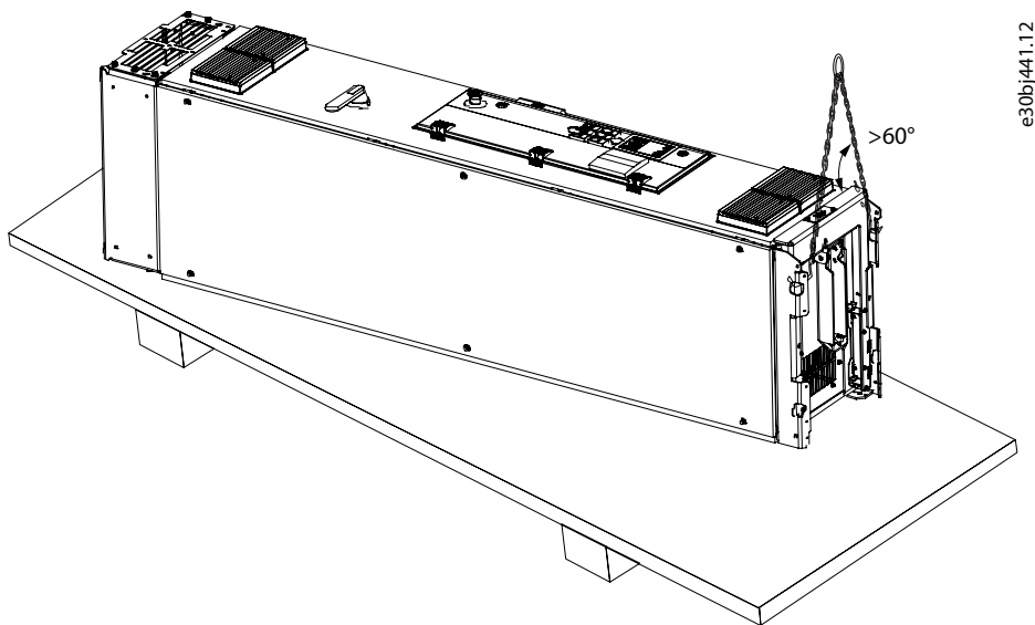
Figure 11: Lifting the Enclosed Drive to an Upright Position
