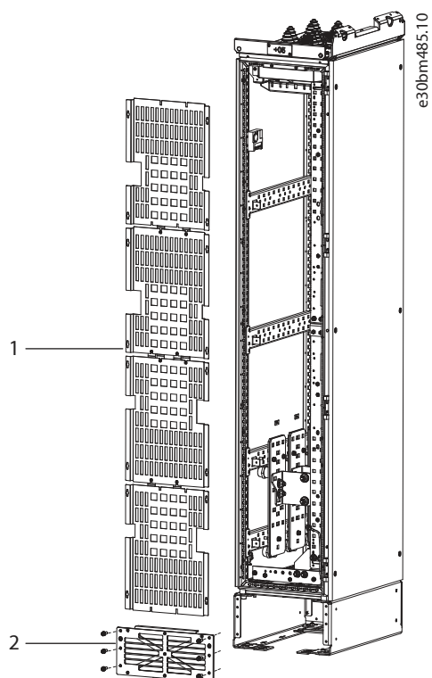
Figure 18: Removing the Front Grill and the Touch Protection
