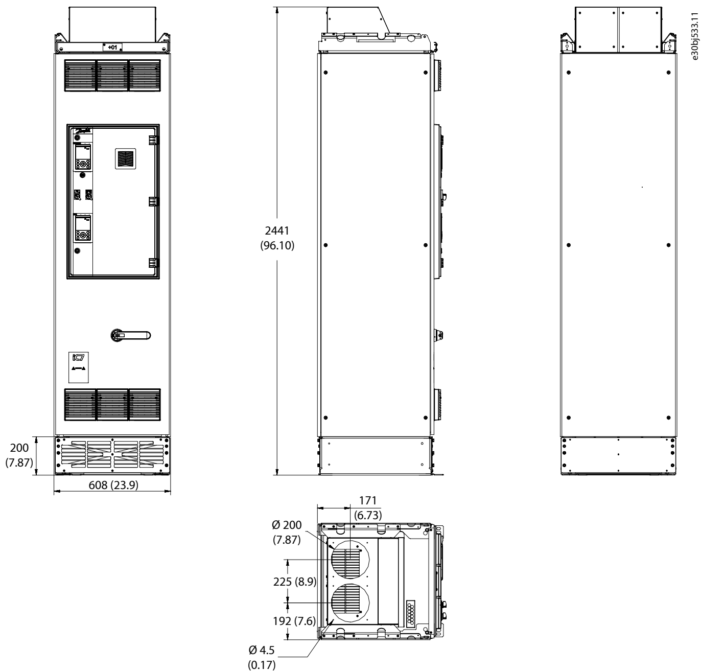
Figure 103: Dimensions for the Cooling Air Output Flange (+OAF), FE10, in mm (in)
