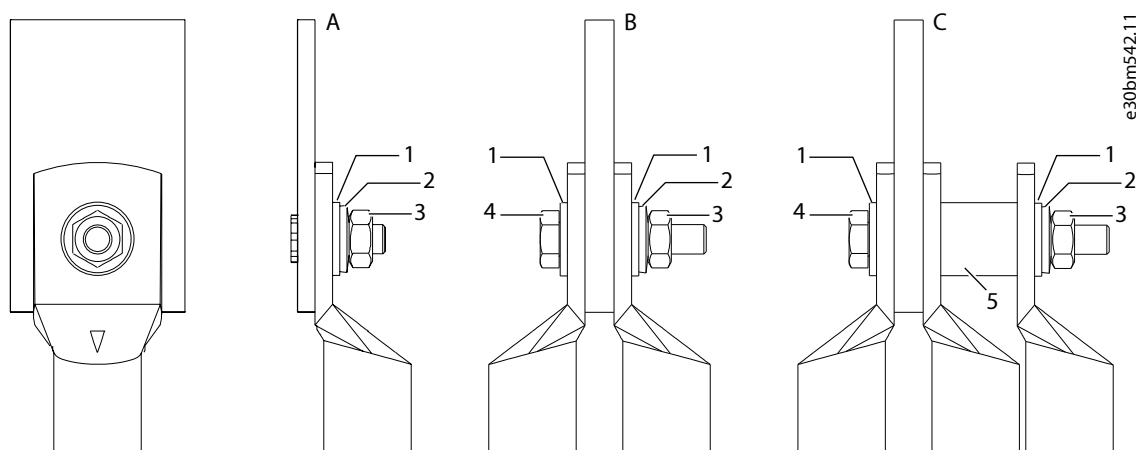
Figure 48: Connecting the Power Cables to the Terminals
