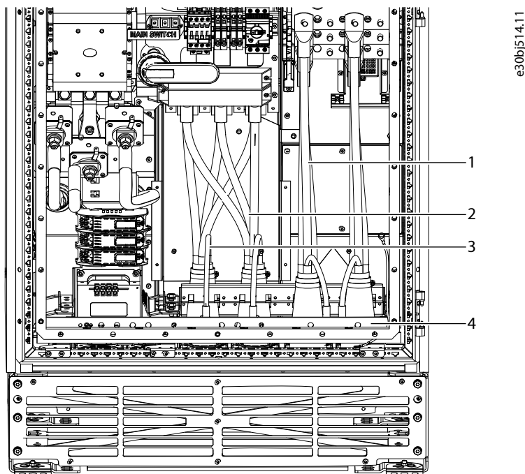
Figure 42: Cabling of the Enclosed Drive
