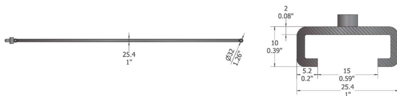
Figure: Mounting
