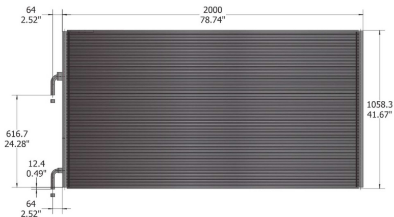
Figure: Dimensions
