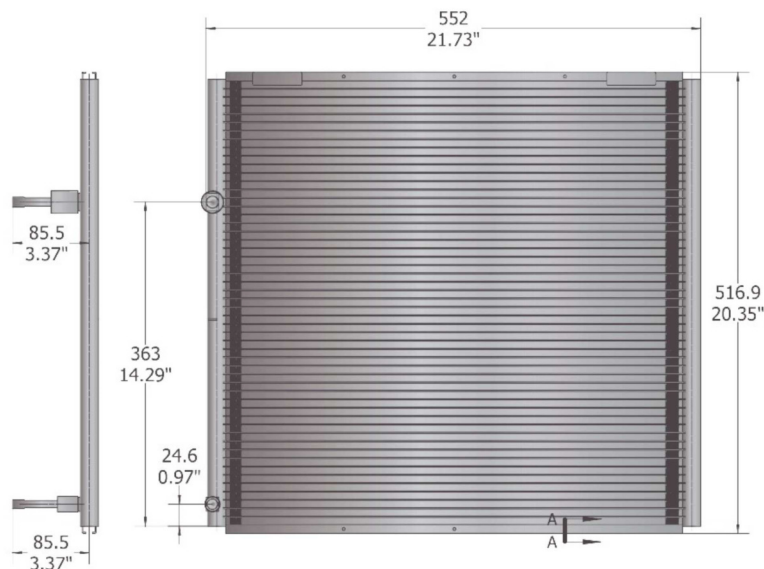
Figure: Dimensions
