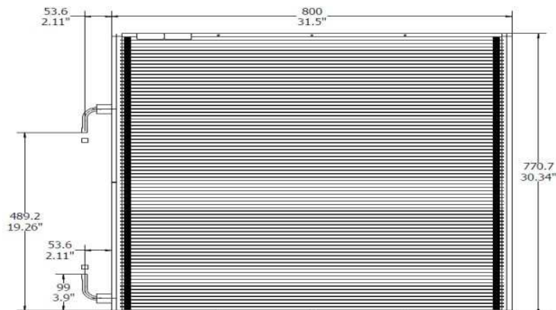
Figure: Dimensions
