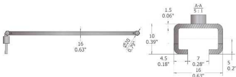
Figure: Mounting
