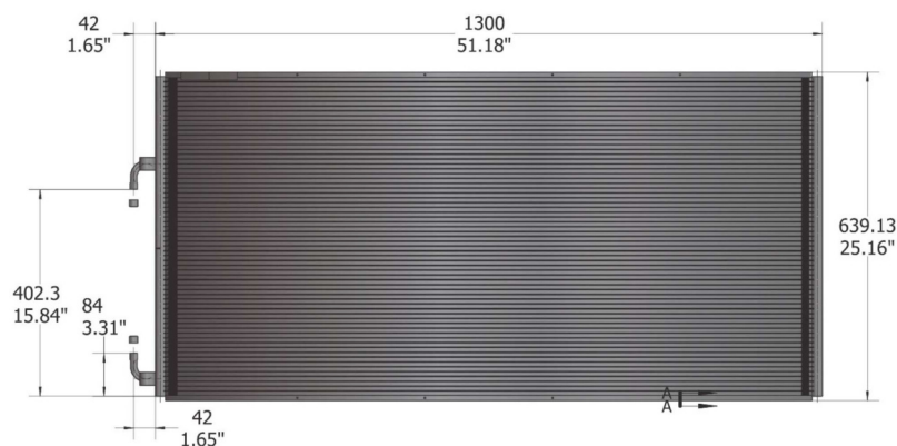
Figure: Dimensions
