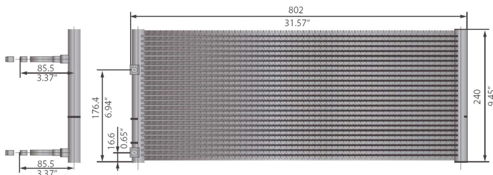
Figure: Dimensions
