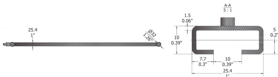
Figure: Mounting
