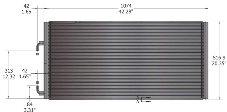
Figure: Dimensions
