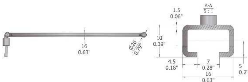
Figure: Mounting
