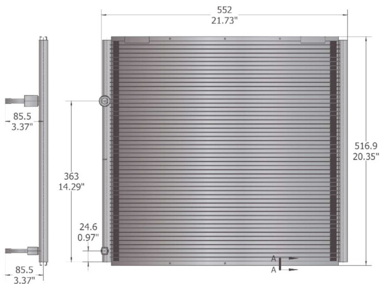
Figure: Dimensions
