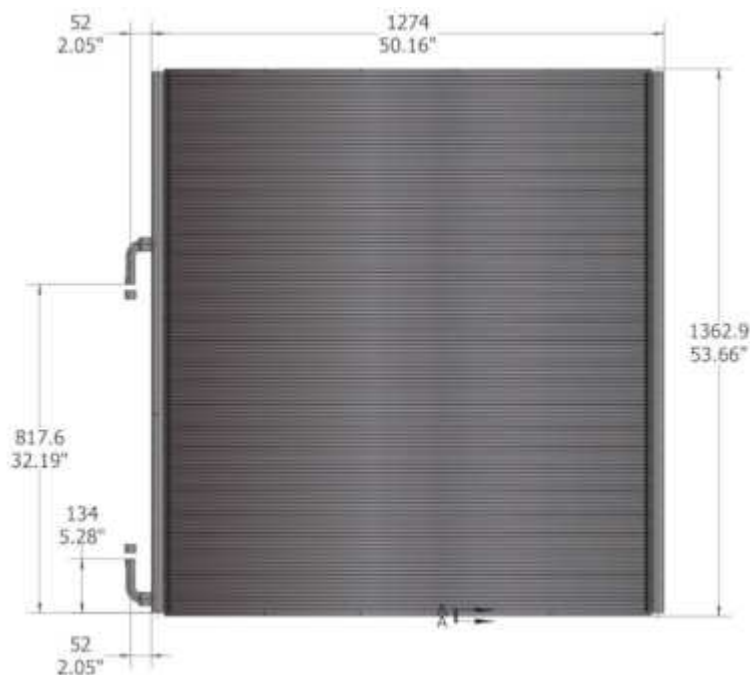
Figure: Dimensions
