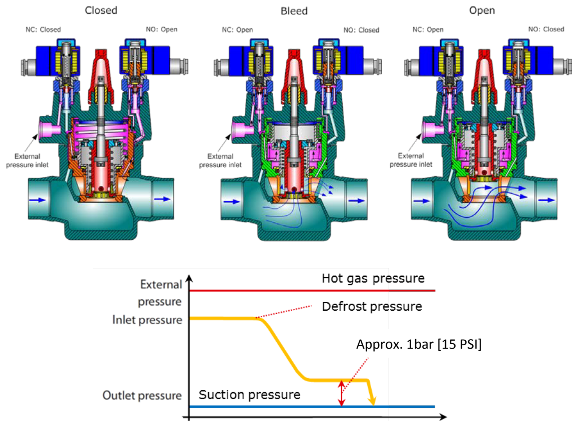
Figure 17: Example of 2-step solenoid valve ("Soft opening solenoid valve")
