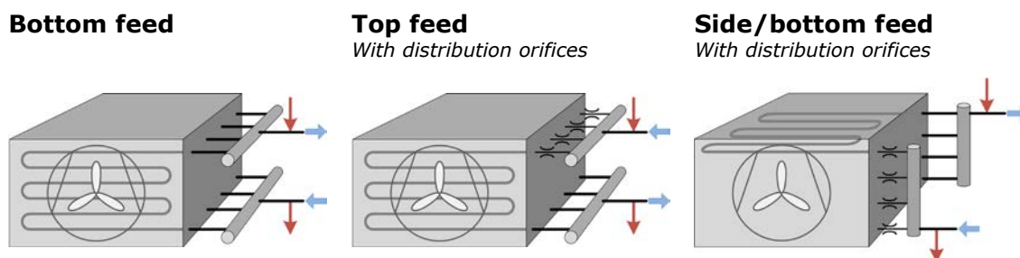
Figure 5: Tested evaporator types
