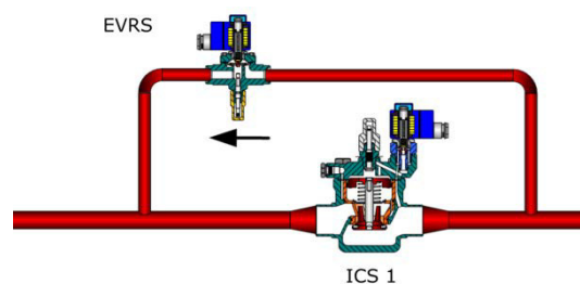
Figure 16: Example of "Soft opening solenoid solution"
