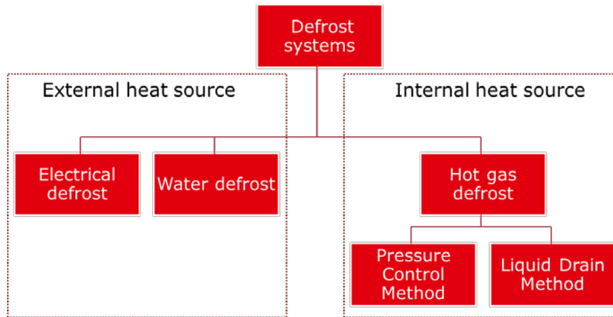
Figure 1: Common defrost systems
