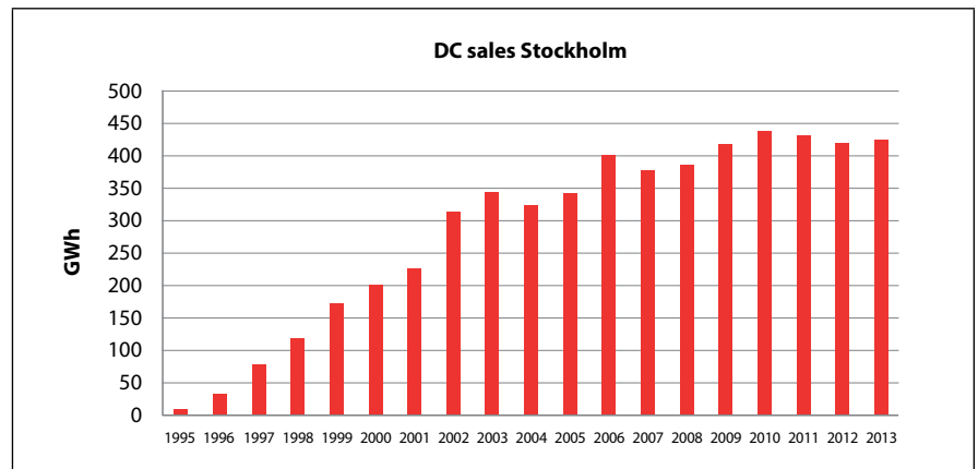
FIGURE 4: District cooling growth in Stockholm, Sweden [3]
