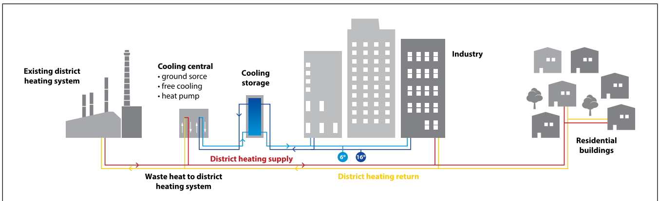
FIGURE 2: Supply concept for combined district cooling and heating
