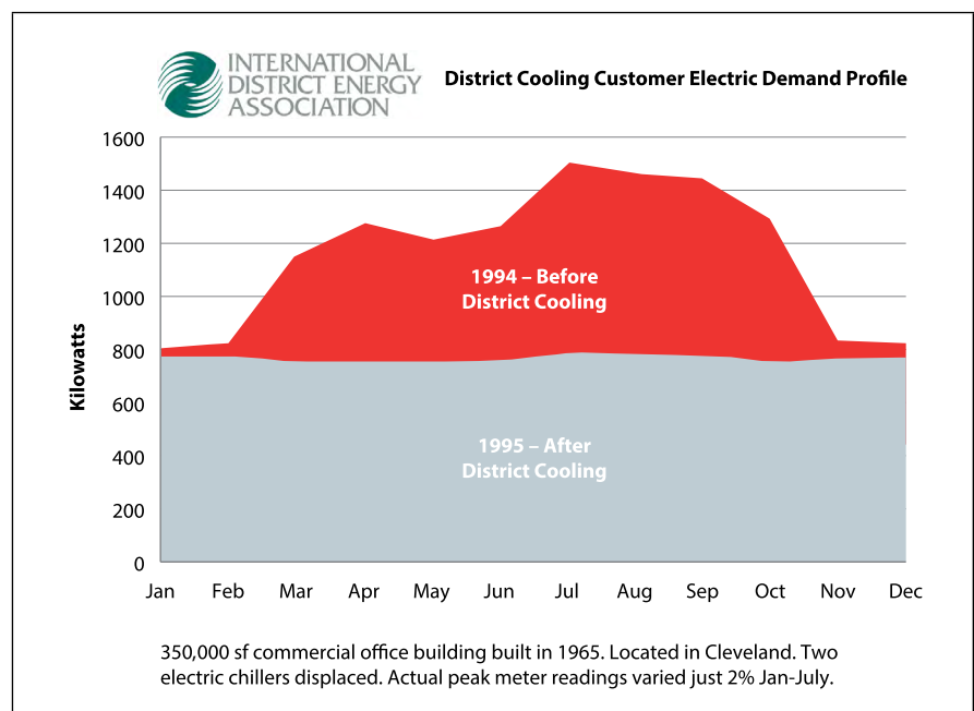
FIGURE 1: Example of how district cooling could change the electrical demand profile across the year [5]
