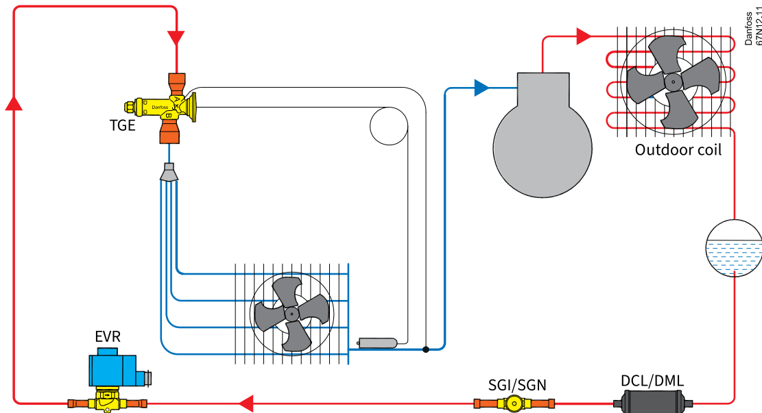
Figure: A diagram of a traditional refrigeration plant where TGE is used for flow in one direction only
