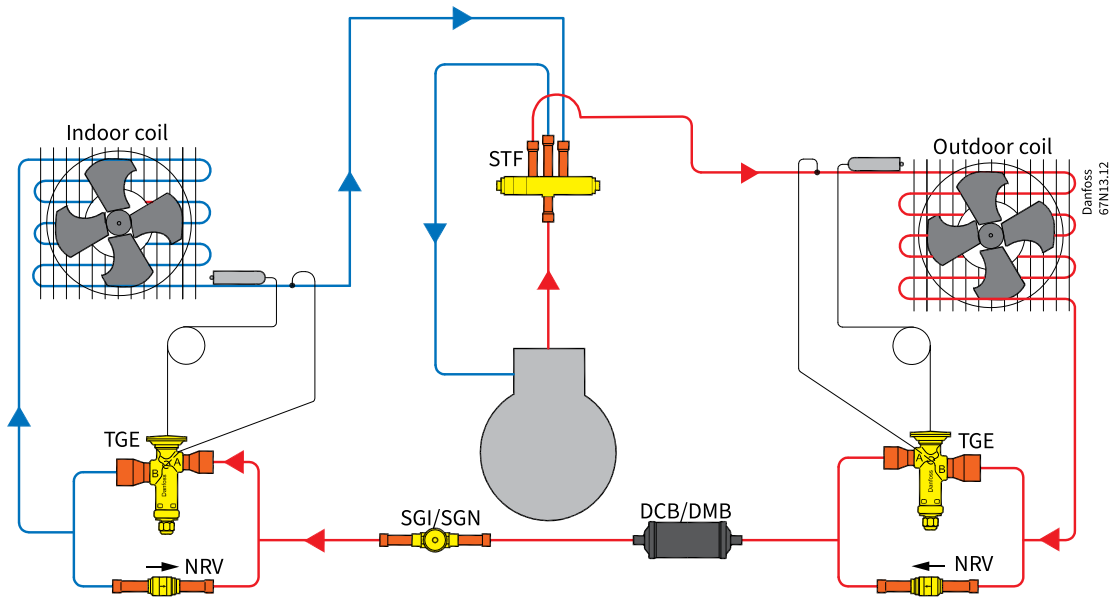
Figure: A conventional split heat pump system shown in cooling mode. This system has two TGE thermostatic expansion valves with fixed direction flow. An NRV check valve is placed in series with each TGE to allow liquid refrigerant to bypass when flow is opposite the TXV fixed direction
