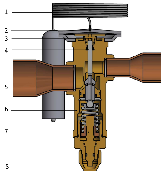
Figure: Double balanced port design TGE 20 and TGE 40
