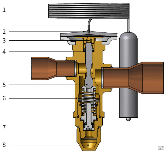
Figure: Balanced port design TGE 10
