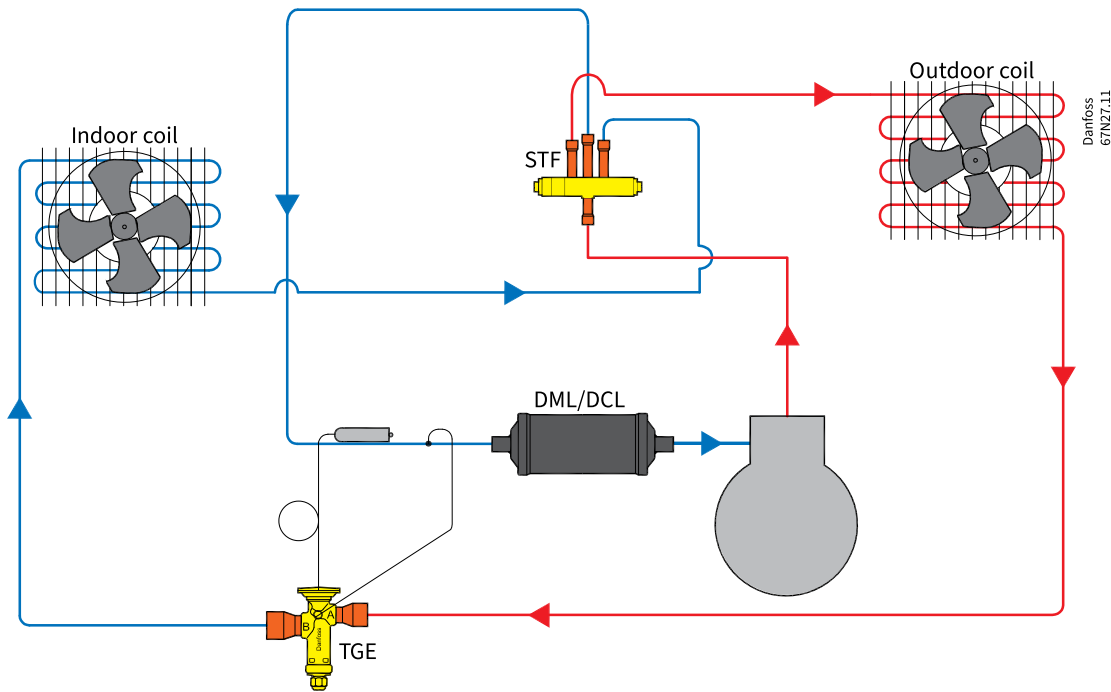
Figure: A heat pump system similar to that in above figure but with a more compact design, where the distance between evaporator and condenser is very short. This system has only one bi-flow TGE valve metering liquid refrigerant effectively in both directions. Changeover is by means of a 4-way valve. A suction filter drier is often placed in suction lines just before the compressor. The normal flow direction of TGE is determined by the primary function, i.e. cooling or heating
