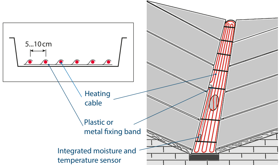
Gutter valley heating cable installation
