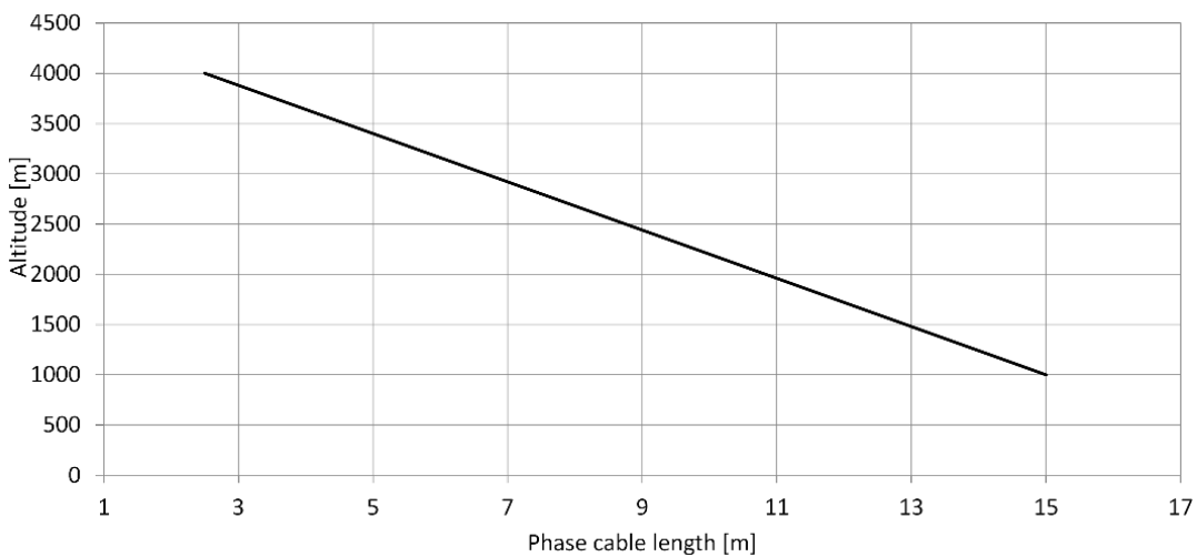
Picture 3 Allowed altitudes vs phase cable length
