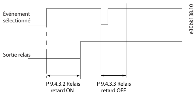
Illustration 87: Relais, retard OFF
