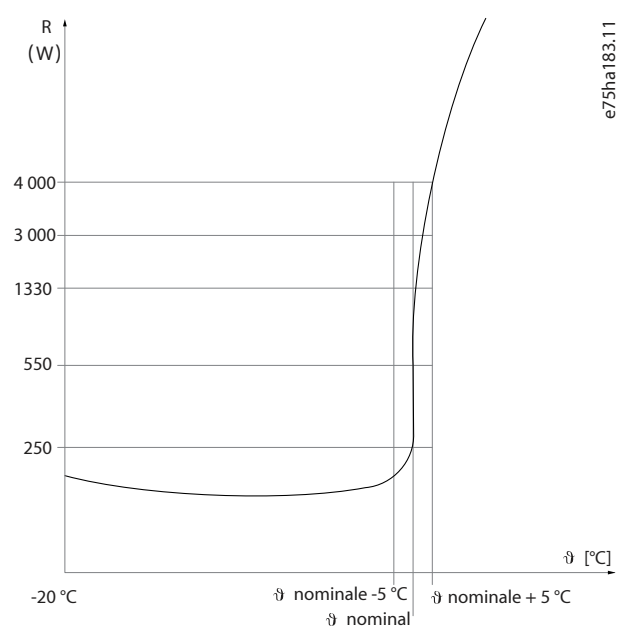
Illustration 74: Profil PTC
