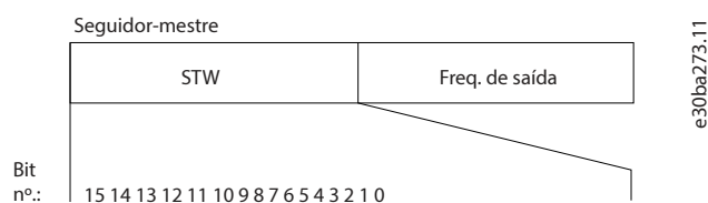
Figura 66: Status Word
