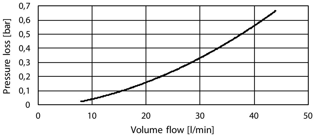
Picture 1 Pressure loss vs coolant flow
