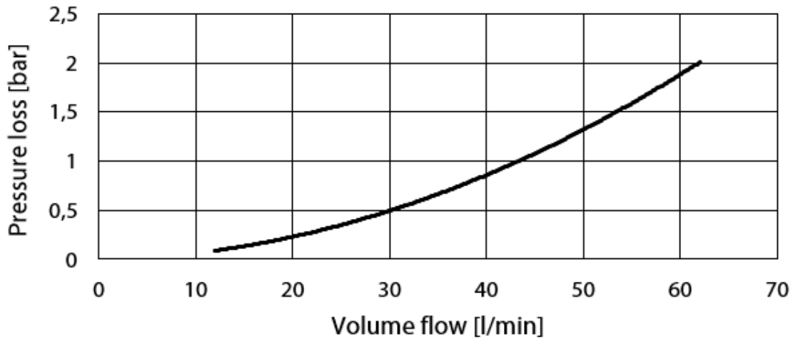
Picture 1 Pressure loss vs coolant flow
