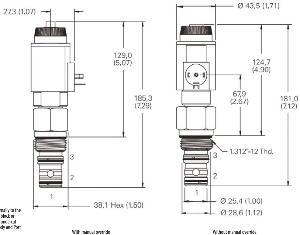
With manual override
