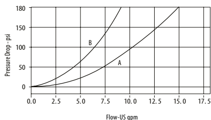
Flow vs Pressure drop Regulated flow P1 to P3 (P2 to Atm) Full current (1700 mA on a 12V Coil)
