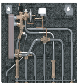
EvoFlat FSS, with circulation
