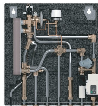
EvoFlat MSS, with circulation
