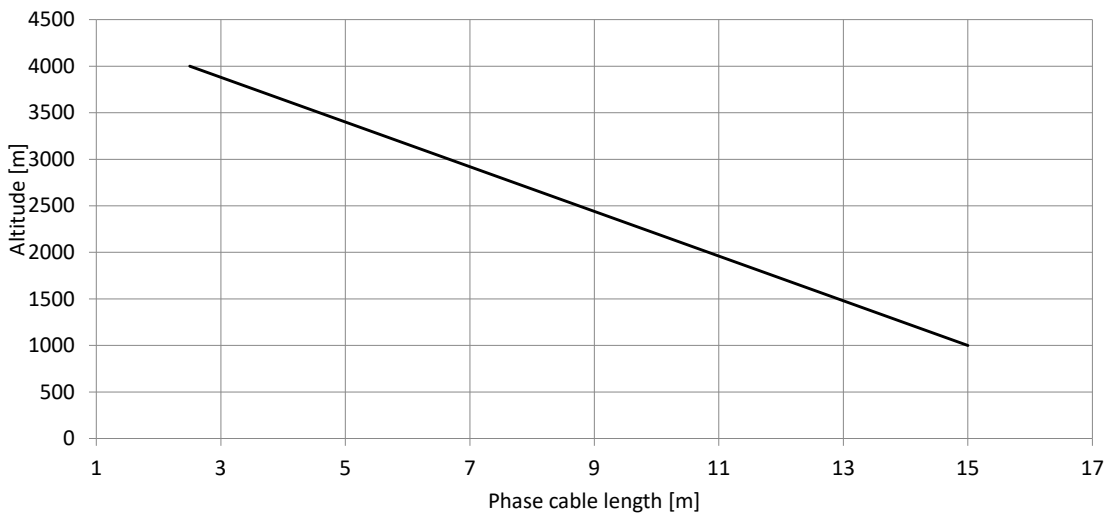
Picture 3 Allowed altitudes vs phase cable length
