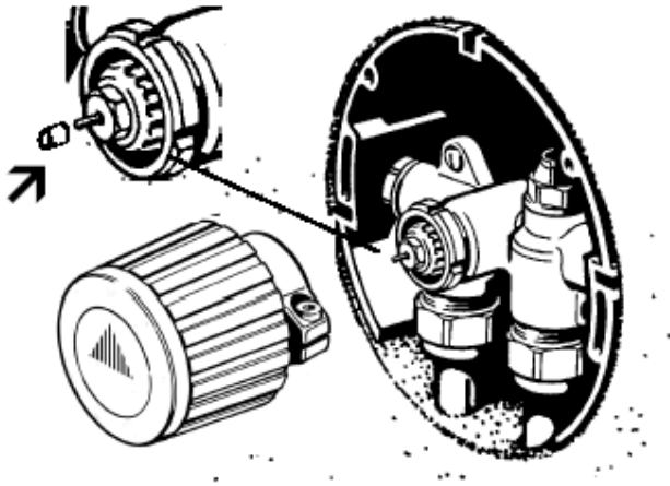
Fig. 2: Instruction in mounting the spindle extension
