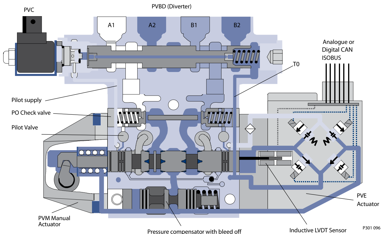
PVBD, PVBZ with optional diverter feature
