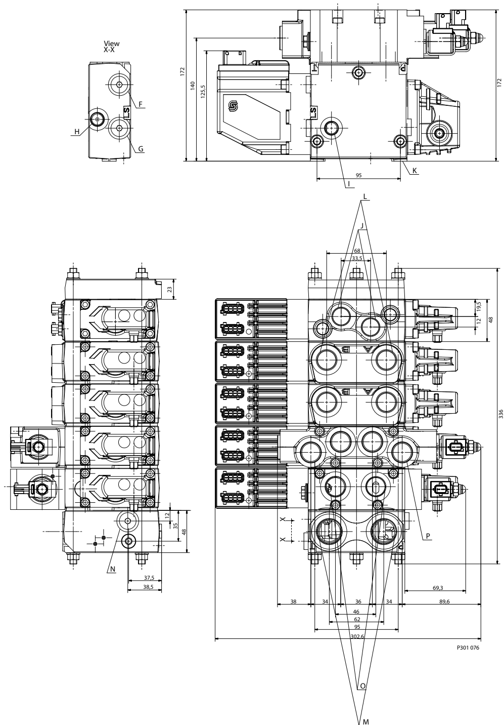
Drawing for 5-section valve group
