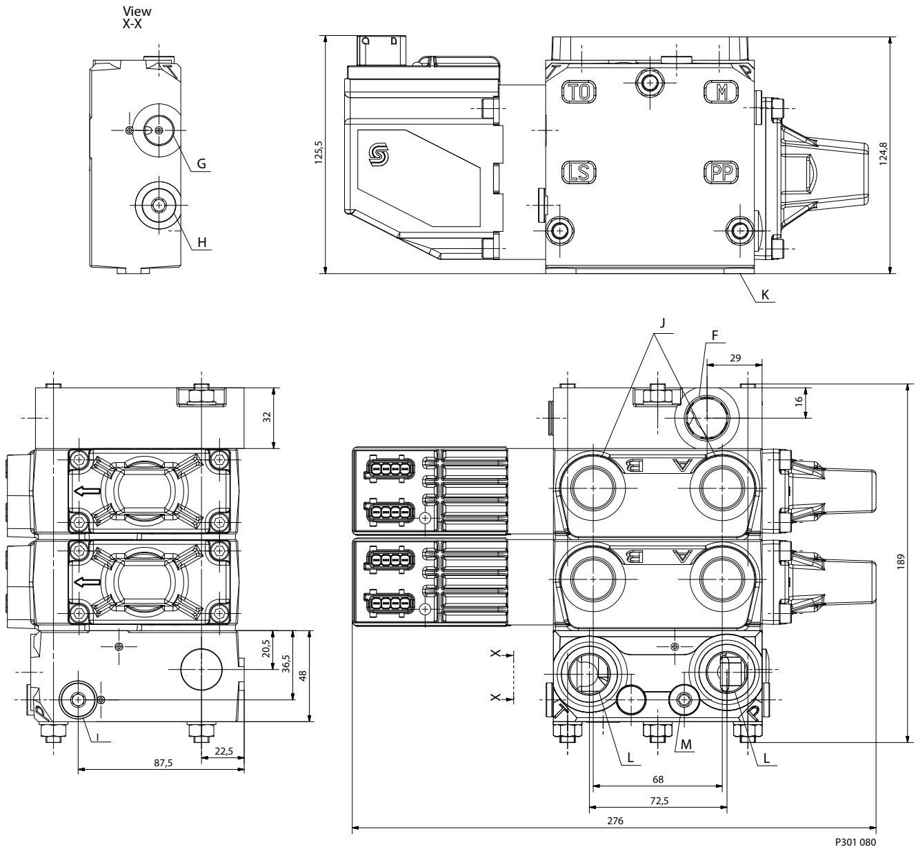
Drawing for 2-section valve group
