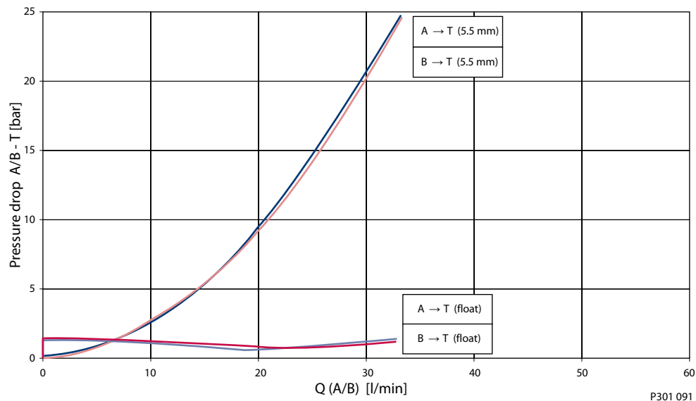
Pressure drop A/B to T : PVBS 157B9410
