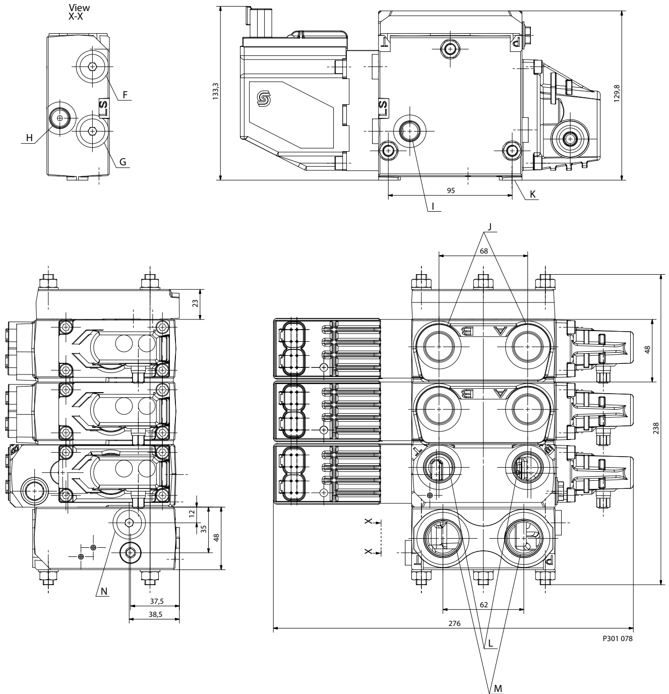
Drawing for 3-section valve group
