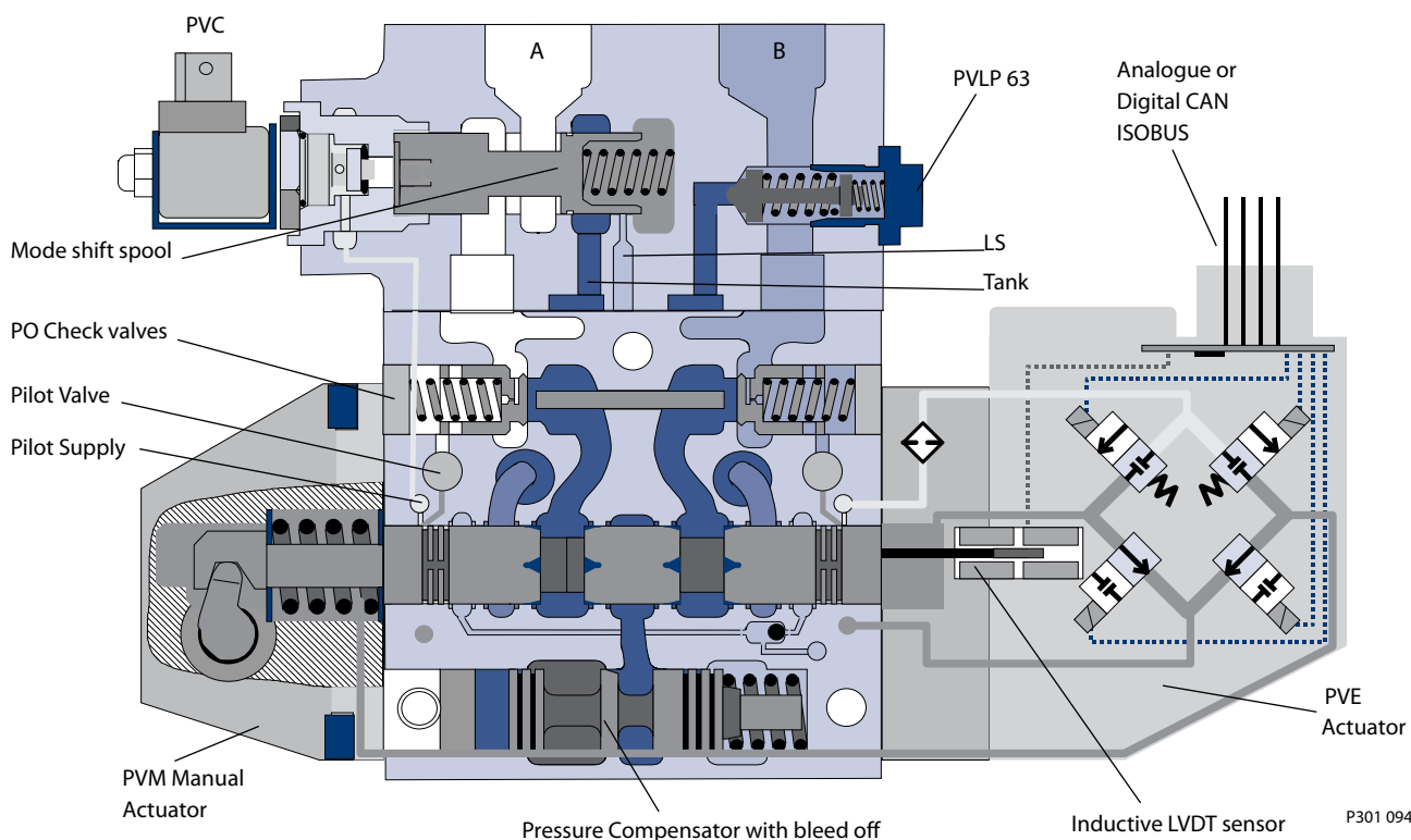
Hitch double-acting valve module
