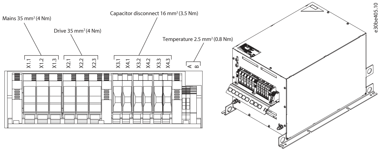
Figure 46: IP20 X4-V3 External Fan, Terminal Designation and 3D View
