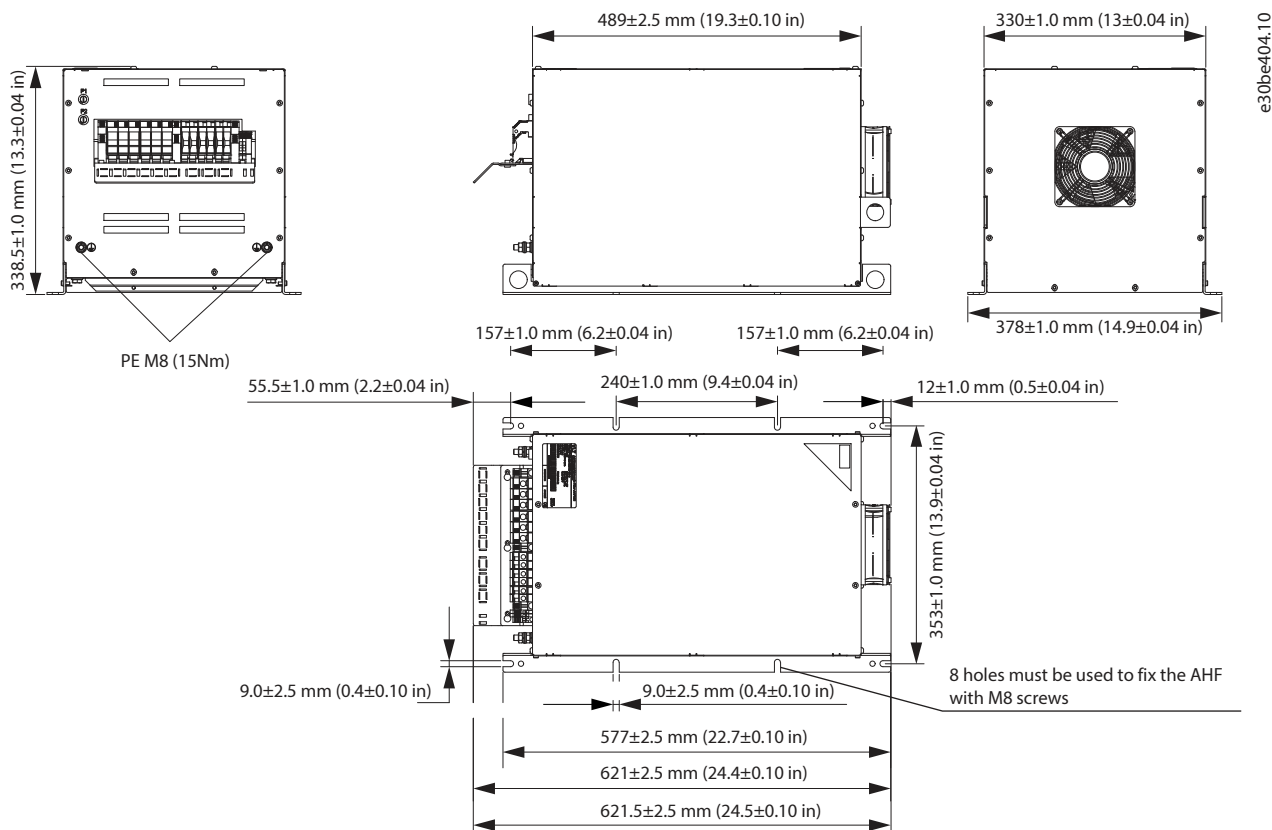
Figure 45: IP20 X4-V3 External Fan
