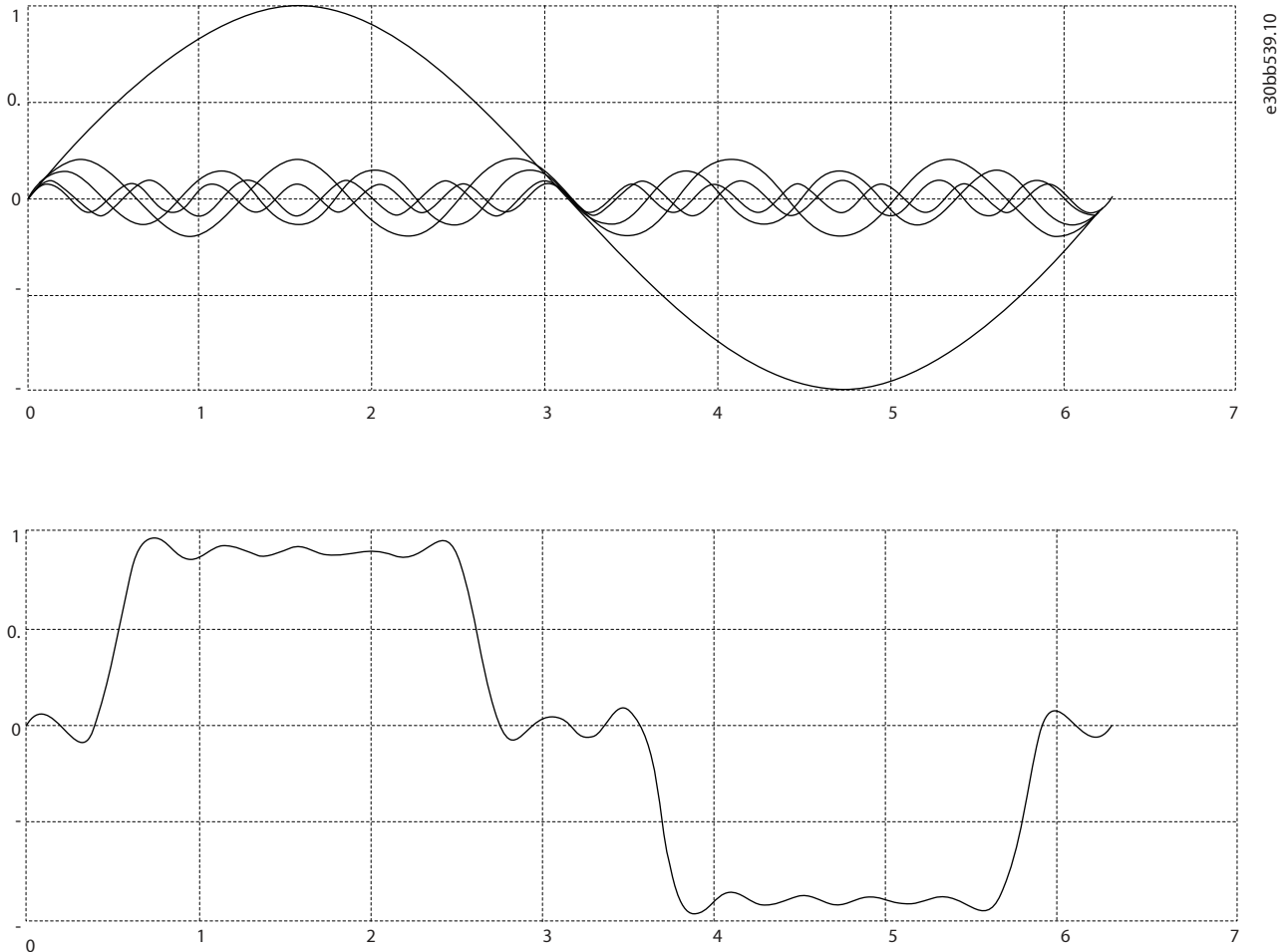
Figure 5: Sinusoidal Waveforms
