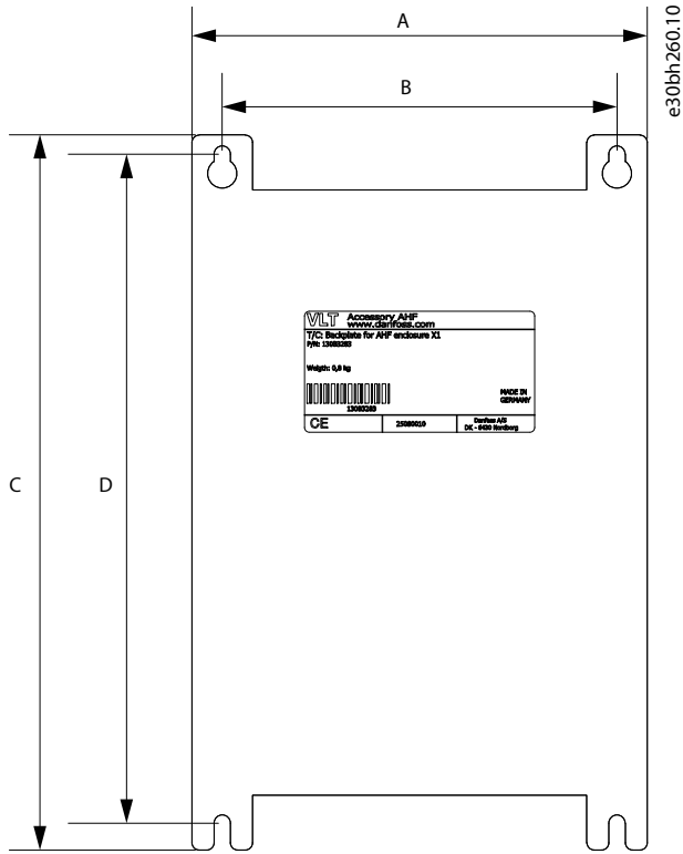
Figure 79: Backplate Dimensions for X1 and X2 Enclosures
