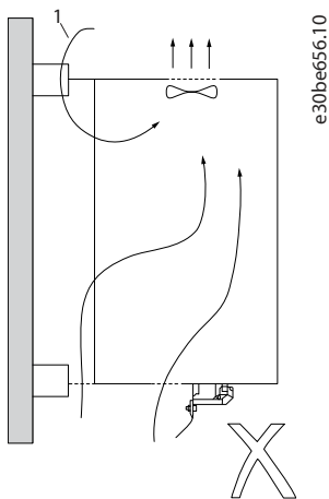
Figure 20: False Airflow
