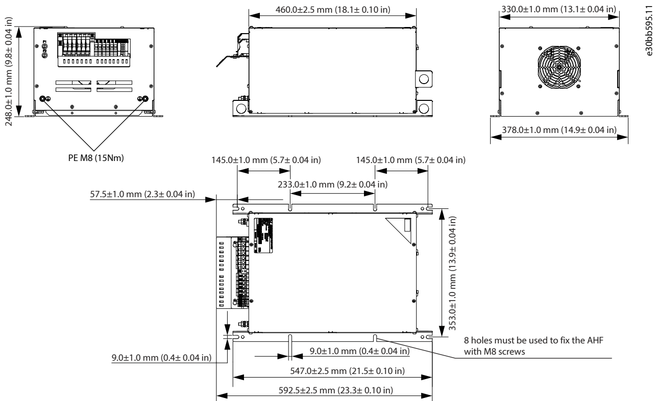
Figure 39: IP20 X3-V3 Internal Fan
