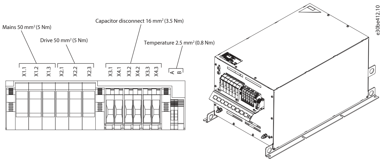
Figure 50: IP20 X5-V3 External Fan, Terminal Designation and 3D View
