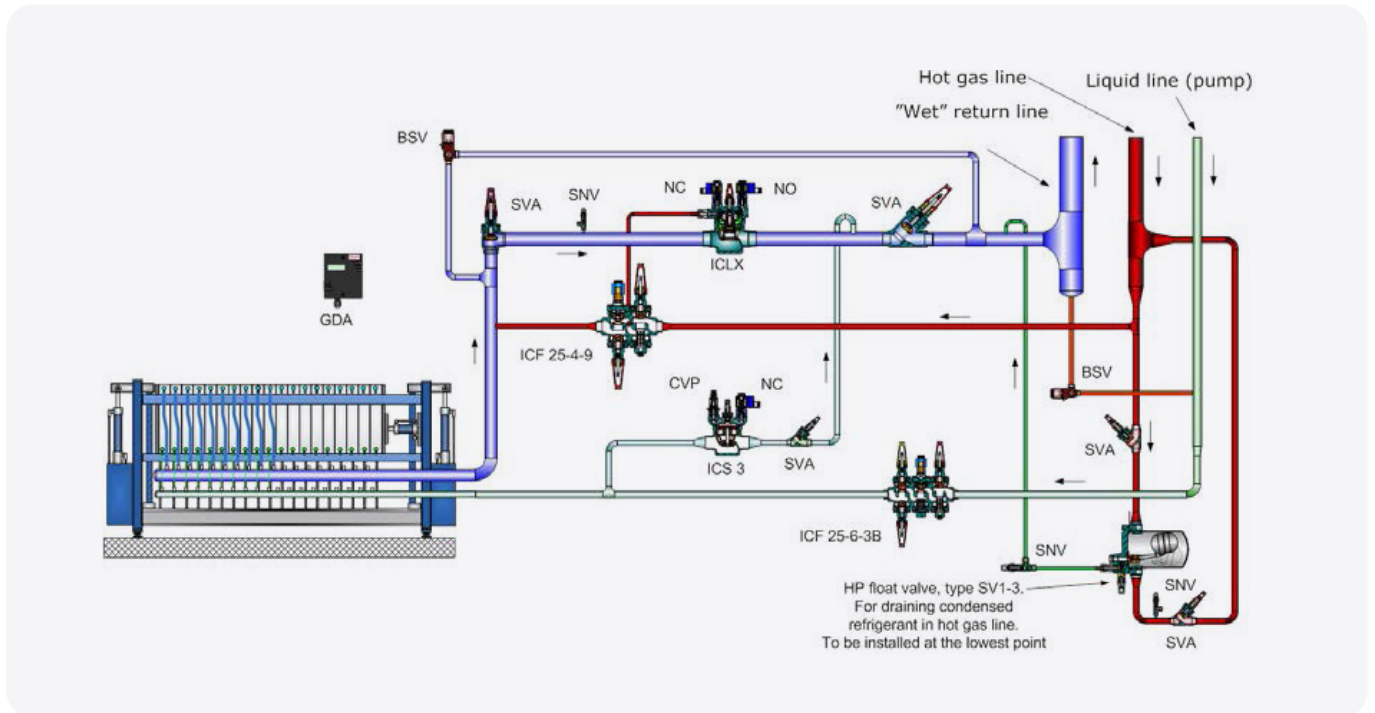
↓ Figure 19: Example of draining condensate from hot gas lines
