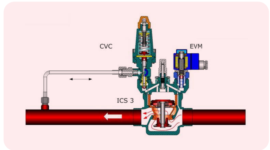
Figure 16: Example of "Regulated hot gas pressure" (back pressure regulator) →
