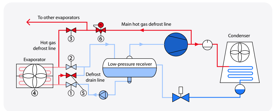
Figure 15: Hot gas defrost principle in an industrial overfeed system →
