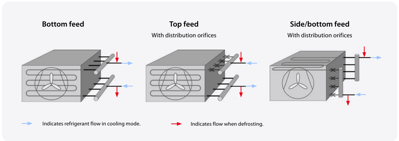
↓ Figure 5: Tested evaporator types
