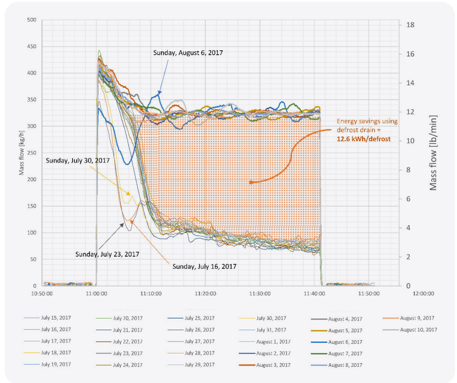
↑ Figure 13: Field test results from a European customer test site: Hot gas mass flow from old Pressure control system vs. the new Danfoss ICFD Defrost Module based on the Liquid drain method.
