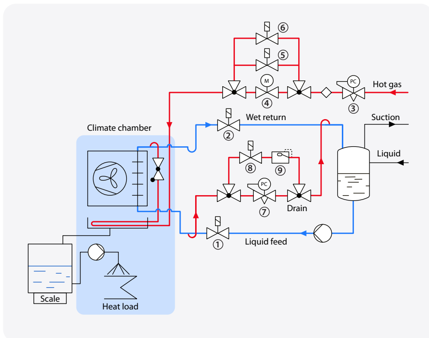
← Figure 4: Principle PI diagram showing of test system
