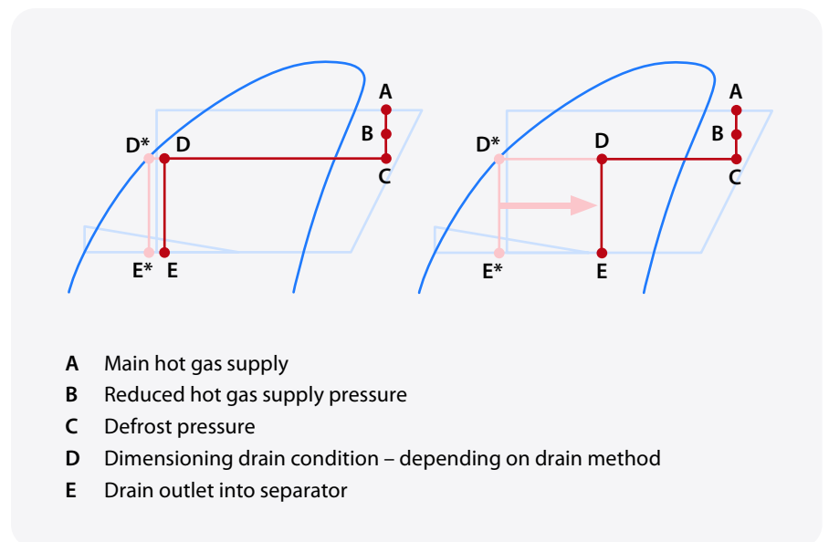
Figure 14: → Defrost principle in log(p)-h diagram
