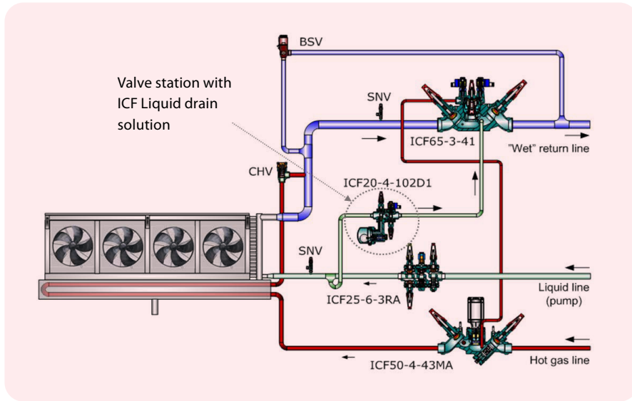
↑ Figure 11: Liquid riser in systems with Liquid drain systems
