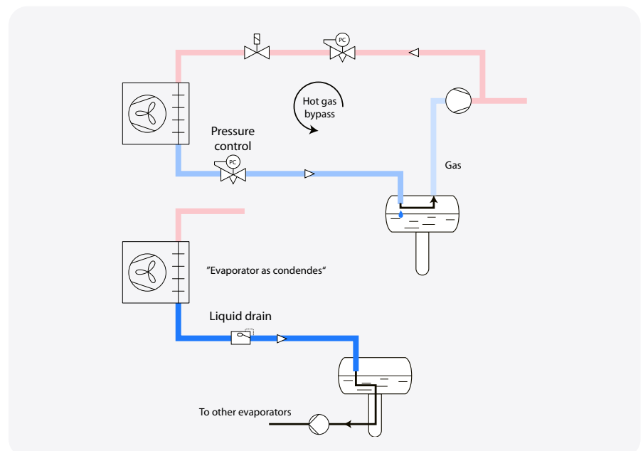
Figure 2: → Pressure control and liquid drain
