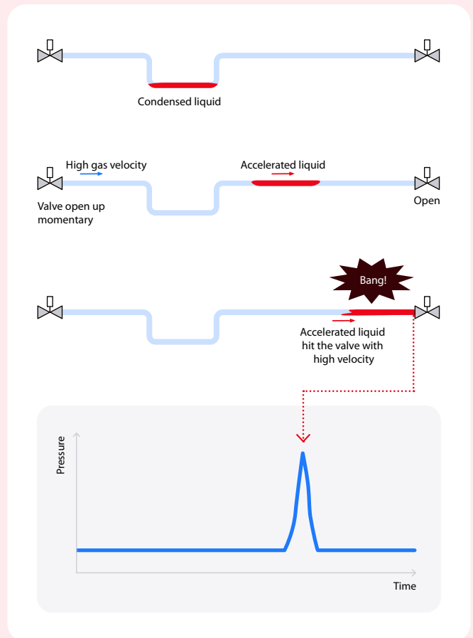
↑ Figure 20: Example on pressure impact caused by Vapour-propelled liquid slug
