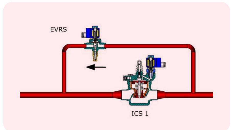
Figure 17: Example of "Soft opening solenoid solution" →
