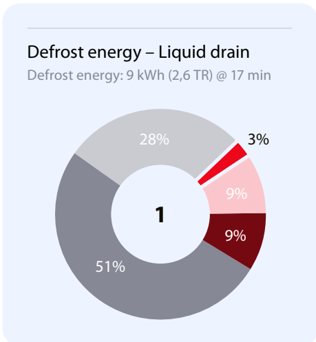
↑ Figure 7: Defrost energy – Pressure control vs. Liquid drain method
