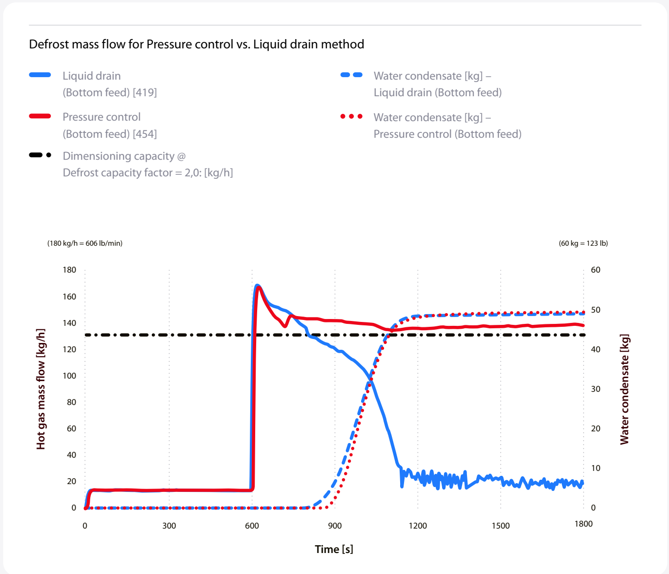
↑ Figure 6: Defrost mass flow for Pressure control vs. Liquid drain method measured in laboratory
