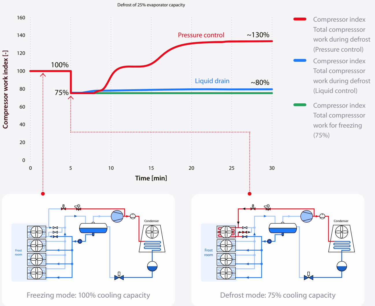
↑ Figure 8: Compressor work during defrost – Pressure control vs. Liquid drain method
