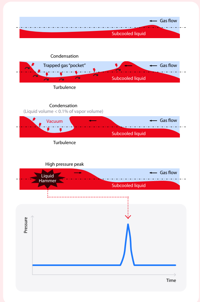
↑ Figure 21: Example on pressure impact caused by Condensation-induced shock
