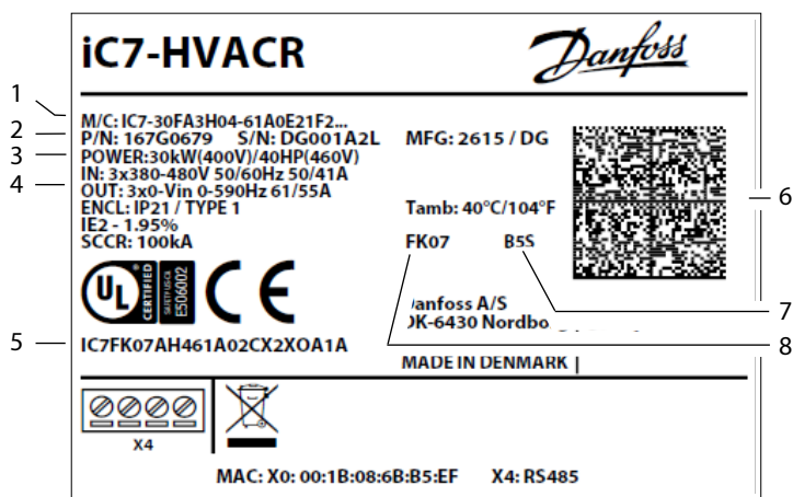
Figure 1: Example of an FB07/FK07 Product Label
