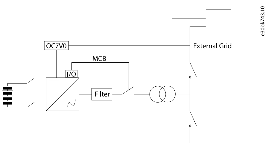
Figure 14: External Grid Synchronization
