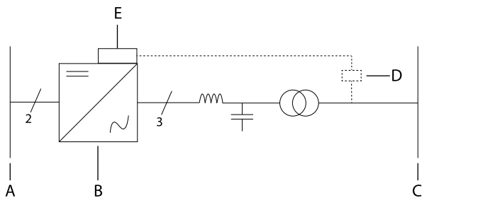
Figure 11: Grid Converter with LC Filter and Transformer
