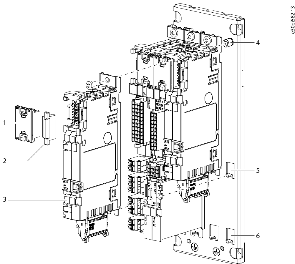
Figure 4: Installing a Board to the Modular Control Unit Mounting Plate
