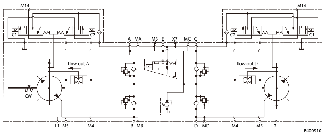
Control-Cut-Off Valve
