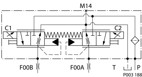
NFPE schematic
