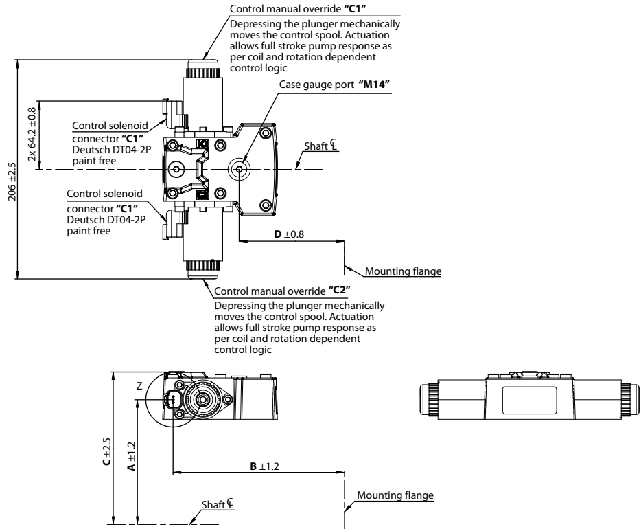
Control solenoid connector "C1" & "C2"
