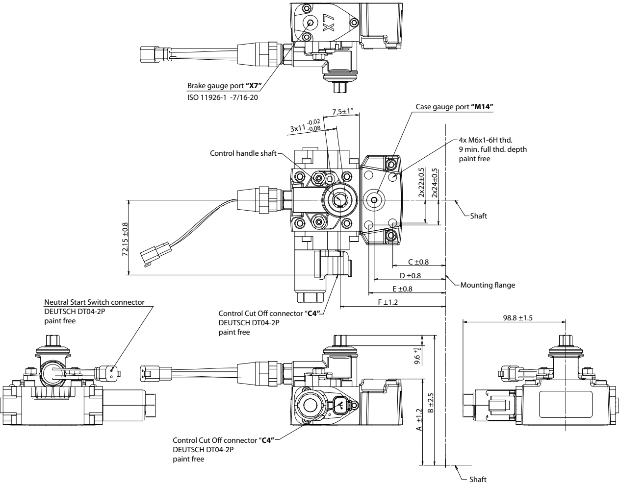
Neutral start switch, control cut off connectors
