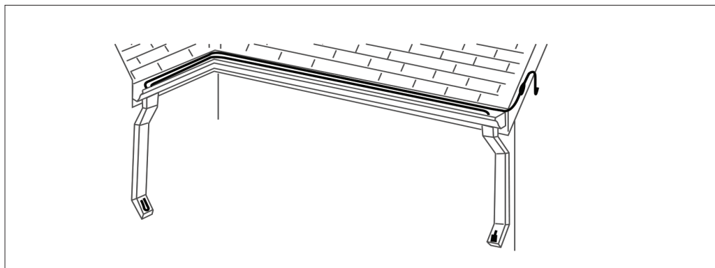
Figure 7. Double Cable Run in gutter and downspouts
