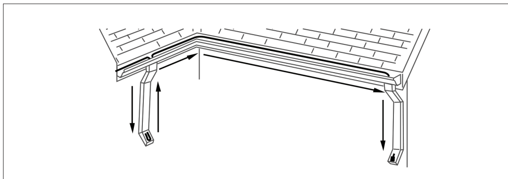
Figure 6. Cable routed back along the roof line in the gutter and downspouts
