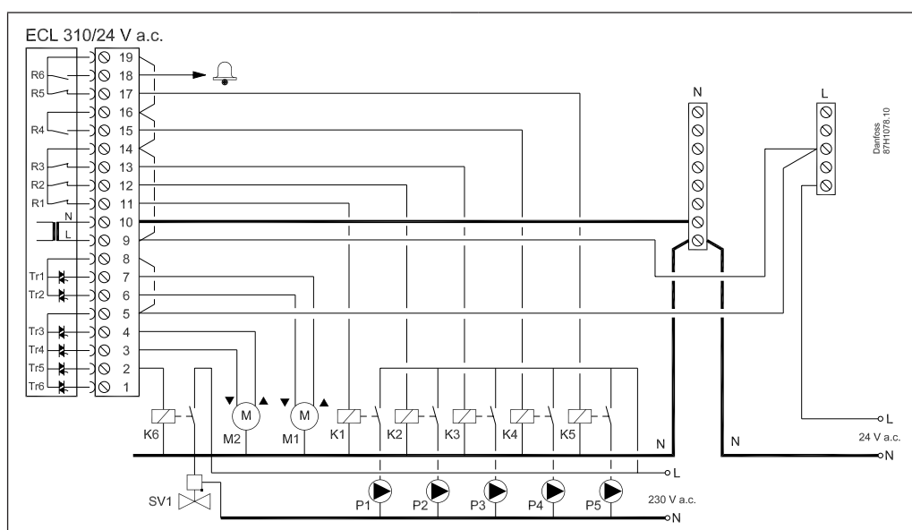
ECL Comfort 310 wiring example: Application A368.1
