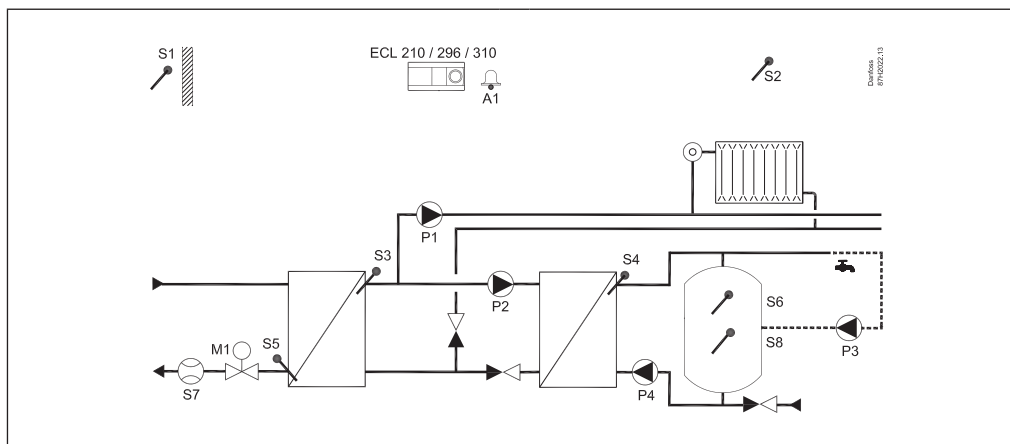
A247.1, ex. a: Indirectly connected heating and DHW tank charging system. Parallel mode or DHW priority
