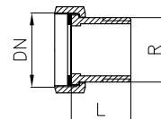
External thread tailpieces
