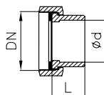
Weld-on tailpieces
