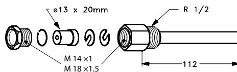
Immersion pocket
