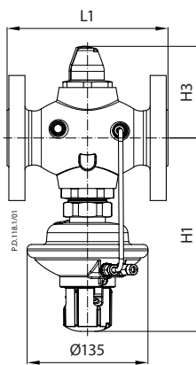
AVPQ DN 32-50 \Delta p = 0.2-1.0 bar
