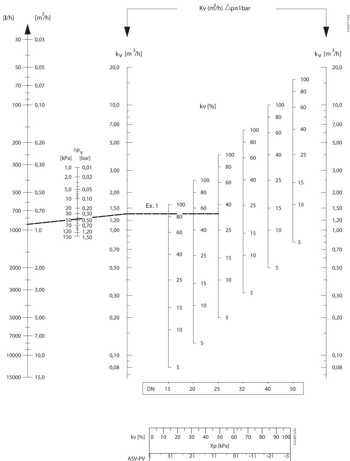
Fig. A – Diagrama de dimensionare ASV-PV DN 15 – 50
